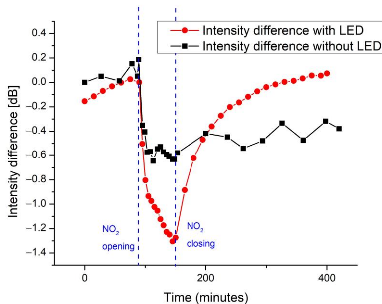
Figure 10. Variation of intensity after opening and closing the NO 2 flux with and without LED irradiation. The opening time is 1 h.
