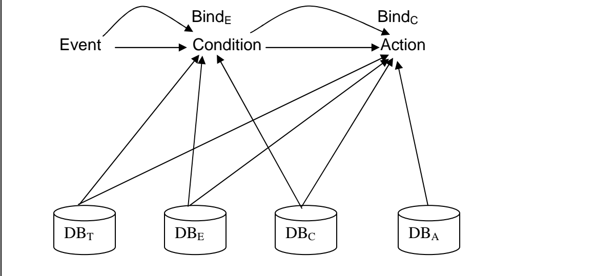
Figure 2: The context within which a rule is processed
