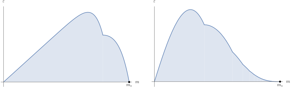
Figure 1. Numerical plots of the curve \varepsilon(m) dividing the stability/instability regions for the unit ball B_1 as in Theorem 1.1; the ball is unstable in the shaded region. Left: the case \beta > \beta_* ( d = 3 , \alpha = 1 , \beta = 30 ). Right: the case \beta < \beta_* ( d = 3 , \alpha = 1 , \beta = 4 ). Here \beta_* = 22 .
