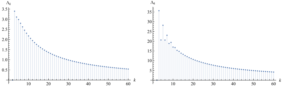
Figure 5. Numerical plots of the sequence \Lambda_k in (30), whose positivity implies the inequality m_{k,k+1} > m_{k+1}^c . Left: d = 10, \alpha = 8, \beta = 10 . Right: d = 10, \alpha = 8, \beta = 130 . Here \beta_* = 134 .
