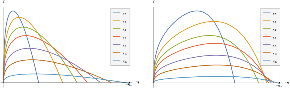
Figure 4. Numerical plots of some of the functions \varepsilon_k(m) in the case \beta < \beta_* . Left: d = 12, \alpha = 9, \beta = 4 . Right: d = 12, \alpha = 9, \beta = 40 . Here \beta_* = 86.5 . The picture on the right shows that some of the functions \varepsilon_k can be “skipped” in the computation of the final profile \varepsilon(m) .
