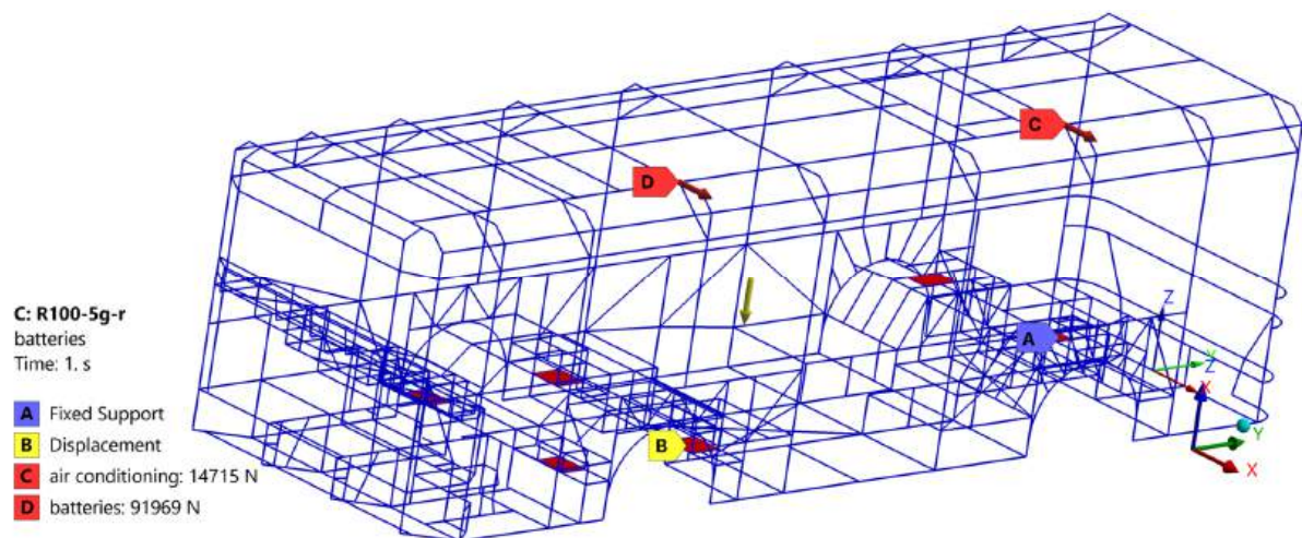
Figure 7. Boundary conditions for the UNECE R100 lateral 5 g loading case (R100-5g-r model).
