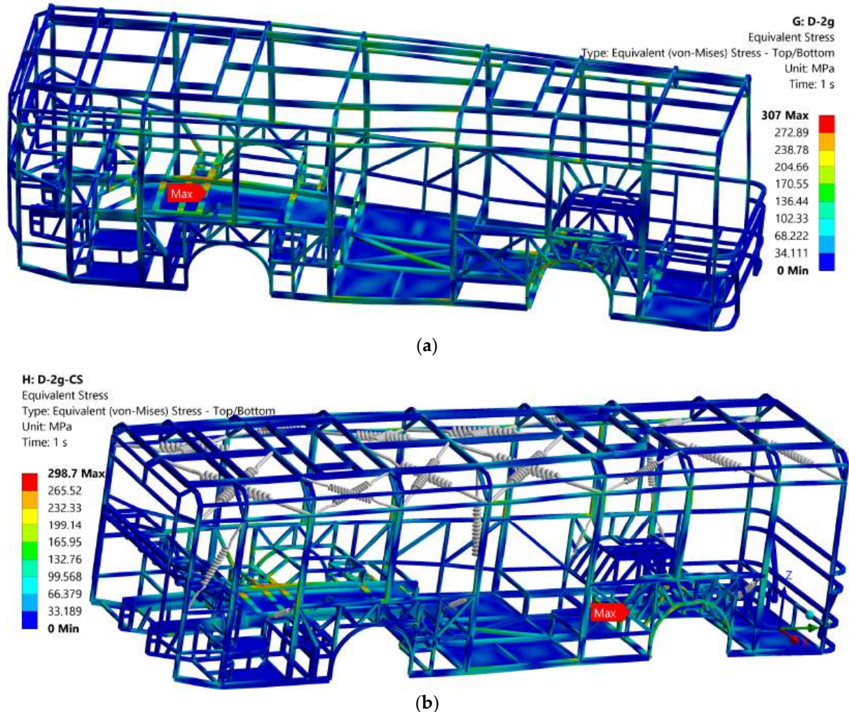
Figure 9. Equivalent stress (von Mises) maps under diagonal racking: (a) D-2g. (b) D-2g-CS.
