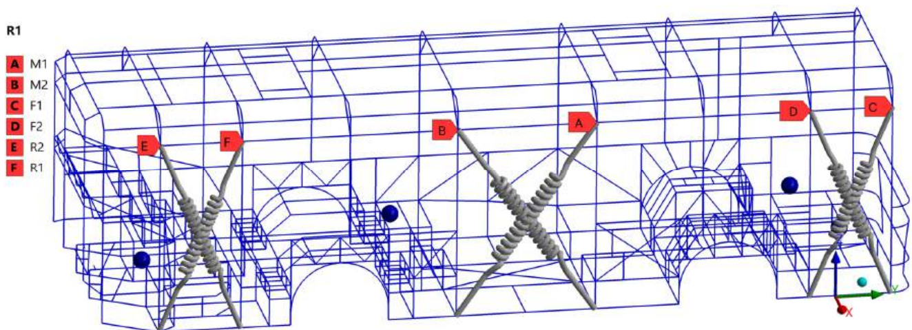
Figure 17. Numerical scheme for quantifying door-opening distortion using low-stiffness diagonal Spring Joints: F1–F2, front door; M1–M2, middle door; R1–R2, rear door.
