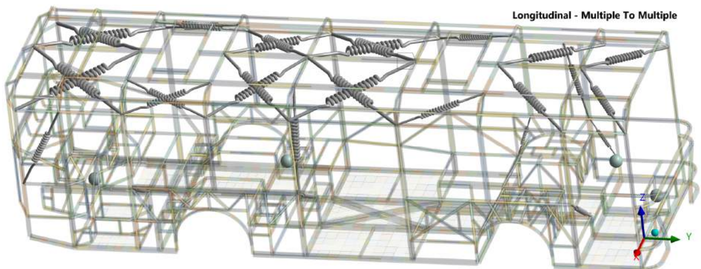
Figure 4. Implementation of the prestressed cable system in the D-2g-CS model.
