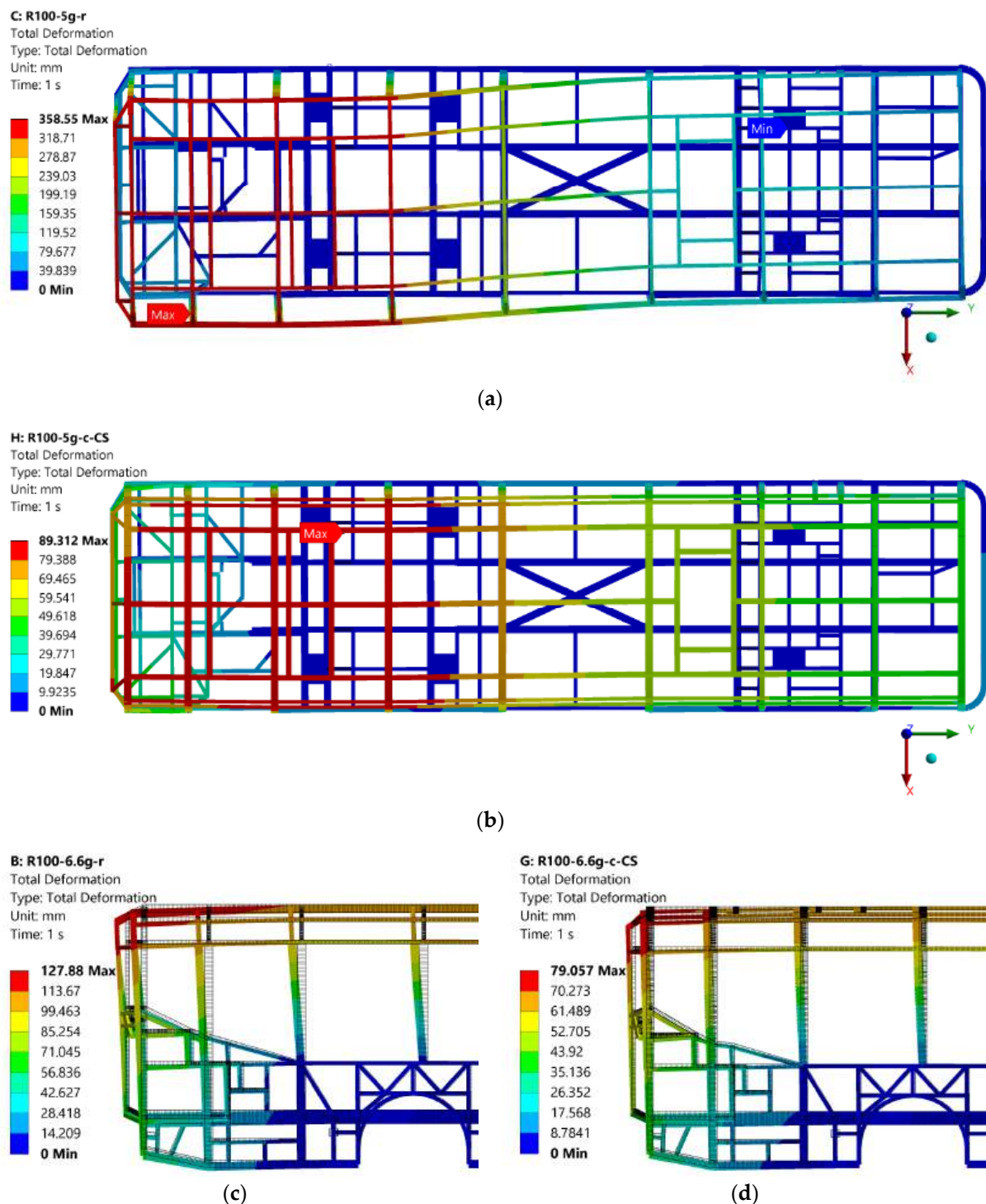
Figure 15. Deformation maps under R100 loading: (a) R100-5g-r. (b) R100-5g-c-CS. (c) R100-6.6g-r. (d) R100-6.6g-c-CS.
