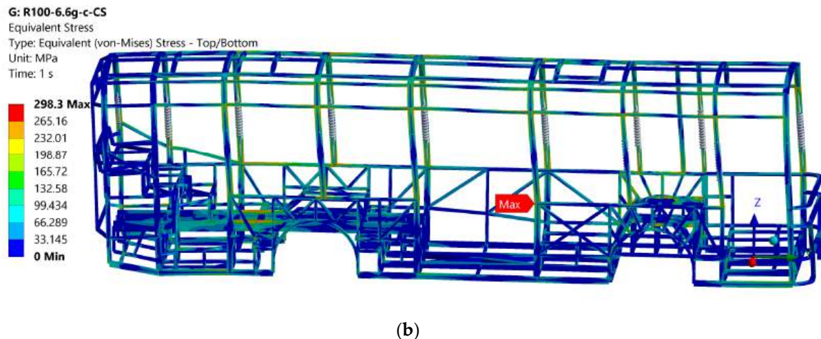
Figure 14. Equivalent stress (von Mises) maps under R100 longitudinal (6.6 g) loads: (a) R100-6.6g-r. (b) R100-6.6g-c-CS.
