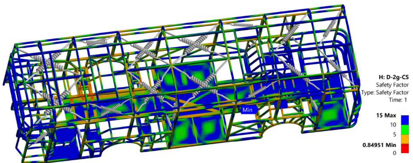
Figure 10. Safety factor map in D-2g-CS mode.
