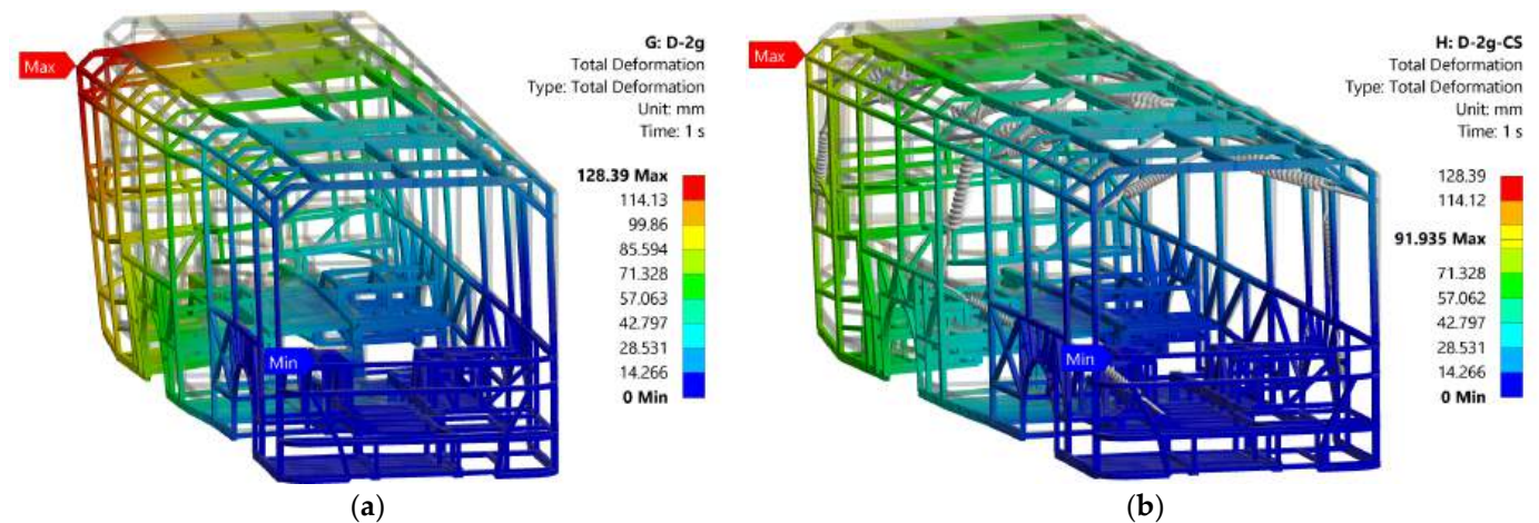
Figure 11. Deformation maps under diagonal racking: (a) D-2g. (b) D-2g-CS.
