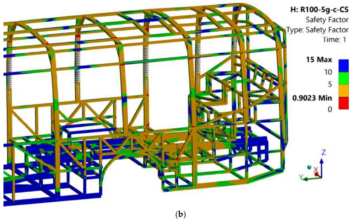
Figure 13. Safety factor maps under R100 transverse (5 g) loads: (a) R100-5g-r. (b) R100-5g-c-CS.
