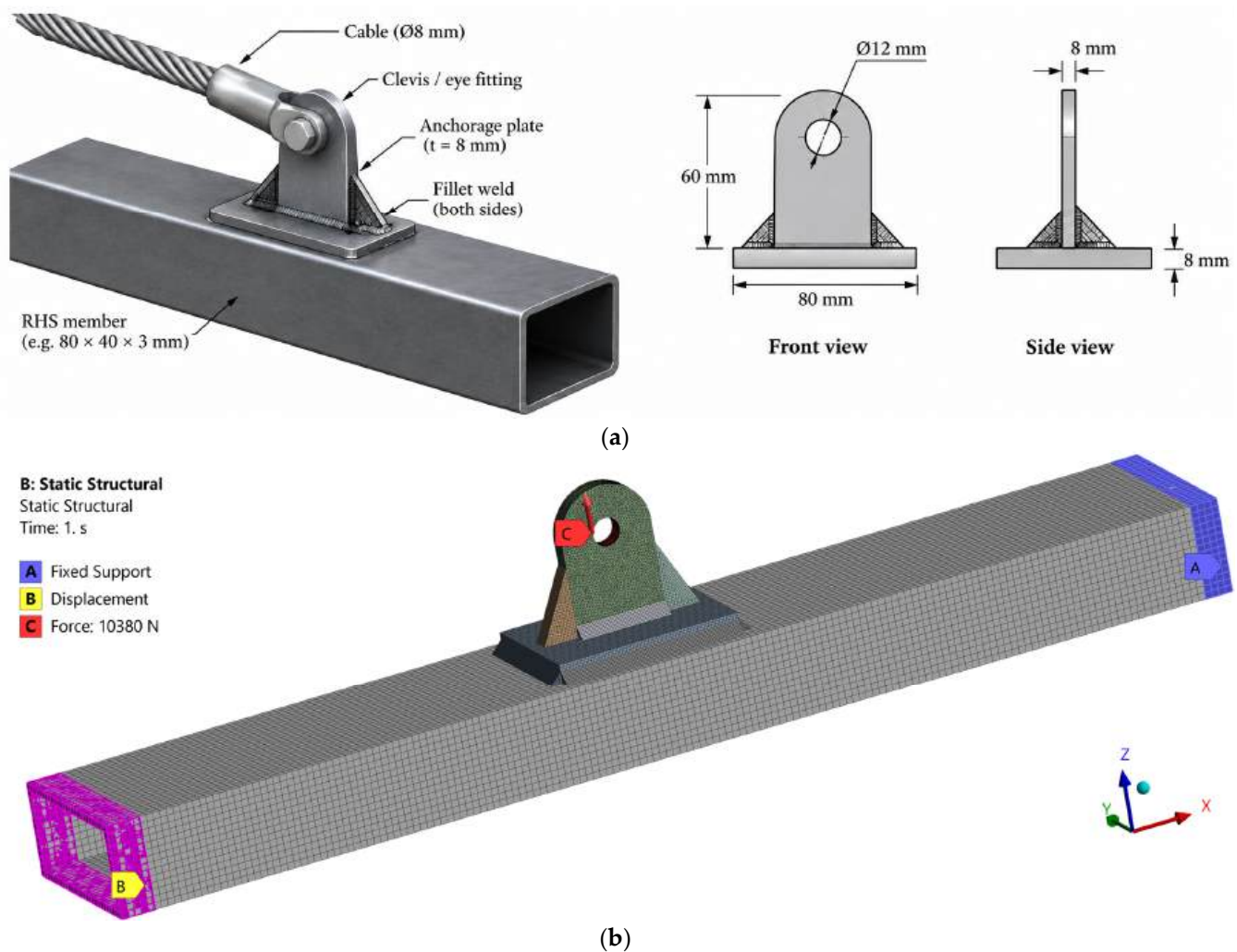
Figure 6. Representative CS anchorage used for the local component-level assessment: (a) anchorage geometry and principal dimensions; (b) finite-element mesh, boundary conditions, and applied cable force.
