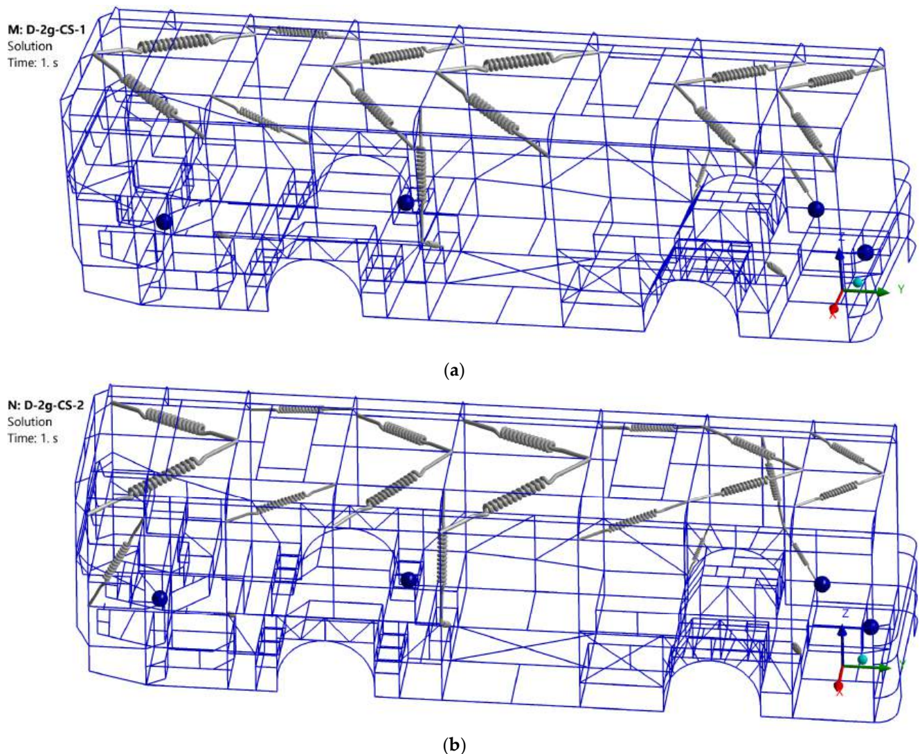
Figure 18. Representative one-directional CS layouts used for verification of the numerical screening procedure: (a) D-2g-CS-1, with Cable Spring diagonals predominantly inclined opposite to the direction of vehicle travel; (b) D-2g-CS-2, with Cable Spring diagonals predominantly inclined in the direction of travel.
