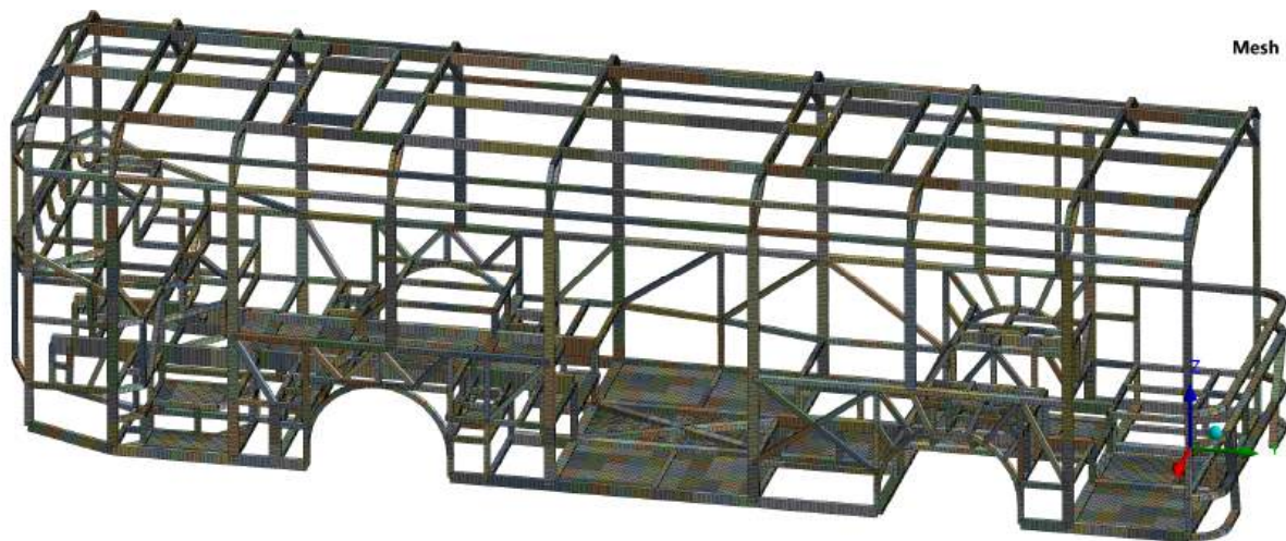
Figure 5. FEA mesh of the bus body model “4289”.
