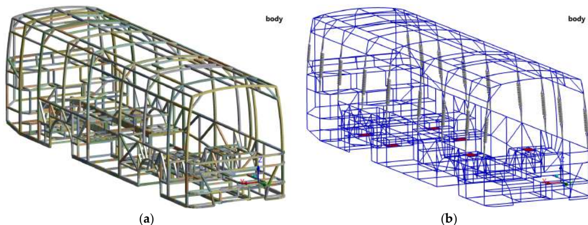
Figure 8. Catenary-curved body-frame Ansys model: (a) R100-6.6g-c/R100-5g-c. (b) R100-6.6g-c-CS/R100-5g-c-CS with integrated Cable Spring joints.
