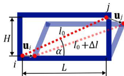
Figure 1. Simplified rectangular frame cell reinforced by a prestressed diagonal cable.
