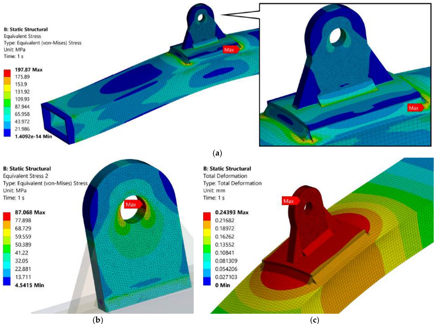
Figure 16. Results of the component-level finite-element analysis of the representative CS anchorage: (a) global equivalent stress distribution with local stress concentration in the welded support region; (b) stress distribution in the lug plate; (c) total deformation.
