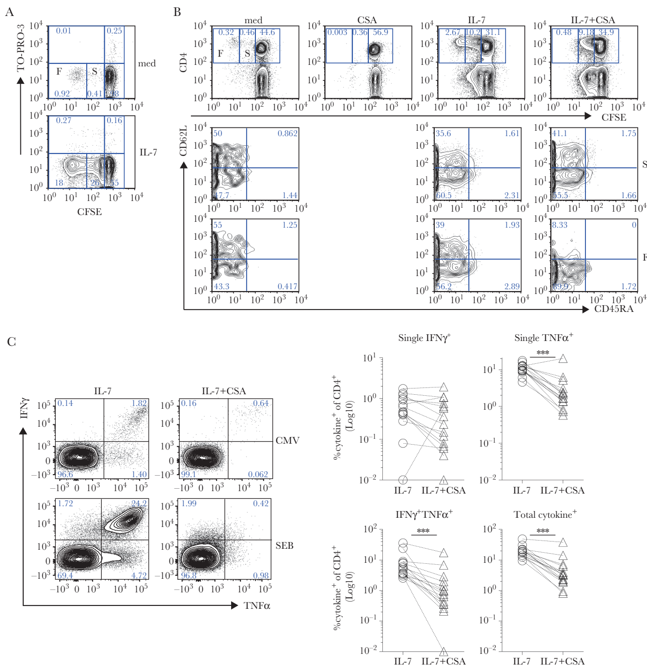
Figure 5. Sensitization by interleukin (IL)-7 promotes pathogen-specific CD4 + T cell proliferation in a cyclosporine A (CSA)-sensitive manner. 5-(and-6)-carboxyfluorescein diacetate succinimyl ester (CFSE)-labeled peripheral blood mononuclear cells (PBMCs) (A–C) from healthy donors (A and B) were cultured for 7 days in the absence (med) or presence of human recombinant IL-7 (IL-7). (A) Proliferation of viable CD4 + T cells in high-density cultures ( 5 \times 10^6 cells/mL) was determined by flow cytometry after staining with anti-CD4 monoclonal antibody (mAb) and TO-PRO-3 (an intercalant agent of deoxyribonucleic acid entering necrotic and apoptotic cells). Contour plots depict the relative CFSE content within the same number of viable, TO-PRO-3 + CD4 + T cells. (B) Cells cultured ( 4 \times 10^6 cells/mL) in the presence of IL-7 for 7 days in the absence or in the presence of CSA. At d7, cells were stained with anti-CD4, anti-CD45RA, and anti-CD62L mAb, and the relative CFSE content was analyzed by flow cytometry in total CD4 + T cells (top row). Fast- (F), slow- (S), and nondividing cells were determined based on CSA inhibition, as indicated. The percentage of naive (CD45RA + CD62L hi ), central memory (CD45RA + CD62L hi ), and effector memory (CD45RA + CD62L lo ) cells were then investigated in slow- compared with fast-proliferating CD4 + T cells. (C) Freshly isolated PBMCs were rested for 5 days then incubated for 1 week in IL-7 or IL-7 plus CSA (IL-7+CSA). At d12, cells were stimulated with Staphylococcus aureus enterotoxin B (SEB) during an intracellular cytokine staining (ICS) assay to test antigen-specific tumor necrosis factor (TNF) \alpha and interferon (IFN)- \gamma release, compared with unstimulated controls (refer to Figures 3 and 4). Left dot plots show that the IL-7-driven accumulation of (top) cytomegalovirus (CMV)- and (bottom) SEB-specific CD4 + T cells producing TNF \alpha and/or IFN \gamma is reversed in the presence of CSA, by d12. After subtraction of individual background levels of IFN \gamma + , TNF \alpha + , and IFN \gamma + TNF \alpha + CD4 + T cells detected in unstimulated controls (nil), the percentage of SEB-specific cytokine + (IFN \gamma + , TNF \alpha + , IFN \gamma + TNF \alpha + , and total) CD4 + T cells was evaluated in 15 independent biological replicates in IL-7 (open circles) compared with IL-7+CSA cultures (open triangles). The right graphs show a statistically significant decrease in the frequency (Log 10 ) of SEB-specific cytokine + (except for IFN \gamma + ) CD4 + T cells in the presence of CSA at d12. All tests are paired Wilcoxon tests; *, P \leq .05 ; **, P \leq .005 ; ***, P \leq .0005 .
