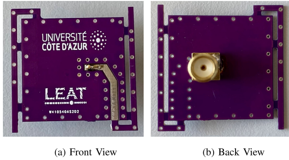
FIGURE 9. End-launcher prototype.
