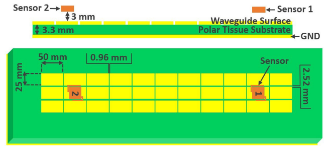
FIGURE 4. Waveguide surface structure.
