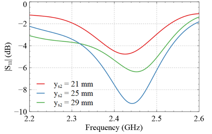
FIGURE 3. End-launcher impedance matching for different y_{s2} values.
