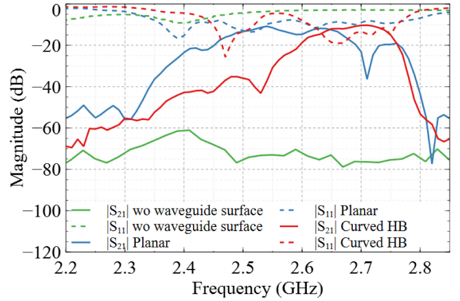
FIGURE 11. S-Parameters measurements.
