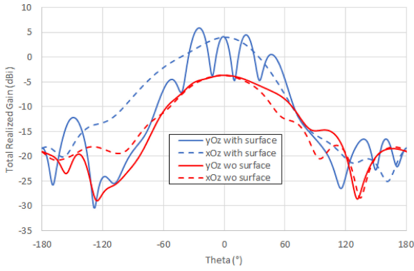
FIGURE 8. Simulated end-launcher radiation pattern with and without the waveguided surface over the human body.
