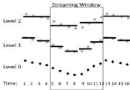
Figure 6: Multilevel Summarization
