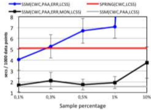
Figure 9: Runtime vs Sample Percentage for SSM
