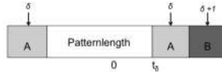
Figure 7: Sequence Placement in Streaming Window at t_0
