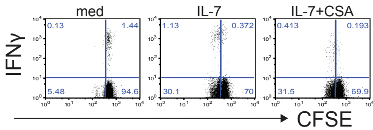
Supplementary Figure 6. Sensitization by IL-7 promotes MTB-specific CD4 + T cells proliferation in CSA-sensitive manner. CFSE-labelled PBMCs derived from TB Pt.#1 (as shown in Fig.1B) were analyzed after a 7-day culture in IL-7 (IL-7) and IL-7 plus CSA (IL-7+CSA) compared to control medium (med). At d7, cells were stimulated with MTP-pulsed autologous irradiated PBMCs and IFN \gamma release was determined by ICS. Events are shown after gating on viable CD4 + T cells.
