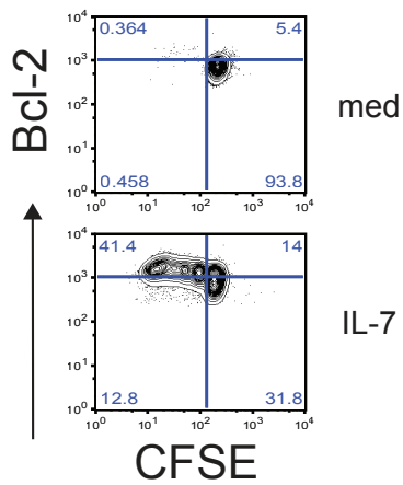
Supplementary Figure 3. Cells cultured in IL-7 upregulate Bcl-2 while proliferating in vitro. CFSE-labeled PBMCs derived from healthy donors were cultured ( 5 \times 10^6 cells/ml) for 7 days with (IL-7) or without IL-7 (med). At d7, proliferation was assessed alongside the expression of the pro-survival mediator (Bcl-2) in flow cytometry. The small frequency of cells autoproliferating in the absence of IL-7 tended to show higher Bcl-2 levels than not-dividing CD4 T cells. Addition of IL-7 supported the proliferation of CD4 T cells alongside the upregulation of the anti-apoptotic factor, Bcl-2.
