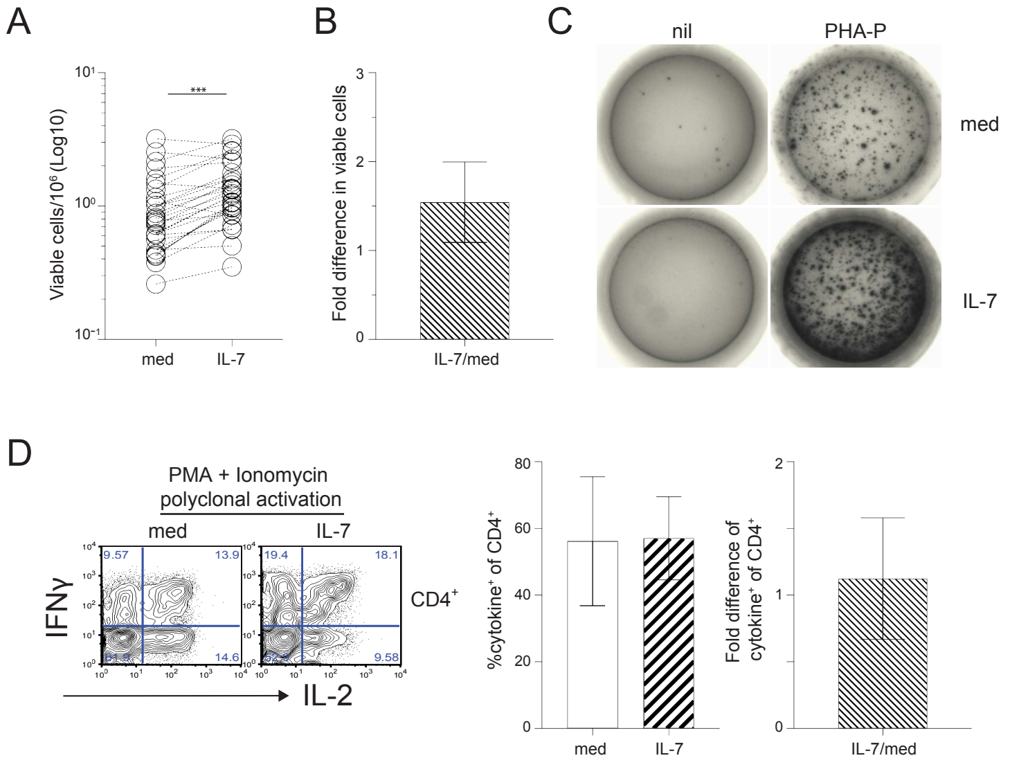
Supplementary Figure 7. IL-7 enhances total cell recovery and non-specific IFN \gamma secretion, but does not increase the total cytokine secretion by CD4 T cells. (A-D) At d0, equal number of viable PBMCs were seeded in culture with IL-7 (IL-7) and control media (med). (A-B) After a 7-day culture, alive cells were counted as 0.1% Trypan Blue negative cells. A. The plot shows total viable cell recovery in complete media (med) compared to IL-7 (IL-7) in many independent biological replicates ( n=30 ). IL-7 significantly enhanced total cell recovery ( p<0.0001 , Wilcoxon matched-pair test). B. For each independent pair ( n=30 ), the fold-increase in viable cells was calculated as a ratio between the cell numbers detected in the culture in IL-7 compared to that in complete media (IL7/med). The graph shows that, on average, total viable cells increased by \sim 1.5 fold, upon exposure to IL-7. C. PBMCs derived from a representative donor were analyzed for the release of the effector cytokine, IFN \gamma by ELISPOT after a 7-day culture in the absence (med, upper wells) or in the presence of human recombinant IL-7 (IL-7, lower wells). IFN \gamma release was measured in unstimulated negative control wells (nil, wells on the left) compared to the ELISPOT positive control, PHA-P stimulation (wells on the right). In agreement with A-B, the total number of spots tended to increase after the IL-7 culture. D. In order to measure whether polyclonal CD4 ^+ T cells generally benefit from the IL-7 culture, PBMCs cultured for 7 days in complete media (med) or with IL-7 (IL-7) were stimulated with PMA and Ionomycin (polyclonal stimulation: 50 ng/ml and 1 \mu g/ml, respectively) in ICS assay (refer to Materials and Methods for details). Then, polyclonal IFN \gamma /IL2 release was analyzed in gated CD4 ^+ T cells (left contour plots). When average percentages of total cytokine ^+ (IFN \gamma^+ and/or IL2 ^+ ) CD4 ^+ T cells were evaluated in cultures derived from 5 independent donors (middle bar graph), no significant difference was observed in IL-7 (black striped bar) compared to control medium (white bar) cultures (Wilcoxon matched-pairs signed rank test). The right graph shows the average ratio of percentage of cytokine ^+ CD4 ^+ T cells between the IL-7 and control media culture (IL7/med).
