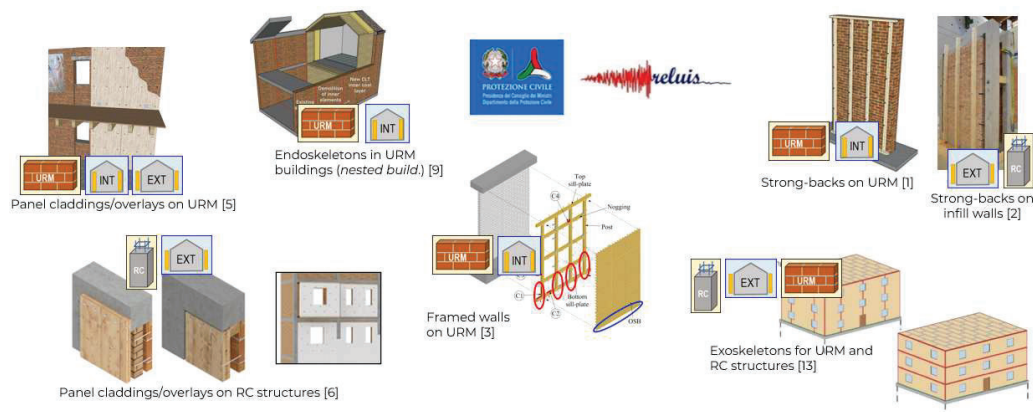
Figure 1 Synthesis of timber-based strengthening techniques for URM and RC structures studied within the ReLUIS-DPC project
