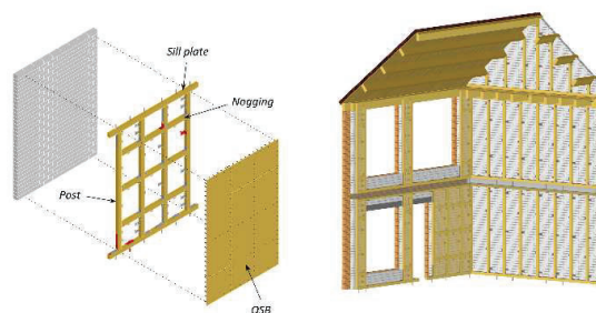
Figure 3 Retrofit with timber-framed walls: overview of the strengthening system—layout, components (left), and application to an existing masonry building (right) [3]
