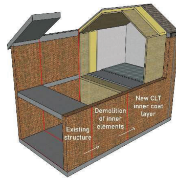
Figure 6 Application scheme of timber endoskeletons on masonry buildings (nested buildings solution) [9]
