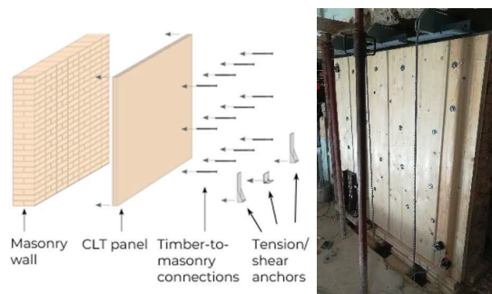
Figure 4 CLT panel retrofit of masonry buildings: components (left) and in-situ testing (right)[11]
