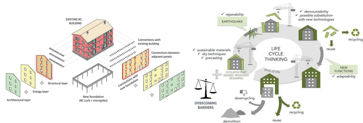
Figure 9 General concept of integrated retrofit with exoskeleton in an LCT perspective (left picture adapted from [35]; right picture from [18];
