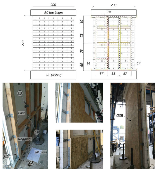
Figure 8 Retrofit with timber-framed walls: geometry and details of the strengthening system [3]
