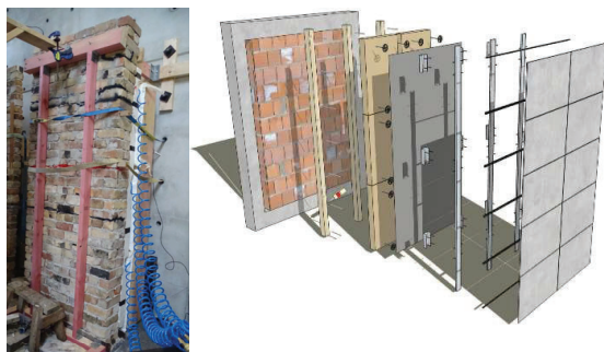
Figure 2 Timber strong-back retrofit applied to masonry walls [1] (left) and to infill walls [2] (right)
