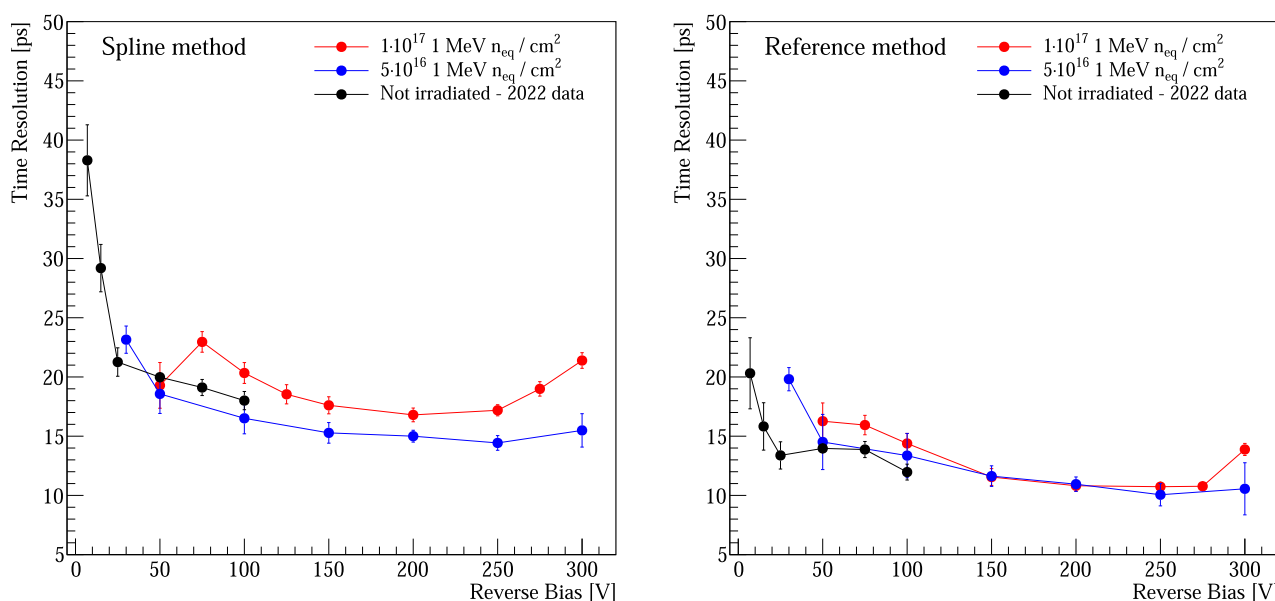
FIGURE 11 Time resolution of the single-pixels as a function of the reverse bias voltage for the different irradiation fluences obtained with the (right) reference method and (left) spline method. The contribution due to the resolution of the time reference is subtracted.
