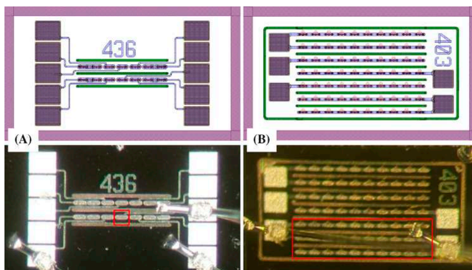
FIGURE 2 Layout and pictures of the 3D trench test structures tested at the CERN SPS: the single-pixel sensor (A) and the triple-strip sensor (B). For each structure the active area is outlined in red and is equal to 55\ \mu\text{m} \times 55\ \mu\text{m} for the single-pixel and 165\ \mu\text{m} \times 550\ \mu\text{m} for the triple-strip sensor.
