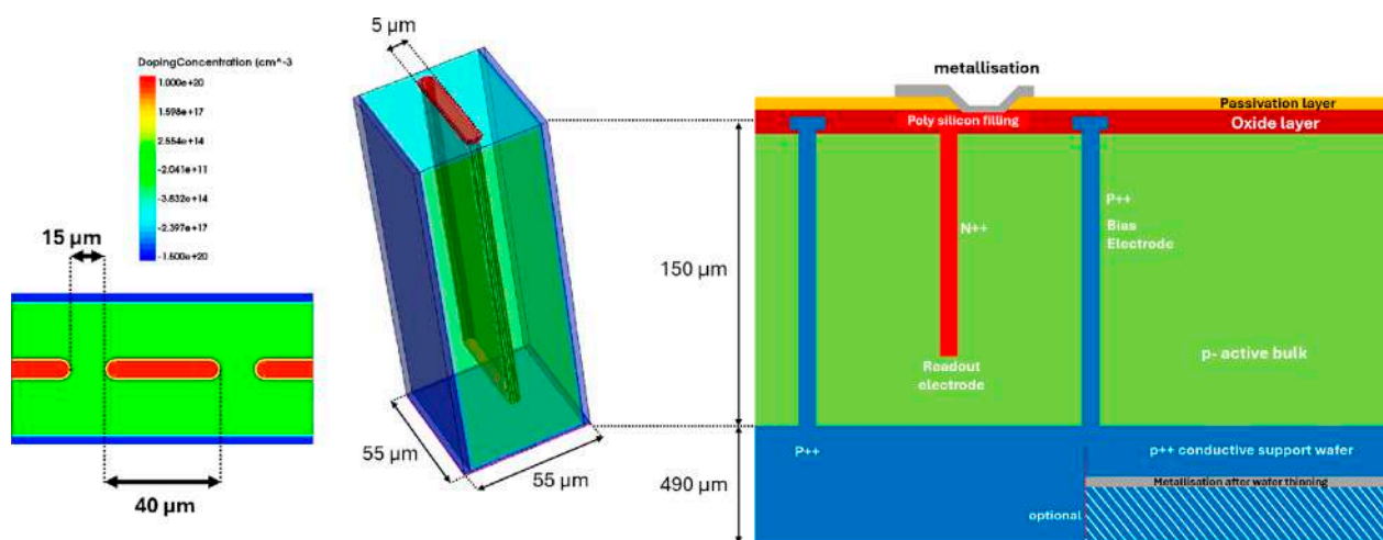
FIGURE 1 Structure and technological profile of the 3D trench sensor developed within the TimeSPOT project.
