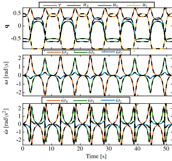
Fig. 2. Reproduction of a rhythmic motion using Quat-pDMP. Top : shows the quaternion components. Middle : shows the angular velocity components. Bottom : shows the angular acceleration components. Dashed black lines represent the synthetic periodic orientation trajectory, while solid colored lines represent the encoded trajectory using Quat-pDMP. (For interpretation of the references to color in this figure legend, the reader is referred to the web version of this article.)
