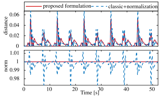
Fig. 3. Comparison between Quat-pDMP and baseline (classical PDMP + normalization). Top : Compares the distance between the demonstration and a reproduction using Quat-pDMP and the baseline. Bottom : Illustrates both norms resulting from Quat-pDMP and the baseline without normalization. (For interpretation of the references to color in this figure legend, the reader is referred to the web version of this article.)
