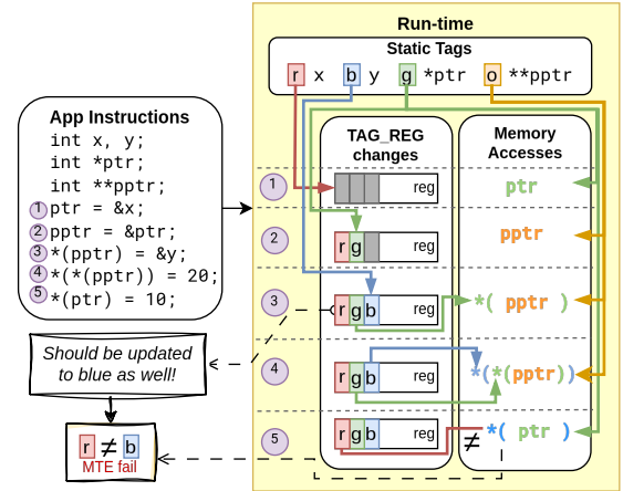
Figure 10: Tag integrity issue with pointer aliasing. After the ptr alias created at ②, instruction ③ should change the TAGShield state for both *(ptr) and *(pptr) . Failing to do so will cause an MTE failure on ⑤.
