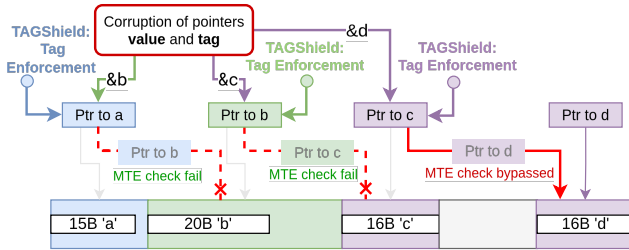
Figure 6: Adversary corrupting both the pointer tag and value with TAGShield enabled. TAGShield prevents the bypass when the corrupted tag mismatches the authentic tag.
