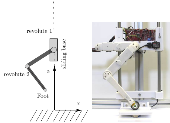
Fig. 1. Structure of the monoped and the real platform, courtesy of Max Planck Gesellschaft
