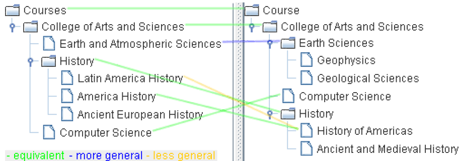
Figure 3: Result of the minimal semantic matching algorithm.
