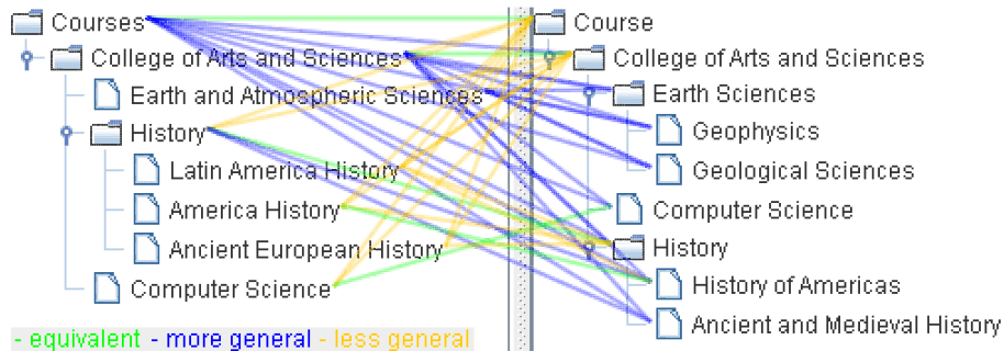
Figure 2: Result of the basic semantic matching algorithm.
