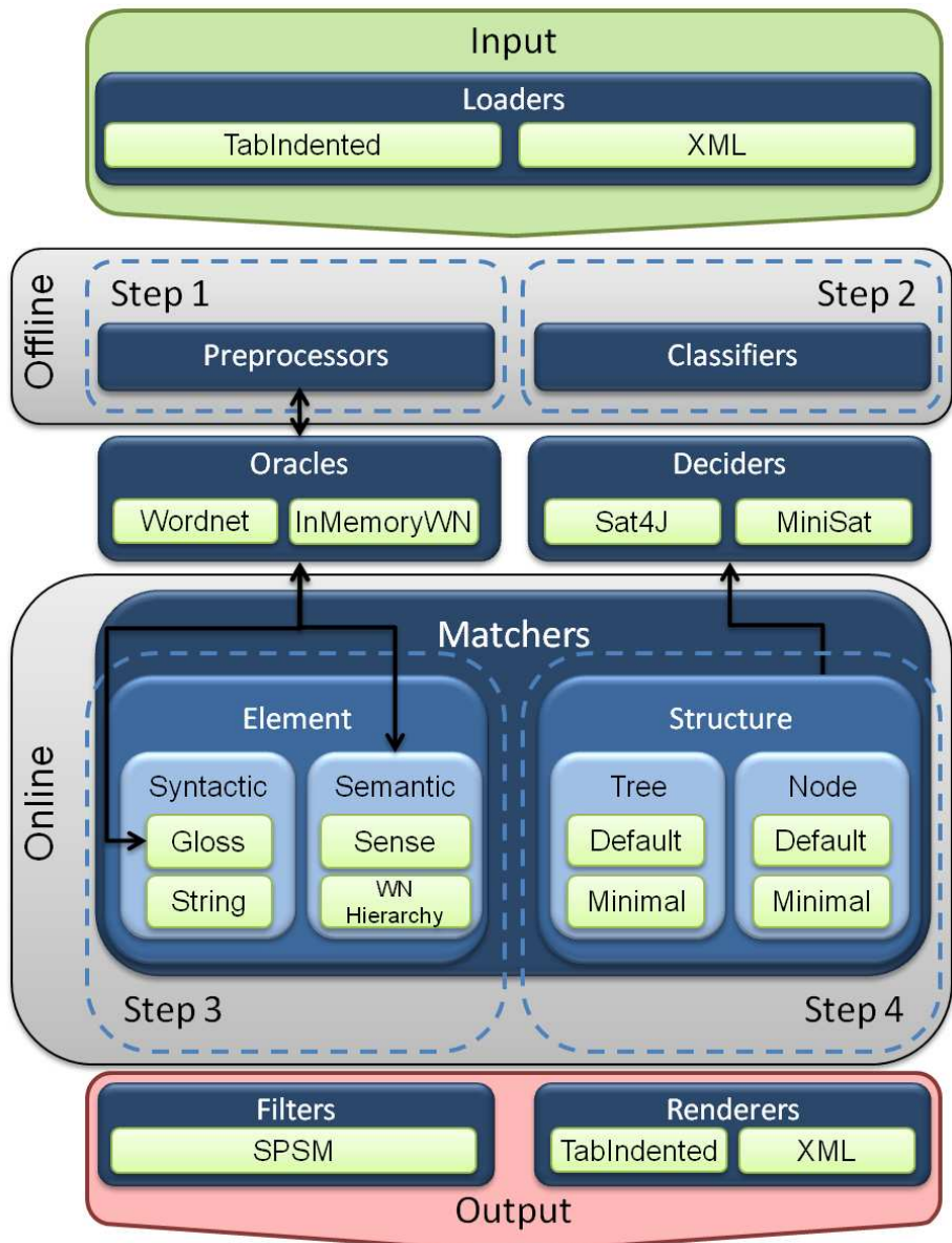
Figure 5: S-Match architecture
