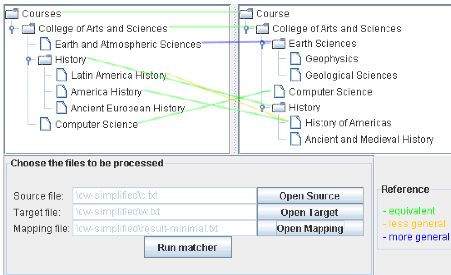
Figure 7: S-Match GUI with course catalogs and a mapping loaded
