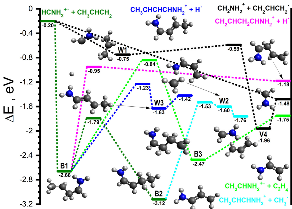
Fig. 6 Schematic potential energy surface for the reaction of \text{HCNH}_2^{+\bullet} with \text{CH}_3\text{CHCH}_2 . To allow for a direct comparison with the PESs shown in Fig. 3–5, the zero of the energy scale (in eV) is given by the sum of the energies of the separated \text{H}_2\text{CNH}_2^{+\bullet} plus \text{CH}_3\text{CHCH}_2 reactants. Calculations are at the CCSD(T)/6-311++G(d,p) level of theory. Molecular structures are shown only for intermediates and products, with TS structures given in the (ESI†).
