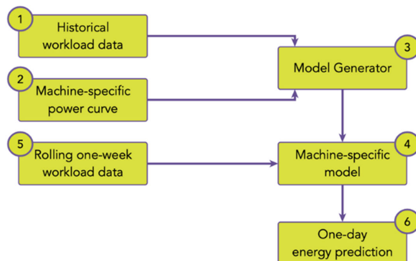
Figure 5. Architecture of the workload prediction model.
