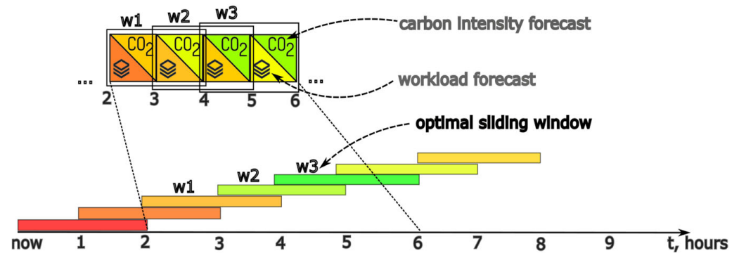
Figure 4. Calculation of the optimal sliding window.
