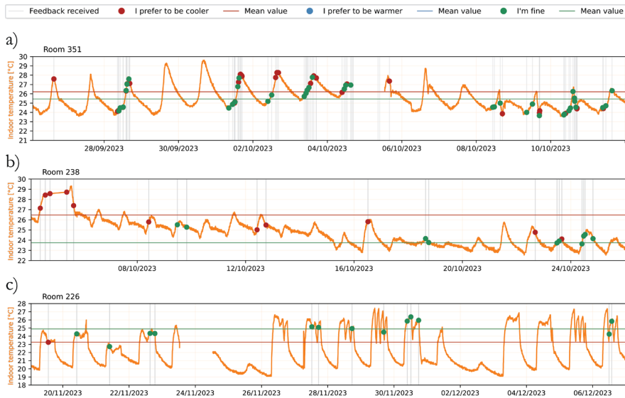
Fig. 6.14 Indoor temperatures in Office 351 (a), Photography Lab 238 (b), and History Lab (c): dots represent thermal feedback from the micro-survey conducted with Cozie. Each dot aligns with the specific time the survey was completed and reflects the corresponding temperature recorded at that moment
