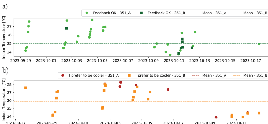
Fig. 6.15 Thermal feedback from the two office 351 users: “No change” (a) and “I prefer to be cooler” (b) Each dot aligns with the specific time the survey was completed and reflects the corresponding temperature recorded at that moment
