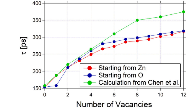
Fig. 8. Calculated positron lifetimes (ATSUP code, BN scheme) for spherical vacancy clusters with increasing size, starting from Zn or O as center atom, plus calculations from Chen et al. [62].
