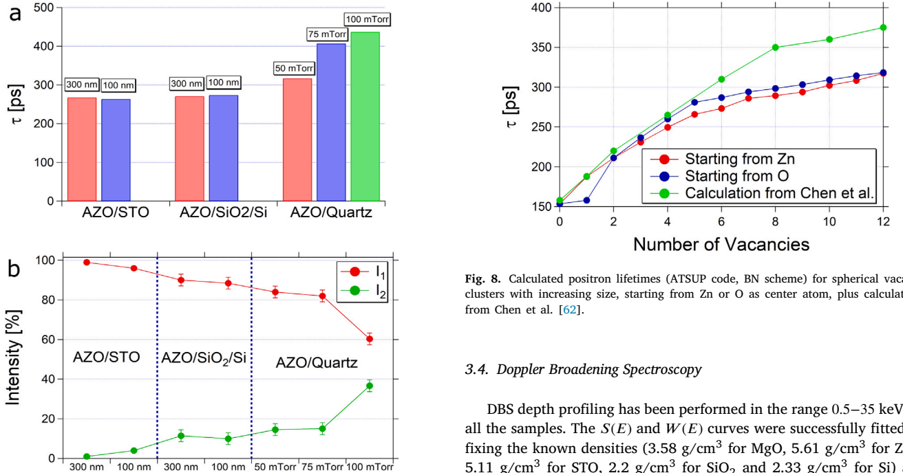
Fig. 7. (a) Average positron lifetime and (b) average intensities of the first two components of the lifetime spectra in the AZO films deposited on different substrates.
