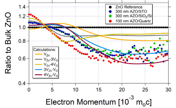
Fig. 11. CDBS ratio curves to ZnO of the selected samples together with ATSUP calculations of some small vacancy clusters included.
