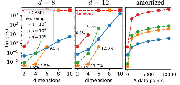
Figure 4: Left and center : runtime of GASP! and rejection sampling (using 10^{\{2,4,6\}} samples) on integrals over 4 random simplices for increasing dimensions. We report the relative error (%) for rejection sampling. Right : Our amortization speed-up compared to rejection-sampling in 2-dimensions for the 12-degree polynomial. Fig. 12 shows more results for different degrees and constraints.
