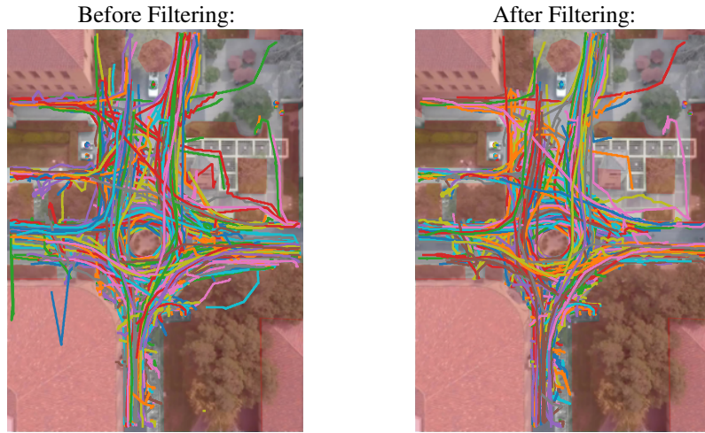
Figure 13: The trajectories before/after filtering for image 12 in the Stanford Drone Dataset. The constraints are shown in red.
