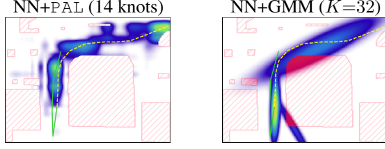
Figure 9: PAL wraps around the boundaries of our constraints , in contrast to the NN with an GMM, which predicts a trajectory straight through the constraint. The observed test trajectory and ground-truth completion on scenario 2 are reported in green/solid and dashed/yellow respectively.
