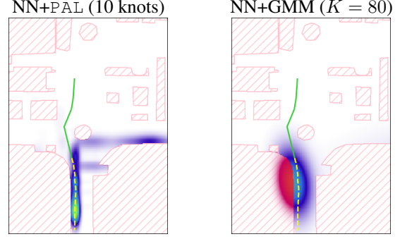
Figure 8: PAL captures meaningful modes when modelling how a trajectory might evolve ( p(\mathbf{Y} | \mathbf{X}) ) while never violating the constraint differently from a NN with a GMM output. The observed test trajectory and ground-truth on scenario 1 completion are reported in green/solid and dashed/yellow. Additional plots in Table 20.
