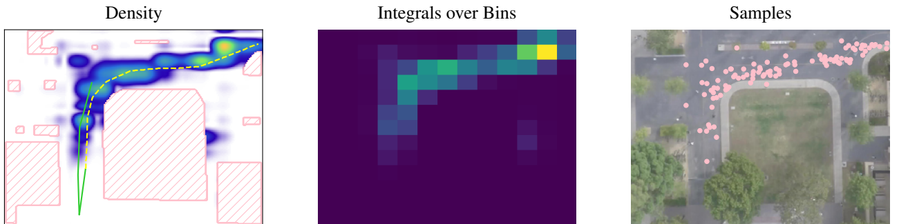
Figure 15: The obtained samples from our sampling procedure applied to Sample 1 from 23 for the model PAL 14/medium. On the left one can see the ground truth density of our spline-based PAL-model, followed by the integral over the bins. On the right, we show the 100 samples drawn by applying algorithm 7.
