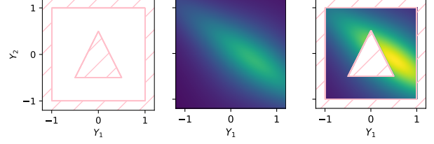
Figure 2: A renormalized constrained density (right) obtained by applying non-convex algebraic constraints (left) over an unconstrained distribution (middle).
