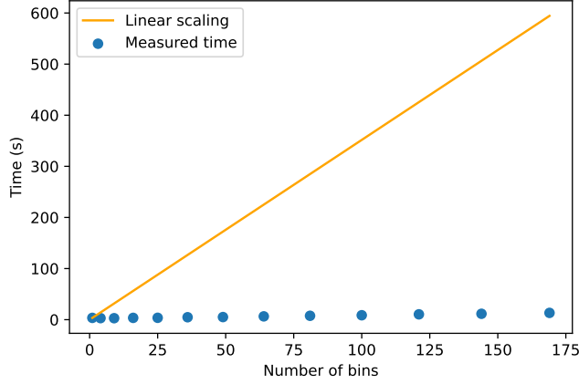
Figure 11: The integration time for splines on the Stanford drone dataset (scene 1) does not grow linearly with the number of bins. In this figure, we compare the time it takes to integrate our squared spline for an increasing number of bins versus a simple linear scaling, which we would expect if the empirical computational complexity per bin would stay approximately constant.
