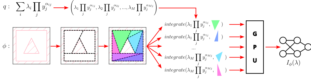
Figure 3: An overview of our pipeline with GASP! . The integrand q is decomposed into parallelizable monomial integrations ( top ). The non-convex constraint is first decomposed into several convex regions (Appendix A) that are further decomposed into (colored) simplices ( bottom ). The resulting computational graph is highly parallelizable on a GPU.
