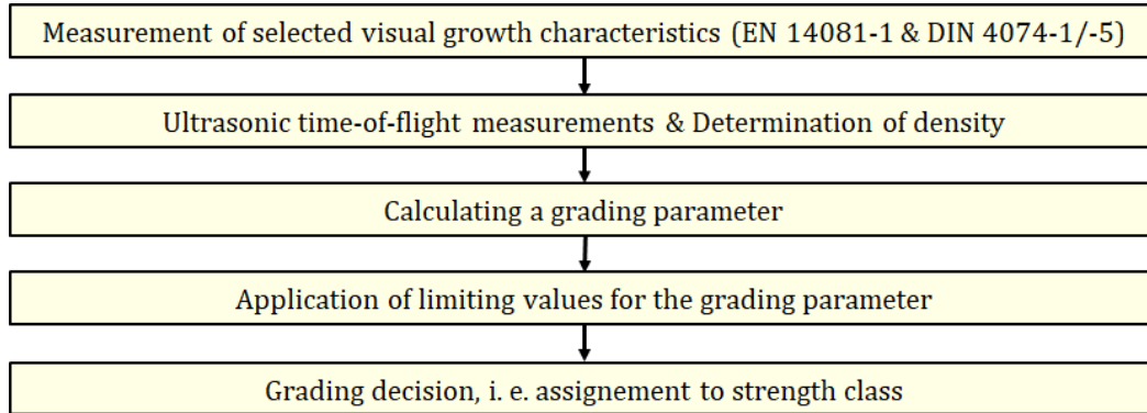
Figure 3. Process of the in-situ strength grading methodology
