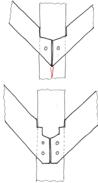
Figure 5 a) and b). Dovetail lap joints have too small an angle ( <10^\circ ). When positioning two adjoining dovetail laps, poor alignment can cause wedge-like action, resulting in splitting of the post. To address this issue, refer to the suggested joint for this purpose located at the lower right.
