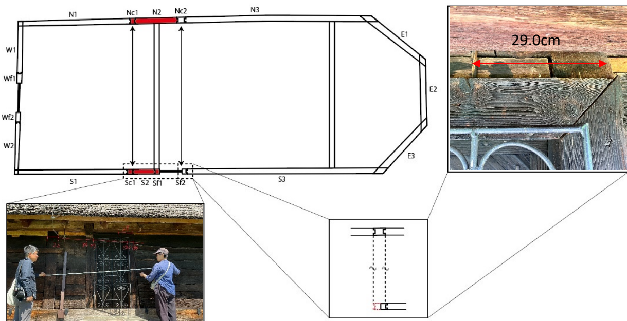
Figure 9. Structure of the beams and girders placed on the upper planks
