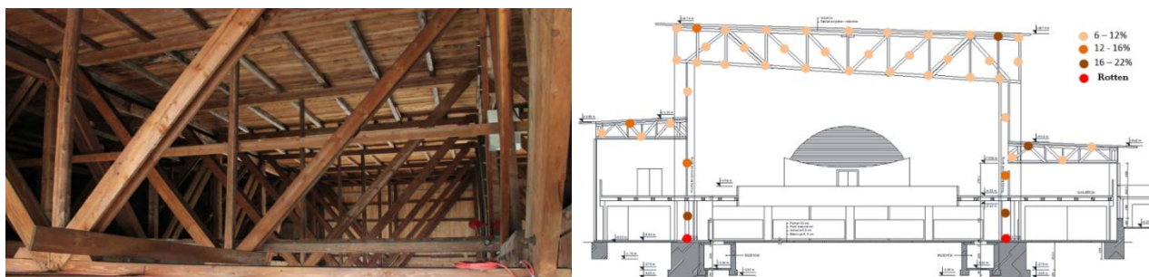
Figure 3. Measurement of the moisture content in roof timber trusses
