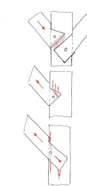
Figure 4 a)-c). Church of St. Michael Archangel, Prelošćica, 1832. Shown here are examples of curiously misshapen blind dovetail laps of knee brackets. The structural problems are as follows: depending on the load, the wood fails in compression perpendicular to fibres (compression) or splits in shear or tension perpendicular to fibres (tension). Additionally, positioning wooden pegs too close to the edge of the post can cause the post to split along its grain. These issues suggest that the church was presumably built by local carpenters with limited experience in carpentry.
