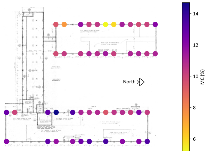
Figure 37. A modified blueprint of the Oak Creek Building [22] overlayed with each column's measured MC (if it was taken). Please note that the top row of measurements was taken five days before the rest and is not necessarily directly comparable.
