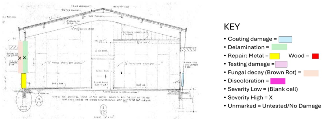
Figure 35. A sample condition assessment map for one of the portals overlaid on a diagram from the blueprints [18], detailing the nature and location of observed deterioration and damage, as well as including a key for identification of observed damage.
