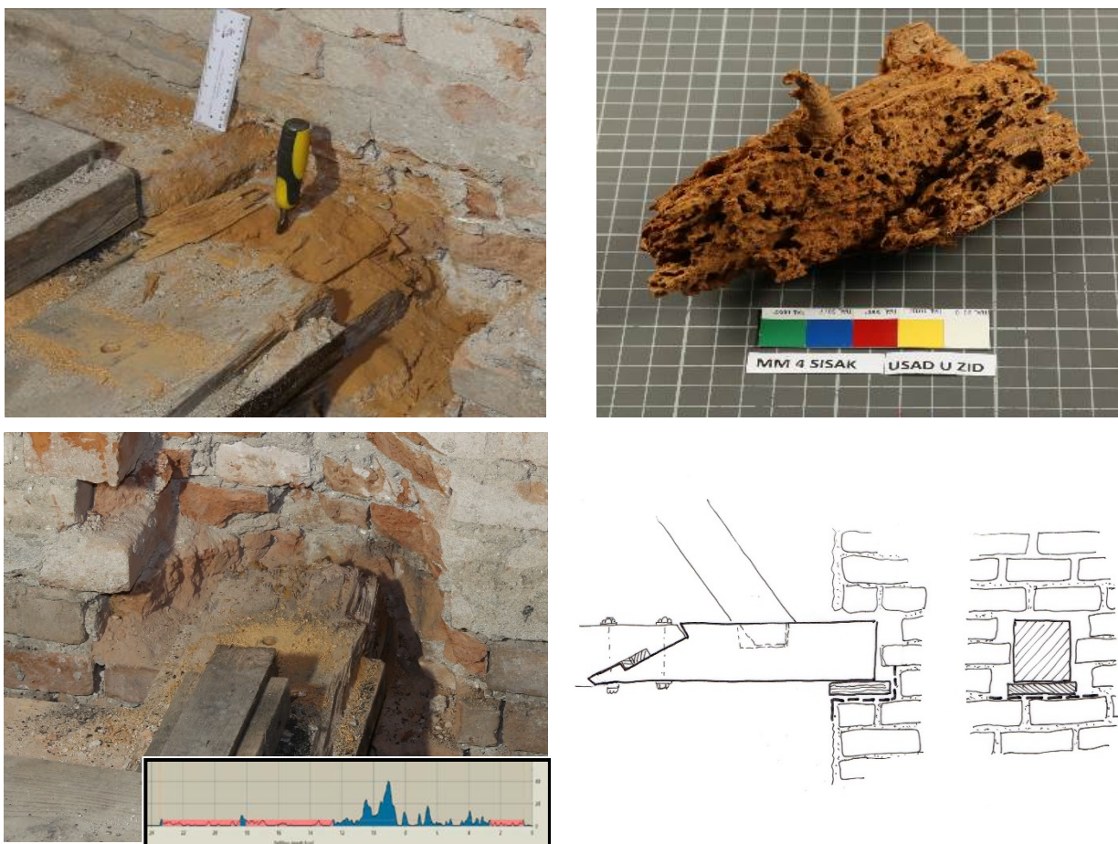
Figure 3. Regular problems with the wood beam inserts in the wall. Photographs: whenever the beam is built in tightly, with no insulation or ventilation, total damage occurs. The sketch represents the optimal firm insert of the beam into the wall, insulated from moisture at least from below, and ventilated by alternate shifting of bricks at the end grain and the sides.
