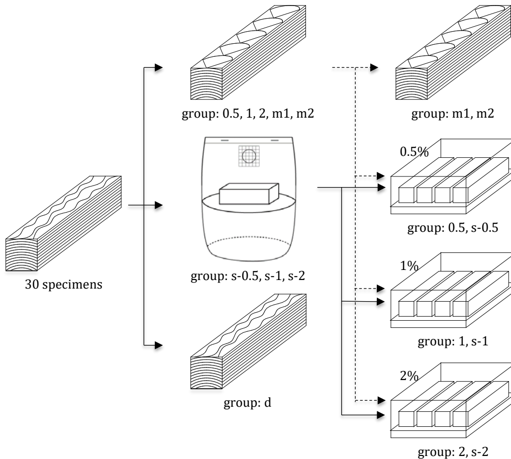
Figure 6. Test flow
