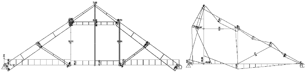
Figure 9. (a) Axial forces in a Queen-post truss and (b) bending moment in a half-truss
