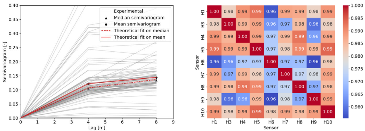
a) Experimental and fitted theoretical semivariograms b) Correlation matrix for humidity sensors on the roof
