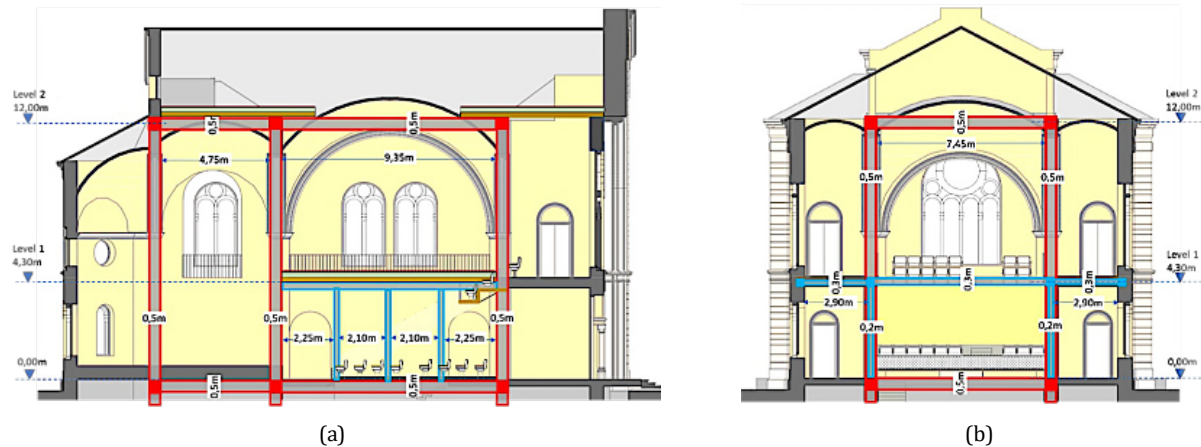
Figure 3. Concept of retrofitted and added structural elements: longitudinal (East-West) (a) and lateral (South-North) (b) cross-section of building.
