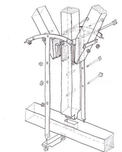
Figure 17 a) – d). This analysis shows the jointing sequence between the king post, tie beam, and supporting struts of the main aisle (two variants). The connections begin with housing and notched mortise and tenon joints, followed by the fitting of heavy ironmongery to secure tightness in all joints. Perfect craftsmanship and joint condition are observed.
