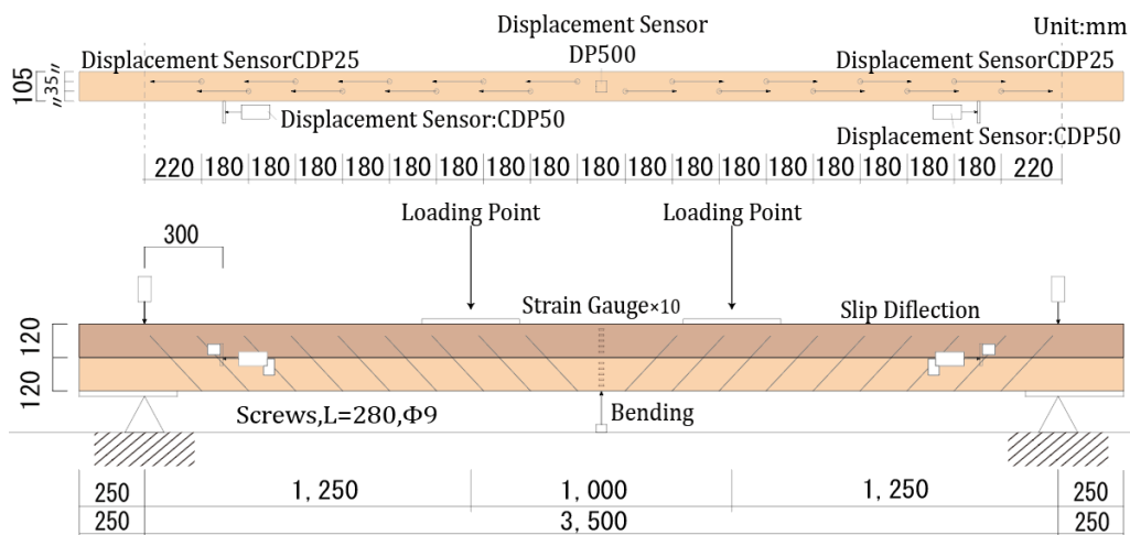
Figure 2. Overview of the test specimens for the short-term test
