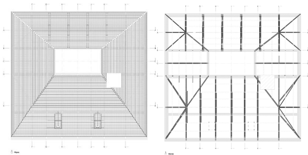
Figure 10. Roof of the Town council with (a) 8 slopes, 2 dormers and secondary structure and (b) main structure
