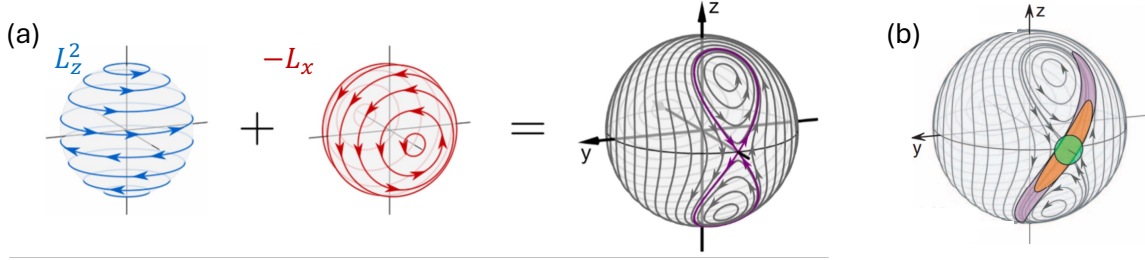
Figure 4.2. Spin-squeezing via one-axis twisting Hamiltonian. (a) Pictorial mean-field representation of the two contributions on the collective Bloch sphere, coming from the nonlinear term \hat{L}_z^2 and rotation term \hat{L}_x , which leads in combination to the bifurcated phase space, where the arrow indicates the existence of an unstable point. (b) If a state is initiated in that unstable fixed point, under the dynamics (will follow the arrow), its quasi-probability distribution will stretch along the lines, and in the orthogonal direction, it will be squeezed. Adapted from Ref. [358].
