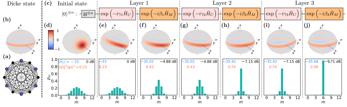
Figure 4.4. Metrologically useful squeezing generated by a depth-three QAOA for the MaxCut problem in a complete graph of 12 nodes. (a) Fully connected unweighted graph with the nodes and edges colored according to one of the 924 possible maximum cut configurations. (b) Wigner quasi-probability distribution of the symmetric Dicke state D_6^{12} , an idealized example of a squeezed state, and the target for our QAOA. (c) Circuit representation of QAOA with alternating application of cost-function and mixer Hamiltonian. The Bloch spheres and histograms from (d) to (j) show the state after the corresponding gate in the optimized QAOA circuit with (\gamma_i, \beta_i) given by (0.199, 0.127) , (0.306, 0.087) , and (4.592, 1.518) for i = 1, 2 , and 3 , respectively. Negativity in the Wigner distribution indicates that the states are non-Gaussian [370]. The squeezing (in black), energy expectation \langle \hat{H}_C \rangle (in blue), and overlap probability density |\langle D_6^{12} | \psi \rangle|^2 with the target Dicke state (in orange) are shown inside each histogram.
