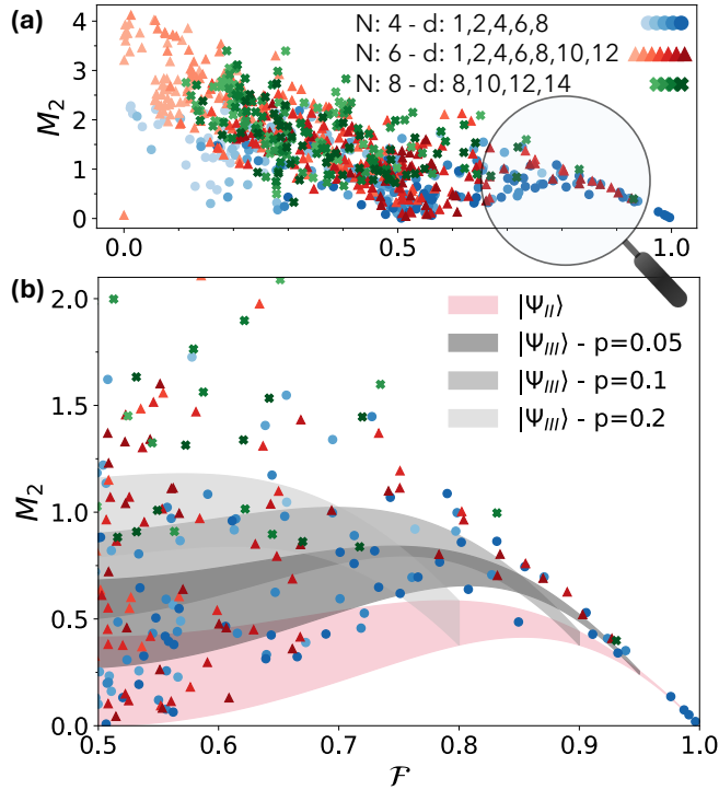
Figure 7.3. Relation between final magic and fidelity (qubits).
