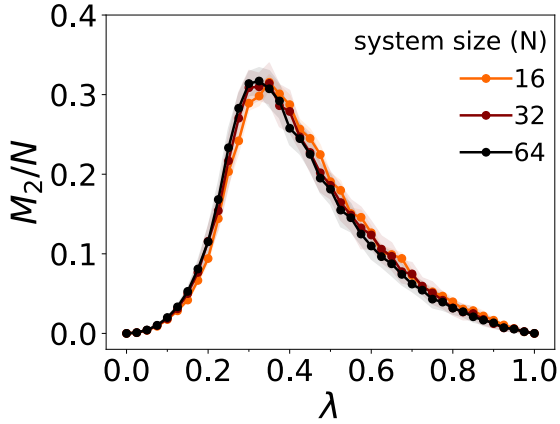
Figure 7.8. Magic barrier in quantum annealing The SRE density, computed on the ground state of the instantaneous Hamiltonian (ideal adiabatic quantum annealing, \lambda \in [0, 1] ), exhibits a magic barrier around \lambda \sim 0.35 . The nearly overlapping curves for N = 16, 32, 64 indicate the SRE density traces a barrier largely independent of system size.
