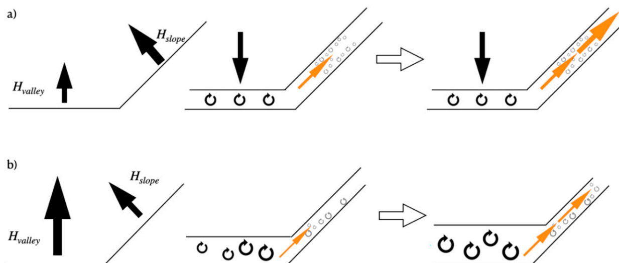
FIG. 12. Schematization of the morning transition and erosion of the nocturnal inversion processes, showing the two possible mechanisms of erosion (b) from below (due to surface heating) or (a) from above (due to mixing). Notice that the role of sensible heat is also represented.
