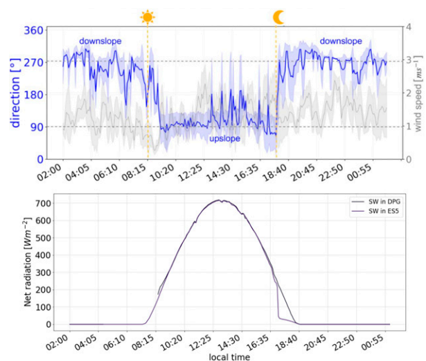
FIG. 4. Time evolution of the average (top) wind direction and speed and (bottom) incoming shortwave radiation during the case F3. For the wind data, the average value is computed using data collected at all towers ES2–ES5, and the associated error (gray band) is identified through the standard deviation. The two vertical dashed lines identify the times of local sunrise and sunset. Data (nondetrended) are averaged over 5 min, and the time in the x axis is local time (MDT). For the radiation data, the two lines refer to the radiation data collected at the highest measurement point on the slope (tower ES5) and on the valley floor (DPG).
