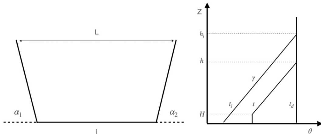
FIG. 8. (left) Valley geometry and (right) potential temperature profile evolution in the Whiteman and McKee (1982) model. The geometrical characteristics of the valley and the temperature profiles are described by introducing the variables represented in the figure, which are then used in the model equations.
