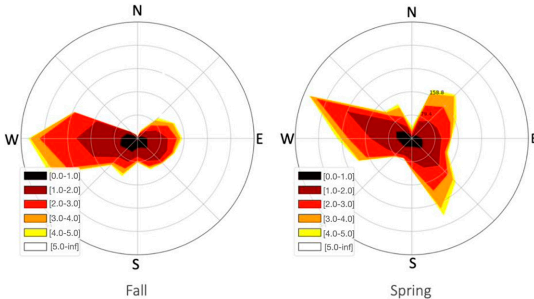
FIG. 3. Wind roses for the entire measurement period in (left) fall 2012 and (right) spring 2013. Analyzed data were collected at tower ES5 and averaged over 15 min. The downslope winds can be identified with a direction of \sim 270^\circ , and the upslope winds have a direction of \sim 90^\circ . The color scale indicates wind strength ranges ( \text{m s}^{-1} ), and the circles refer to 10% intervals of the entire set of values.
