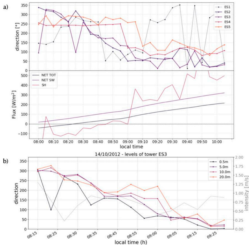
FIG. 6. Initiation of the transition on F3: (a) the scatterplot of the time evolution (MDT) of the averaged wind direction at each tower is reported, along with the evolution of both total and shortwave net radiation (notice that, as expected, ES1 behaves differently from all of the others, because it is located on the valley floor and not on the slope), and (b) the detail on the different levels of tower ES3.
