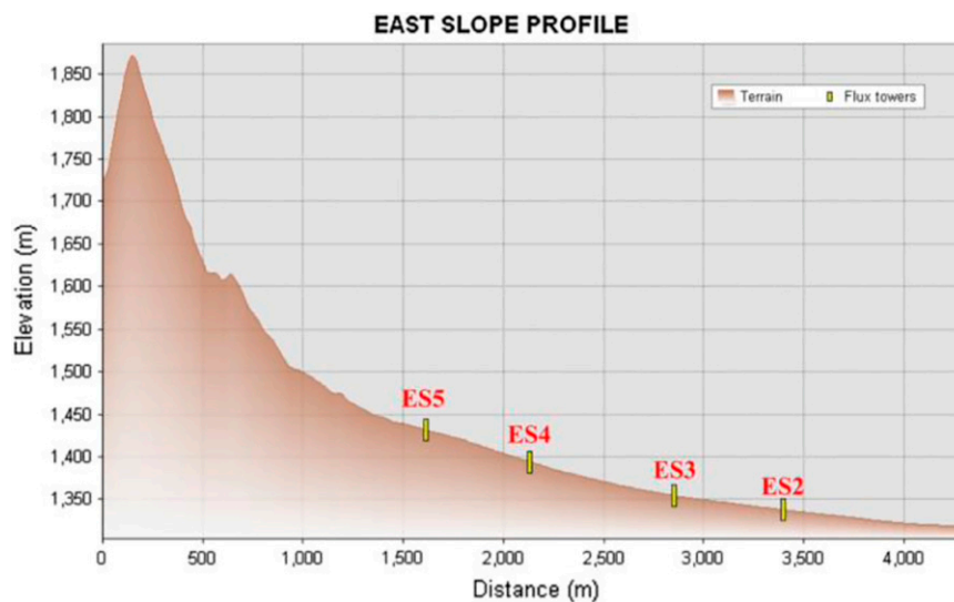
FIG. 2. Layout of the four towers along the ES of Granite Mountain (adapted from Grachev et al. 2016).
