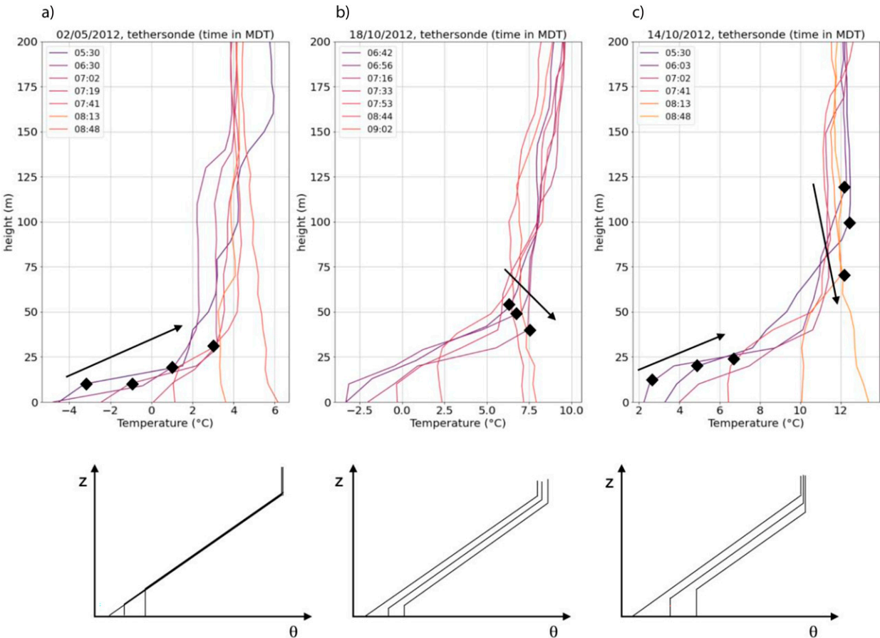
FIG. 7. Examples of patterns of the inversion erosion: (a) upward growth of the CBL, (b) descent of the inversion top, and (c) a mix of the two previous patterns. The three plots represent the time evolution of the vertical temperature profile measured by tethersonde launched from the Sagebrush site. Each line refers to an ascent, identified by the launching time reported in the legend. Data refer to the mornings of S1 [in (a)], F3 [in (b)], and F2 [in (c)], which are also the selected cases for the observation of the upslope winds. A schematic representation of the three patterns is represented below each plot.
