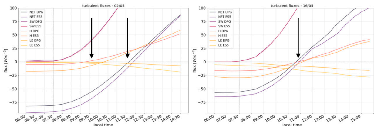
FIG. 11. Time series of energy fluxes on the valley floor (DPG site) and the slope (ESS site) for two selected cases, (left) S1 and (right) S2, in a period centered at sunrise. The vertical dashed line represents local sunrise, and the black arrow highlights the differences between the two cases. The labels in the legend indicate the net radiation (NET), sensible heat flux (SH), and latent heat flux (LE).
