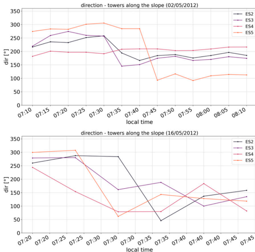
FIG. 10. Expanded view of the evolution of the average wind direction measured at different towers along the slope during two cases taken as examples, (top) S1 and (bottom) S2. Different lines refer to different towers (ES2–ES5) as indicated in the legend. Time on the x axis is local time, and data are averaged over 5-min time windows.
