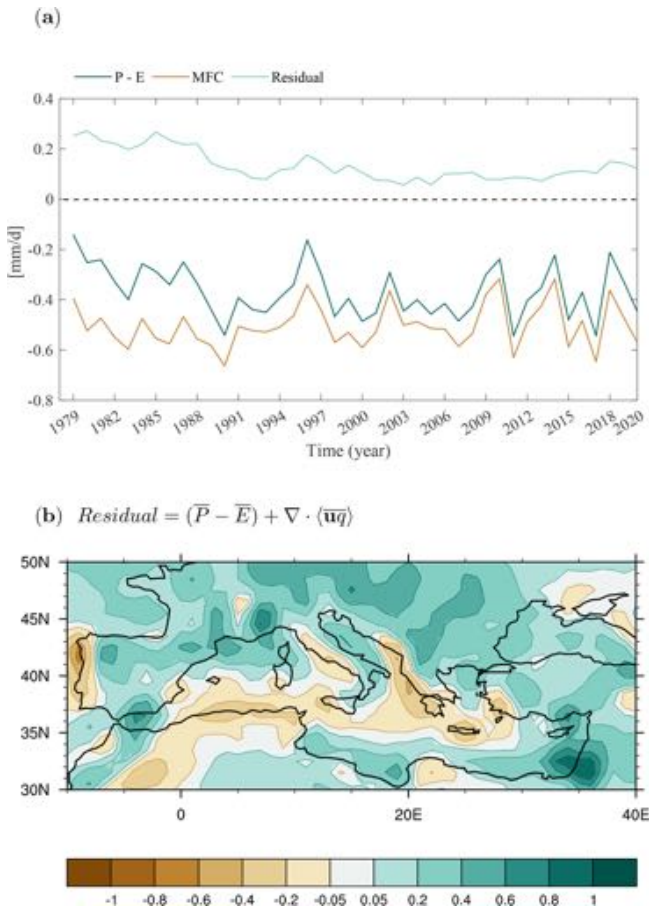
Figure 2. Annual mean moisture budget components in the Mediterranean region from ERA5 in the 1979–2020 period. (a) Temporal evolution of P - E (green line), total moisture flux convergence (MFC; brown line), and the difference between the two (residual, cyan line). (b) Time-averaged spatial variations in the imbalance between P - E and total MFC in millimetres per day. The total MFC is obtained from the publicly published mass-consistent divergence of the vertical integral of moisture flux. See Sect. 2.1 for more details.
