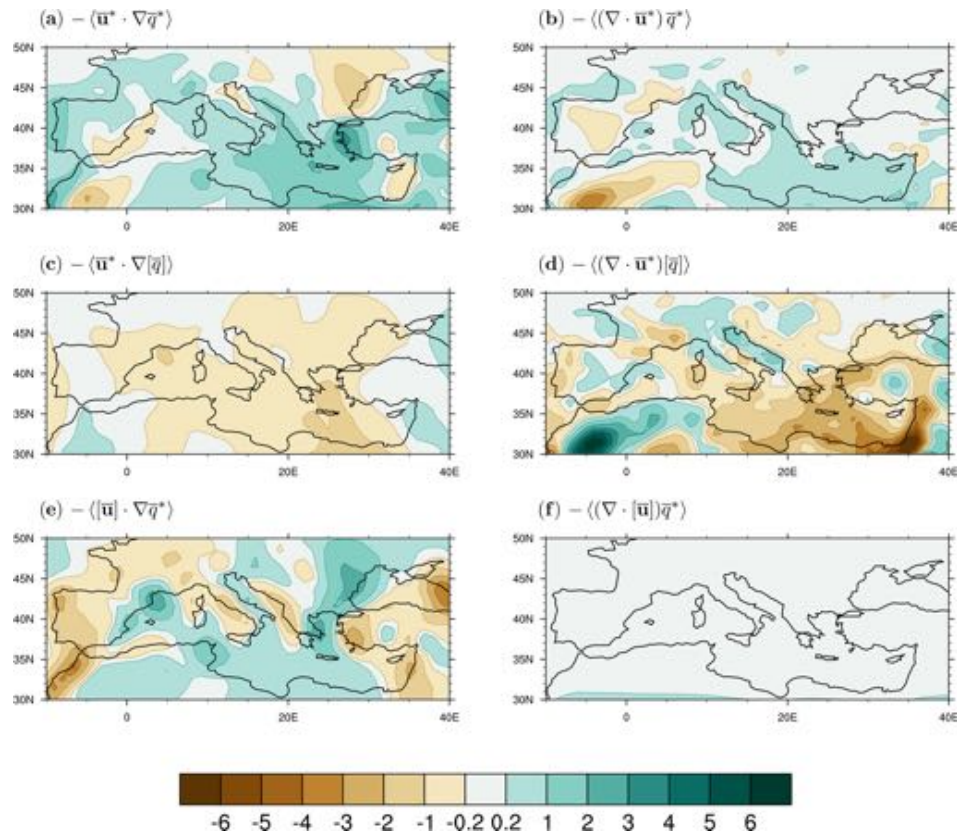
Figure 7. Annual mean climatological contribution from advection (a, c, e) and wind divergence (b, d, f) to the stationary eddy MFC within the Mediterranean region in the 1979–2020 period from ERA5: (a, b) pure stationary eddies, (c, d) zonally anomalous circulation term, and (e, f) zonally anomalous water vapour term. Units are millimetres per day.
