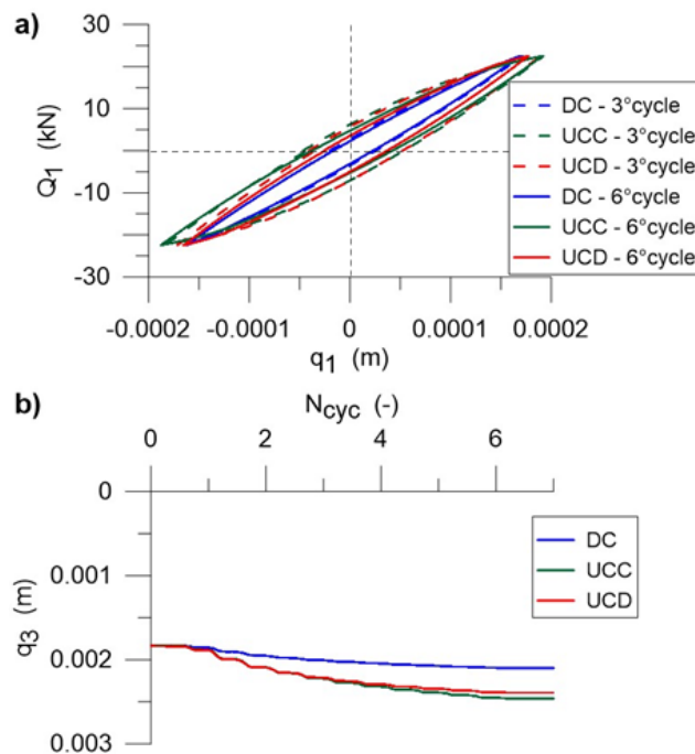
Figure 3. Comparison between the DC, UCC and UCD cases in terms of a) horizontal force-deformation relationship of the foundation in correspondence of the 3 rd and 6 th cycle, and b) time history of the vertical displacement for sequence T1.
