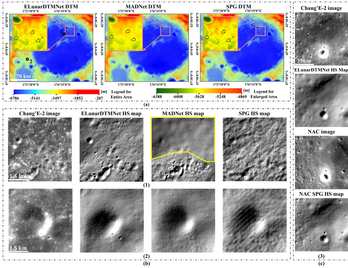
Fig. 15. Reconstructed DTMs of the Von Kármán Crater area using the Chang'E-2 imagery. (a) DTMs reconstructed by the proposed ELunarDTMNet with a resolution of 7 m, MADNet with a resolution of 14 m, and SPG method [46] with a resolution of 20 m. (b) Chang'E-2 imagery, and the HS maps derived from ELunarDTMNet, MADNet, and SPG method in local areas 1 and 2. The yellow arrows point to some craters where MADNet exhibits discrepancies compared to both SPG and our methods. The irregular yellow polygon indicates the areas identified by MADNet as oversmoothed. The black boxes in (a) indicate the locations of local areas. (c) Chang'E-2 imagery and the corresponding HS map generated by the proposed ELunarDTMNet, along with the NAC image and the HS map derived from the SPG method based on NAC images in local area 3.
