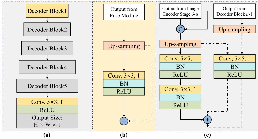
Fig. 6. Architecture of the decoder module. (a) Illustration of the overall structure. (b) Details of decoder block1. (c) Details of subsequent decoder blocks, where u ranges from 2 to 5. The dash-dotted line in (c) represents the residual connection fashion of UPB, while the dashed line represents the residual connection fashion proposed in this study. “C” represents the concatenation operation. “+” represents the addition operation.
