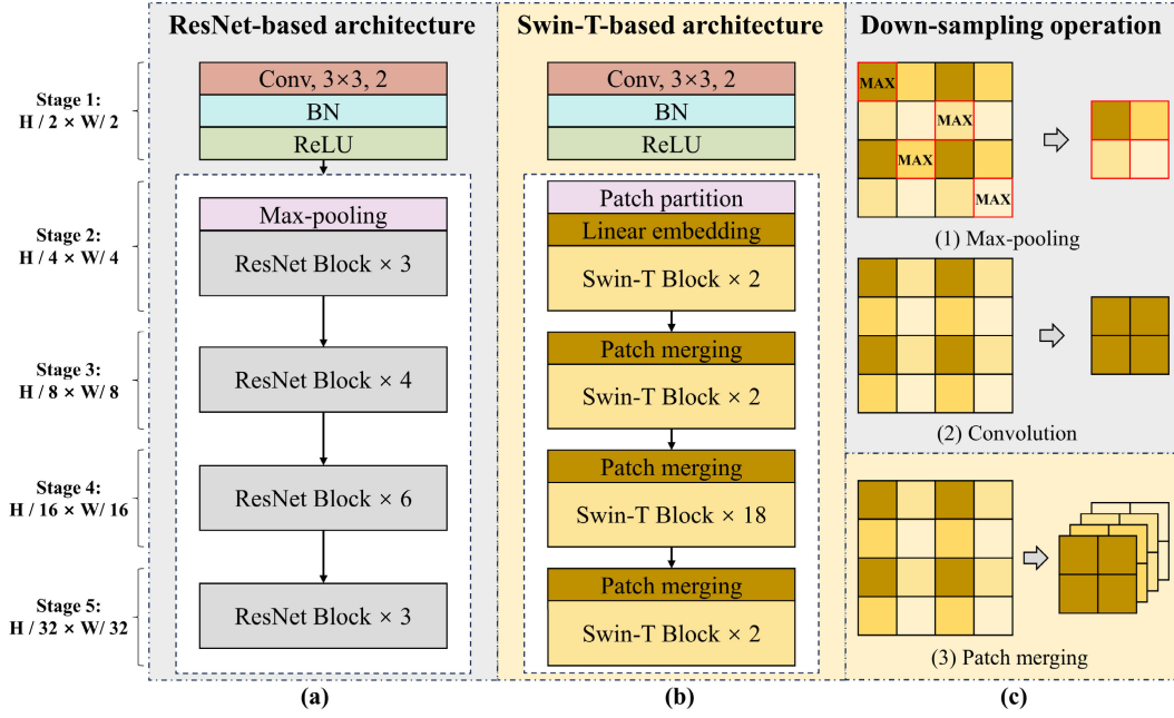
Fig. 4. Architecture of the encoder branch for extracting multiscale features from high-resolution optical images captured from an orbiter. (a) ResNet-based architecture from DLunarDTMNet, (b) Swin-T-based architecture introduced in this article, and (c) spatial dimension reduction methods of ResNet using (1) max-pooling, (2) convolution with a stride of 2 operations, while (3) Swin-T using patch merging. The values depicted on the left side indicate the output size of each stage. Conv: convolution operation, BN: batch normalization, ReLU: an activation function.
