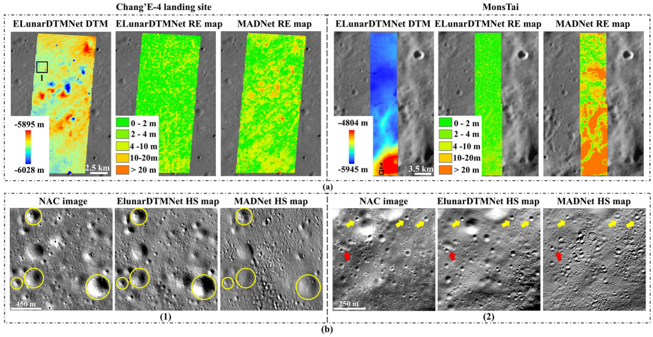
Fig. 12. Reconstructed DTMs using the proposed ELunarDTMNet and their performance comparison with the MADNet in the Chang'E-4 landing site and MonsTai areas. (a) DTMs generated by ELunarDTMNet, and the RE maps generated by ELunarDTMNet and MADNet. (b) NAC images, and the HS maps derived from ELunarDTMNet and MADNet on the local areas. The SPG DTM [7] in the Chang'E-4 landing site area and the SLDEM [41] in the MonsTai area are used as the reference DTMs to determine the RE maps. The results from MADNet have been coaligned to the SPG DTM (SLDEM) in this study. The black boxes in (a) indicate the locations of the local areas. The yellow circles and arrows indicate some craters that MADNet struggles to accurately predict. The red arrows point to an irregularly shaped feature that MADNet fails to reconstruct.
