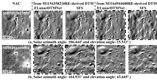
Fig. 14. Cross-illumination verification for the proposed ELunarDTMNet and the SFS method [8] centered at (19.60°W, 44.43°N). (a) M1154358210RE. (b) M1164944600RE. From left to right, the figures show the NAC images, the proposed ELunarDTMNet (second and fourth columns), and the SFS (third and fifth columns) results from M1154358210RE-derived and M1164944600RE-derived DTMs. The HS maps in columns two through five are generated using the same illumination conditions as the left NAC images. Bolded borders on the maps indicate that the corresponding DTMs are generated from another NAC image.
