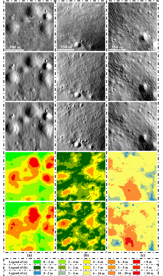
Fig. 19. Performance comparison using our proposed mean-normalized loss and l1 loss in three local areas. Areas (a) centered at (23.46^\circ, 0.66^\circ) , (b) centered at (292.48^\circ, 32.04^\circ) , and (c) centered at (167.24^\circ, 42.13^\circ) . From top to bottom, the images show the NAC images, the HS maps using the mean-normalized and the l1 losses, and the RE maps using the mean-normalized and the l1 losses.
