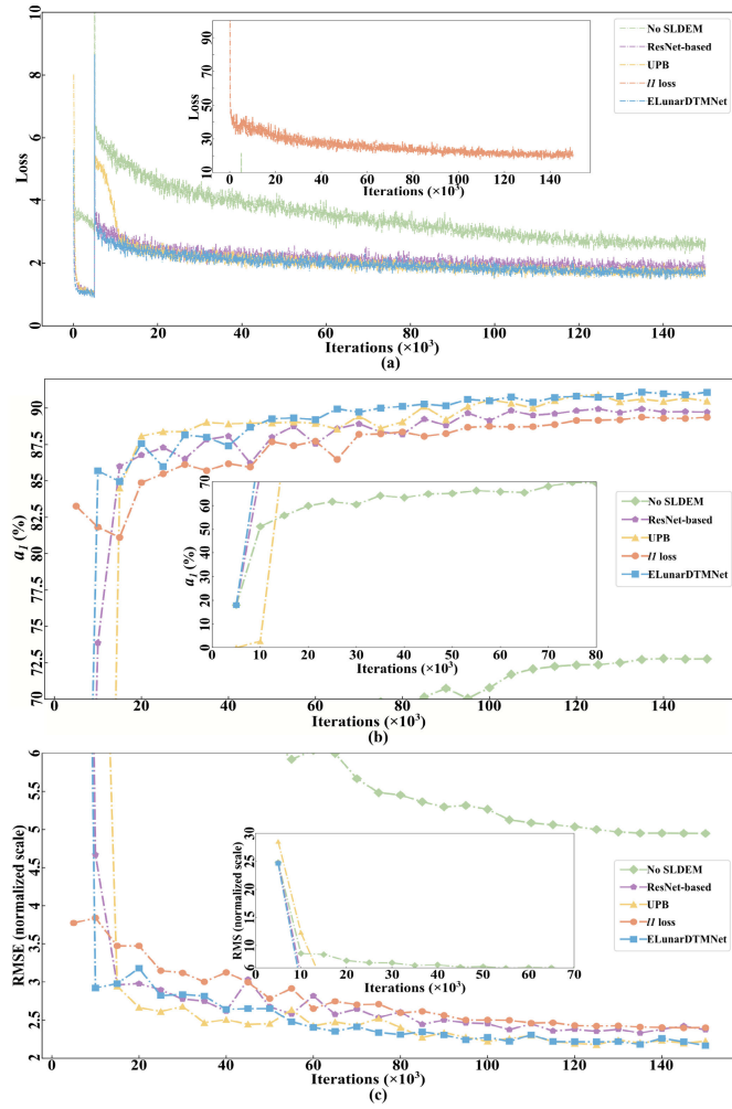
Fig. 16. Training and validation logs of the ablation study based on our proposed DTM normalization strategy. (a) Training curves. (b) and (c) Metrics a_1 and RMSE on the validation set every 5 k iterations, respectively. “No SLDEM” indicates training the network without using SLDEM as input. “ResNet-based” indicates using ResNet-based instead of Swin-T-based backbone to extract features from images. “UPB” indicates using UPB instead of our proposed residual-connected mechanism to construct the decoder module. “ l_1 loss” indicates using l_1 loss instead of our proposed mean-normalized loss function to train the network. “ELunarDTMNet” represents using our proposed method to train the network. The max-min DTM normalization strategy is not compared in this context as it uses a different normalization range, resulting in inconsistent metric scales.
