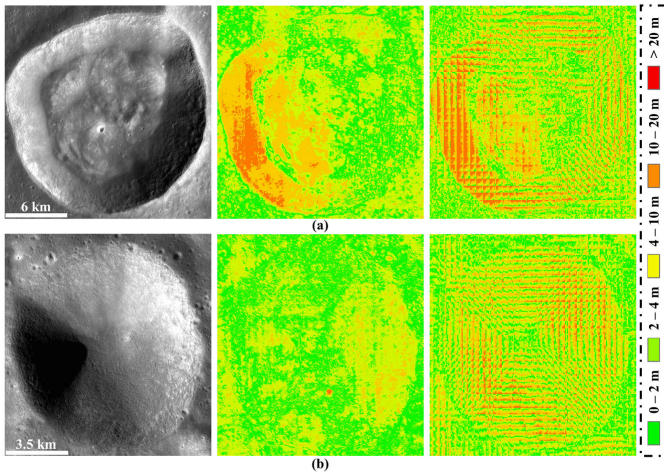
Fig. 20. Accuracy analysis for the large bright slopes in the Lichtenberg (a) and Hponds (b) regions. From left to right, the images show the NAC image, the RE map between our DTM and SPG DTM, and the RE map between SLDEM and SPG DTM.
