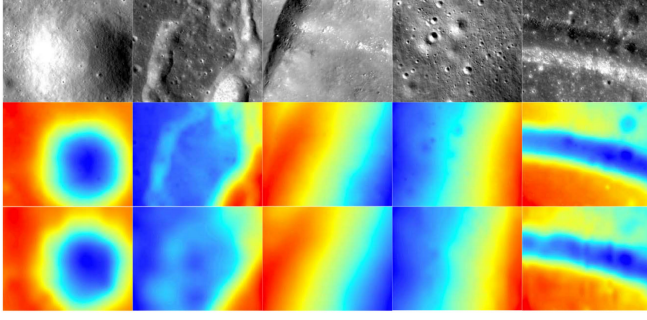
Fig. 9. Examples of the small-sized samples: top panel is the NAC ORIs, middle panel is the SPG NAC DTMs, and bottom panel is the corresponding SLDEM.
