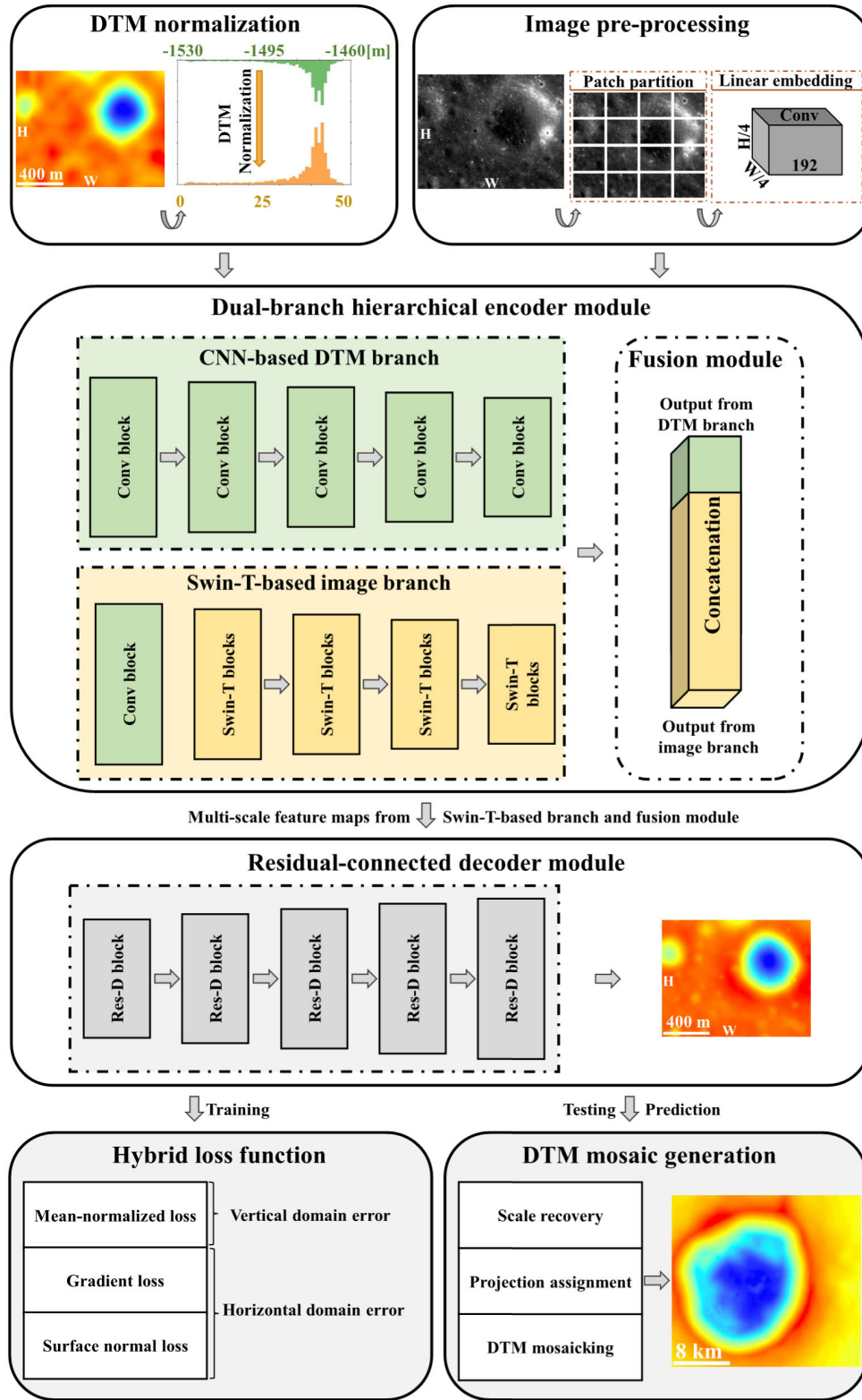
Fig. 2. Framework of our proposed ELunarDTMNet for pixel-level resolution DTM reconstruction. The CNN-based DTM branch is designed to process input DTMs, while the Swin-T-based image branch is designed to process input images. Swin-T: Swin Transformer, Res-D: Residual-connected decoder, H: image height, W: image width.
