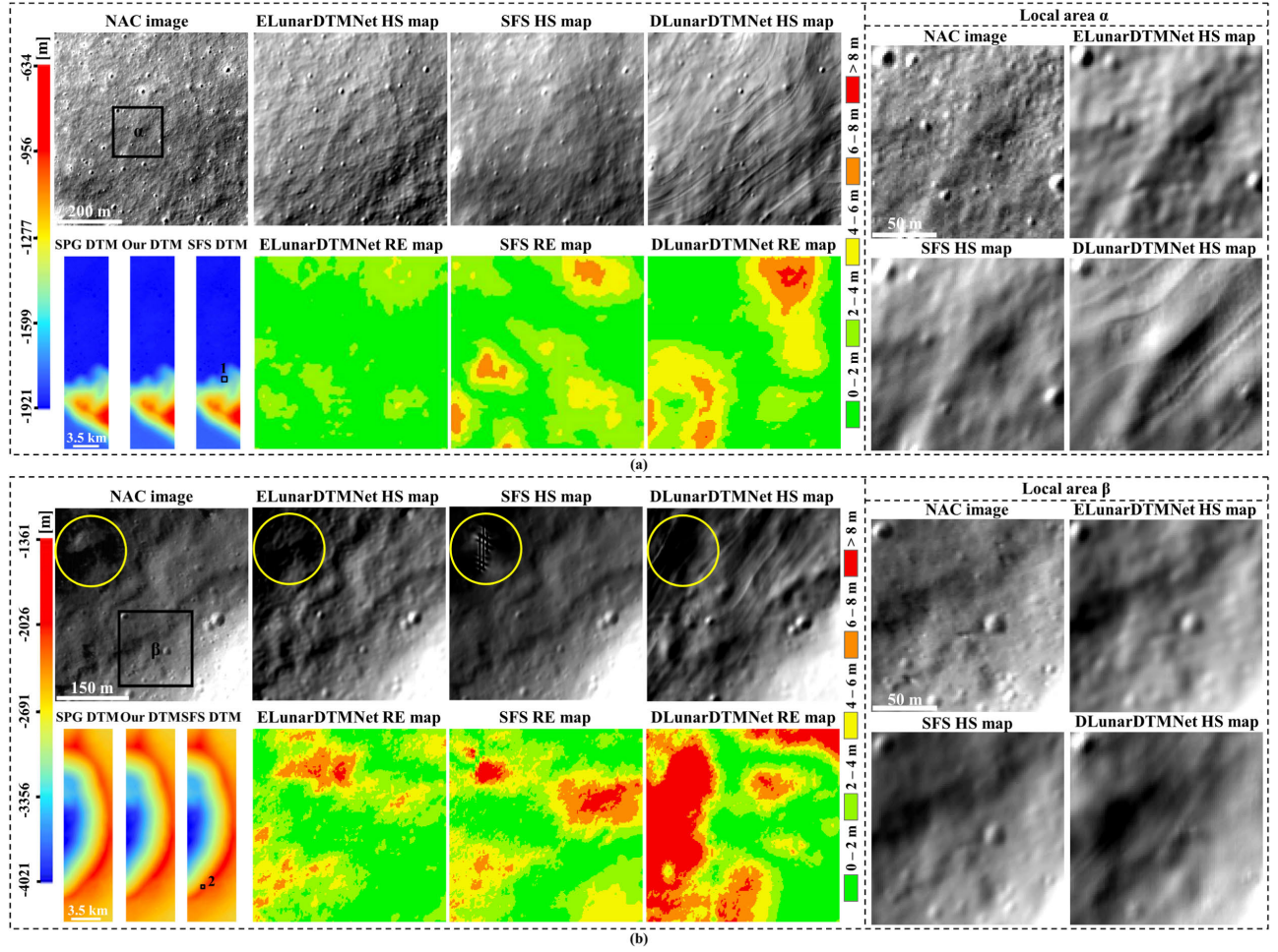
Fig. 13. Reconstructed DTMs by the proposed ELunarDTMNet and the SFS method [8], with comparisons of local areas using HS maps and RE maps. (a) Imbrium region. (b) Lichtenberg region. The black boxes 1 and 2 on the SFS DTMs mark the locations of the local areas shown in the left panels. The locations of further localized areas in the right panels are indicated by the black boxes labeled \alpha and \beta .
