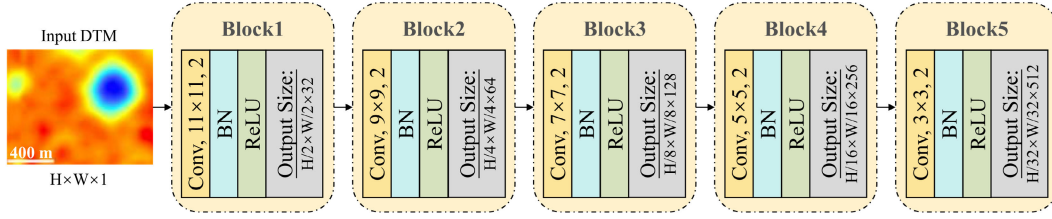
Fig. 5. Architecture of the encoder branch for extracting features from coarse-resolution DTMs.
