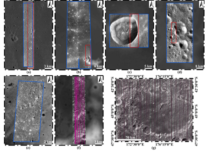
Fig. 10. NAC images of the test areas with the SLDEM as background. (a) Apollo 11 (M150361817LE, M150361817RE, and M150368601RE). (b) Imbrium (M1106095239LE, M1106095239RE, M183697099LE, and M183697099RE). (c) Lichtenberg (M191052644LE, M191052644RE, M191059794LE, and M191059794RE). (d) Hponds (M182432168LE, M182432168RE, M182439316LE, M182439316RE, and M182425021LE). (e) Chang'E-4 landing site (M1303619844 and M1303619844). (f) MonsTai (M123417906 and M123417906). The red boxes in (a)–(d) indicate the areas considered for comparing the performance of our method with the SFS method. (g) Chang'E-2 imagery for the Von Kármán Crater area. The blue polygons mark the regions of SPG DTMs for accuracy evaluation. The purple tracks in (f) and (g) indicate the LOLA tracks used for accuracy assessment due to the absence of publicly released or reliable SPG DTMs for reference.
