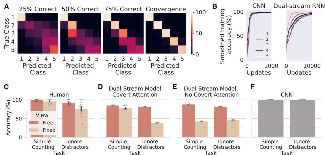
Figure 5. Comparisons with human behavior
