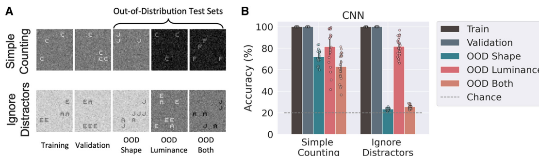
Figure 2. Task and baseline performance
