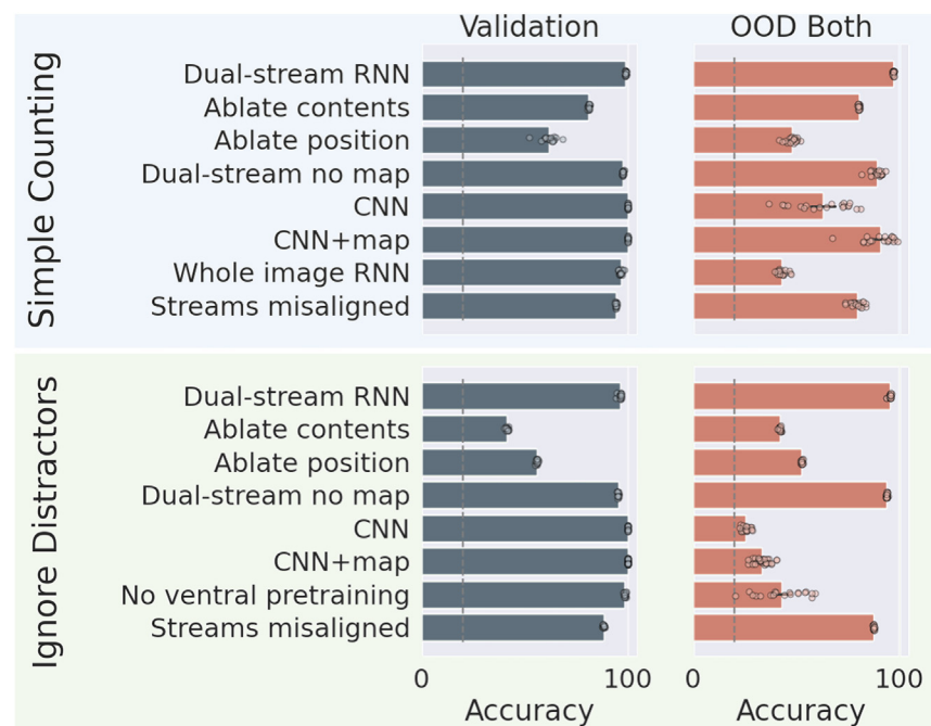
Figure 4. Ablations and control models
