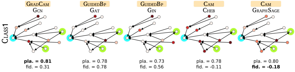
Fig. 17. Examples of explanations provided for each model by its highest plausibility explainer, when applied to a random node from INFECTION. Class 0 and class 2 are omitted, since their visualization does not provide significant insights. The plausibility and fidelity values are those of the entire dataset, as reported in Figure 16.
