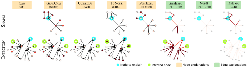
Fig. 12. Explanation masks (node- or edge-based) computed by the different explainers on the predictions of GRAPH-SAGE on SHAPES and INFECTION. Each row visualizes the mask computed for a given random graph from each dataset. For each dataset, only the explainers that passed the filtering procedure are shown.
