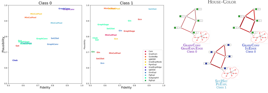
Fig. 10. Left: Fidelity and plausibility achieved by all the model-explainer pairs when applied to HOUSE-COLOR, where the two classes (0 and 1) are represented in the left and right panel. In each pair the name refers to the model, while the color identifies the explainer. The plot is limited to metrics larger than 0.5 to simplify the visualization. Right: stability of the explanations for the three top-performing model-explanation pairs. The colors identify important edges (dark red), and the edge thickness the variability of the importance in the dataset.
