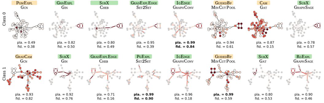
Fig. 11. Examples of explanations provided for each model and its highest plausibility explainer, when applied to a random sample from GRID-HOUSE. Each row shows the results for one of the two classes. The plausibility and fidelity values are those of the entire dataset, as reported in the right of Figure 10.
