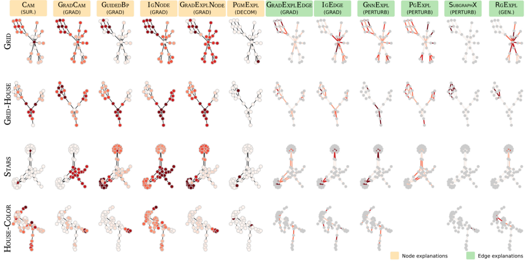
Fig. 1. Explanation masks (node- or edge-based) computed by the different explainers on the predictions of GCN. Each row visualizes the mask computed for a given random graph from each dataset.
