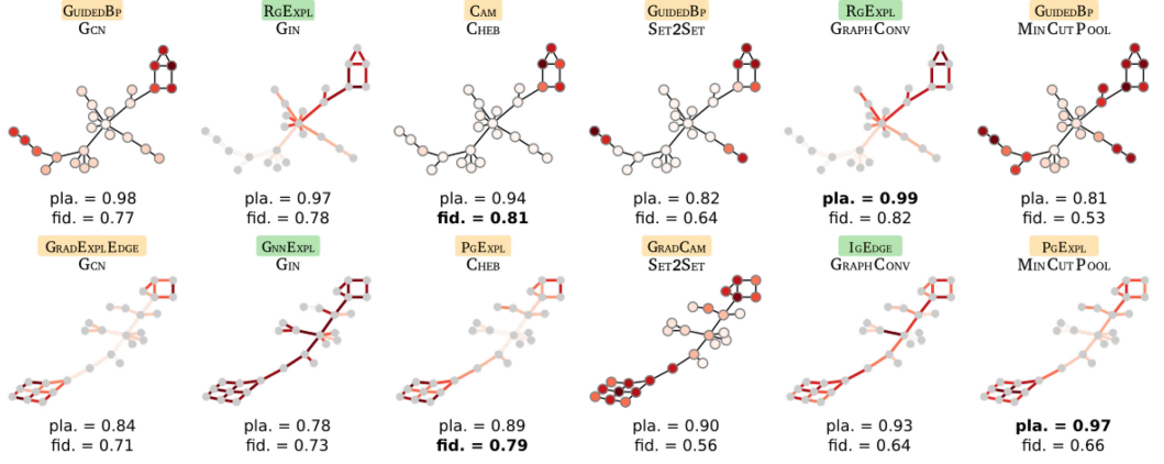
Fig. 6. Examples of explanations provided for each model and its highest plausibility explainer, when applied to a random sample from GRID-HOUSE. Each row shows the results for one of the two classes. The plausibility and fidelity values are those of the entire dataset, as reported in Figure 5.
