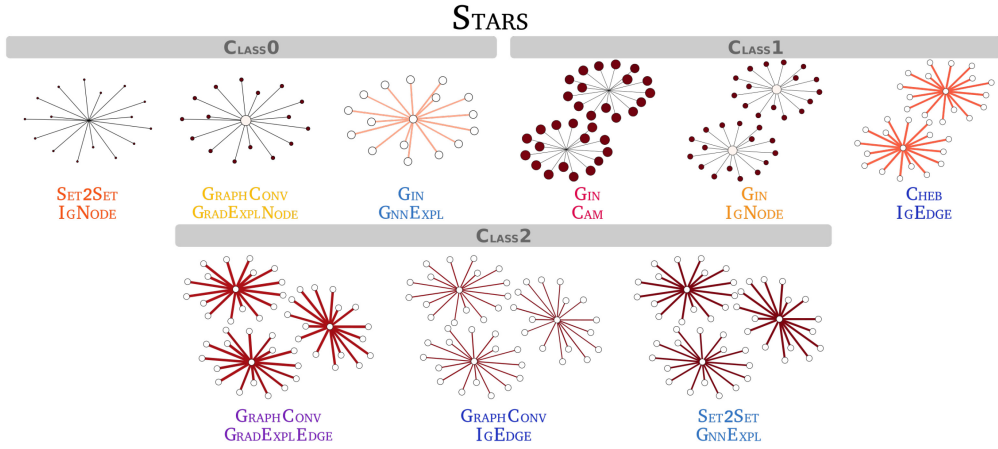
Fig. 8. Stability of the explanations for the three top-performing model-explanation pairs for each of the three classes. The colors identify important edges (dark red) and the edge thickness the variability of the importance in the dataset.
