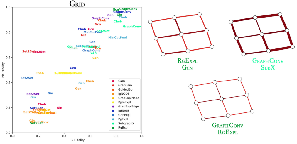
Fig. 3. Left: Fidelity and plausibility achieved by all the model–explainer pairs when applied to GRID. In each pair, the name refers to the model while the color identifies the explainer. Right: Stability of the explanations for the three top-performing model–explanation pairs. The colors identify important edges (dark red), and the edge thickness the variability of the importance in the dataset.
