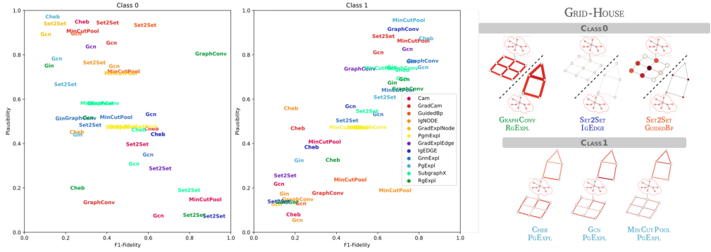
Fig. 5. Left: Fidelity and plausibility achieved by all the model-explainer pairs when applied to GRID-HOUSE, for class 0 (left) and class 1 (right). In each pair the name refers to the model, while the color identifies the explainer. Right: Stability of the explanations for the three top-performing model-explanation pairs, for each of the two classes. The colors identify important edges (dark red), and the edge thickness the variability of the importance in the dataset.
