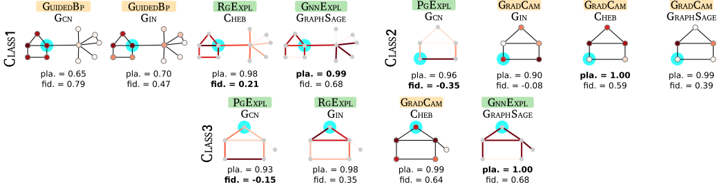
Fig. 15. Examples of explanations provided for each model by its highest plausibility explainer, when applied to a random node from SHAPES. Each row shows the results for one of the three house-structure classes. The plausibility and fidelity values are those of the entire dataset, as reported in Figure 14.
