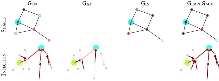
Fig. 13. Explanation masks (node- or edge-based) computed on the predictions of GNNExPL by the different explainers both on SHAPES and INFECTION. Each row visualizes the mask computed for a given random graph from each dataset. For each dataset, only the explainers that passed the filtering procedure are shown.
