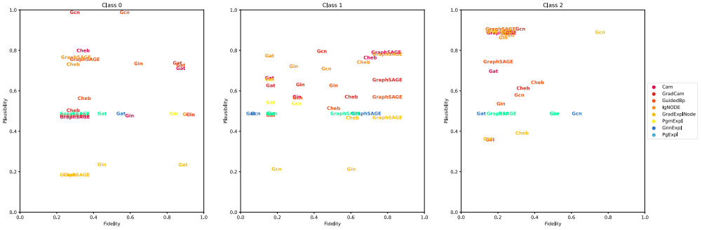
Fig. 16. Fidelity and plausibility achieved by all the model-explainer pairs when applied to INFECTION. In each pair the name refers to the model, while the color identifies the explainer.
