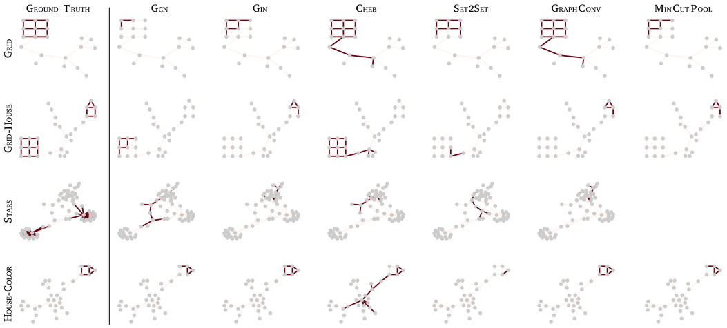
Fig. 2. Explanation masks computed by SUBX on the predictions of the different models. Each row visualizes the mask computed for a given random graph from each dataset.
