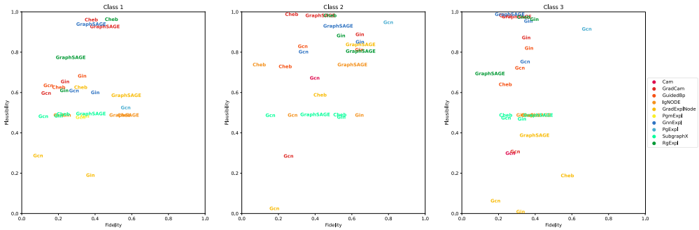
Fig. 14. Fidelity and plausibility achieved by all the model-explainer pairs when applied to SHAPES. In each pair the name refers to the model, while the color identifies the explainer. Class 0 is omitted from the visualization, since it is less relevant for the discussion of the explainers.
