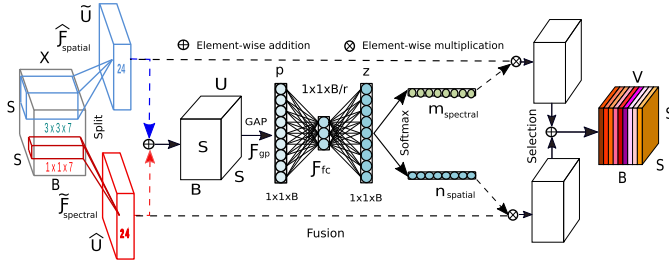
Fig. 2. Adaptive spectral-spatial kernel attention module.
