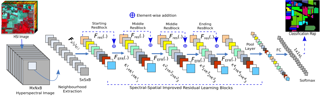
Fig. 1. Framework of the proposed network for HSI classification. Given a raw 3-D input patch of size S \times S \times B , where B is the number of spectral bands, the input is first passed through \mathcal{F}_{A^2S^2K}(\cdot) to learn the selection of spectral-spatial kernel among different RFs. Then, discriminative features are extracted through F_{res}(\cdot) and recalibrated through the spectral-spatial channel attention \mathcal{F}_{EFR}(\cdot) . Finally, the classification is performed using the softmax layer.
