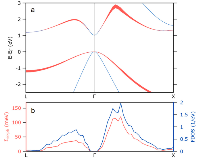
Fig. 7. Panel a ): wannierized GaAs band structure starting from a LDA calculation. Here, the linewidth associated to the highest valence and lowest conduction band eigenvalues is two times the imaginary part of the associated electron-phonon self energy \Sigma_{el-ph} on a high-symmetry path of the FCC BZ. Panel b ): \mathbf{k} -resolved electron-phonon self energy \Sigma_{el-ph} and final-state density of states (FDOS, Eq. (49)) for the lowest conduction band along the same path of panel a ).
