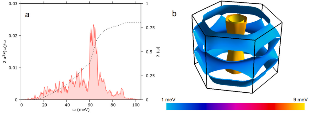
Fig. 2. Superconducting properties of \text{MgB}_2 . Left panel: frequency-resolved Eliashberg function and electron-phonon coupling parameter \lambda . Right panel: Fermi surface resolved Migdal-Eliashberg gap ( T = 10 K). (For interpretation of the colors in the figure(s), the reader is referred to the web version of this article.)
