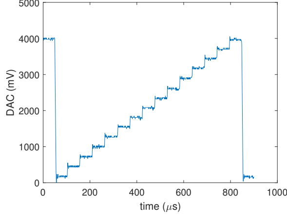
Figure 5.2: DAC output voltage, when driven by Arduino running the phase correction code 1 in the absence of any input. New outputs are provided every 55\mu s approximately, thus at 18k bps , and the maximum output voltage at the DAC is \sim 4V . The value of the voltage steps shown is a consequence of the proportional constant ( k_p ) set.
