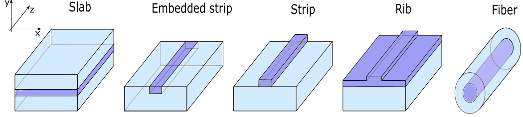
Figure 2.9: Waveguide geometries, with the darker blue region representing the core of the waveguide where light propagates.
