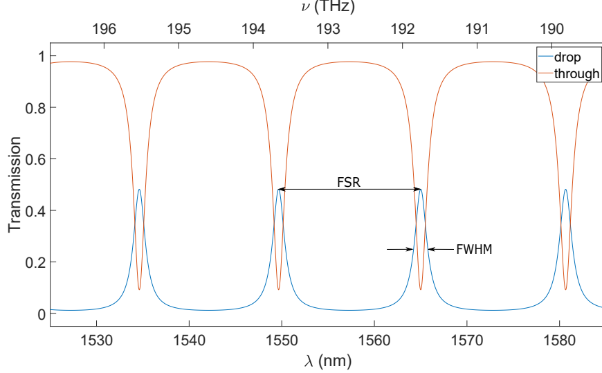
Figure 3.2: Through and drop transmissions of a microring resonator in add-drop filter configuration, having radius r = 6.75\mu m , k^2 = 0.2 and a_{rt} = 0.9 .
