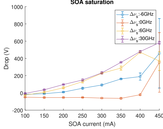
Figure 6.5: Response of a virtual node sampled at 273\text{ns} as a function of the SOA current, for different starting detuning values.
