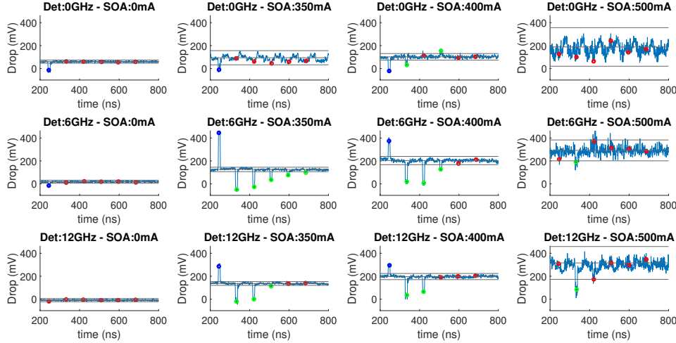
Figure 5.9: Drop response to a 10ns input pulse, acquired at \Delta\phi_F = \pi/3 and for various detuning (rows) and feedback strength \eta_F (SOA current) (columns). The first column represents the system response in absence of a feedback signal (zero SOA current). An increase in the SOA current allows a larger number of delayed copies (echoes) in the microring with external feedback. The blue dots indicate the drop copy that follows the input one, while the green dots refer to the copies via the feedback loop. The red dots indicate the delayed copies that are not counted by the algorithm.
