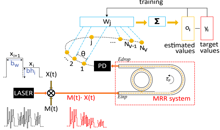
Figure 4.7: Schematic of time delay RC with an MRR subject to optical feedback. The encoded information X(t) is masked with a sequence M(t) and modulates the optical power from the laser (LAS) emission. At the drop port, the photodetected (PD) signal provides the time-multiplexed output states of the reservoir, which are weighted and linearly combined to compute the predicted value o_i . The weight optimization is performed via a linear classifier, with supervised learning over the expected values y_i data set.
