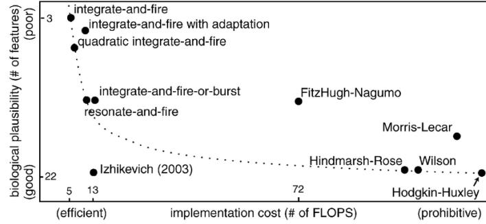
Figure 2.7: Trade-off between biological plausibility and implementation cost in FLOPS per 1ms of simulation time, for several mathematical and biophysical models. Taken from [20].
