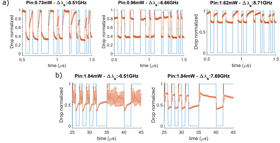
Figure 6.14: Example of experimental traces acquired at an input bit rate of a) 40Mbps and b) 1Mbps, for specific configurations (P_{in}, \Delta\nu_s) indicated on top of each panel. These configurations refer to the red dots in Fig. 6.13. The modulation amplitude is 0.5.
