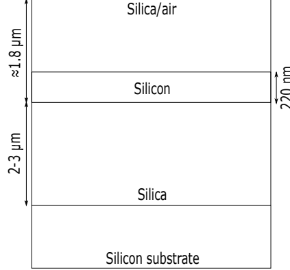
Figure 2.8: Illustration of an SOI wafer cross-section with typical dimensions, having a silicon core and silica cladding and substrate. Also air, for example, can serve as a cladding. The bottom silicon layer is used as substrate of the structure while the optical components are built in the top silicon layer.
