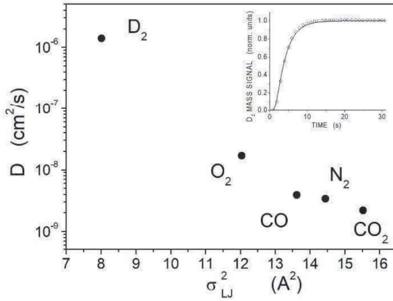
Fig. SI4: Plot of the diffusivity value of the examined penetrants in Matrimid® obtained at T = 300 \pm K as a function of the squared Lennard-Jones molecular size ( \sigma_{LJ} values are reported in Table II). The deuterium ( D_2 ) diffusivity value is also reported. This value was evaluated fitting by eq. 5 a normalized D_2 permeation curve obtained at T = 300 \pm 2 K and feed pressure of 40 kPa (see inset).
