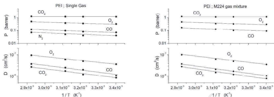
Fig. 6: Arrhenius plot of the gas permeability ( P ) and diffusivity ( D ) of the PEI membrane sample as obtained in single gas permeation (left panel) and with the ternary M224 gas mixture (right panel). Numerical values are reported in the Supplementary Information section. N_2 diffusivity values measured in Single Gas conditions (left panel) are not reported as overlap with CO diffusivity values. Permeation tests were carried out with feed pressure between 20 and 90 kPa.
