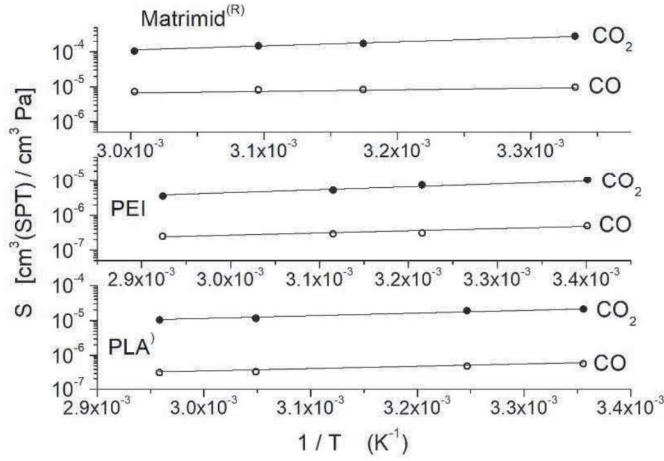
Fig. 8: Arrhenius plot of the gas solubility ( S ) of the Matrimid ® , PEI and PLA membrane film in single gas permeation tests obtained using P and D data in the left panels of figs. 4-6 by the relation S = P/D . Numerical values are reported in the Supplementary Information section. Permeation tests were carried out with feed pressure between 20 and 90 kPa.
