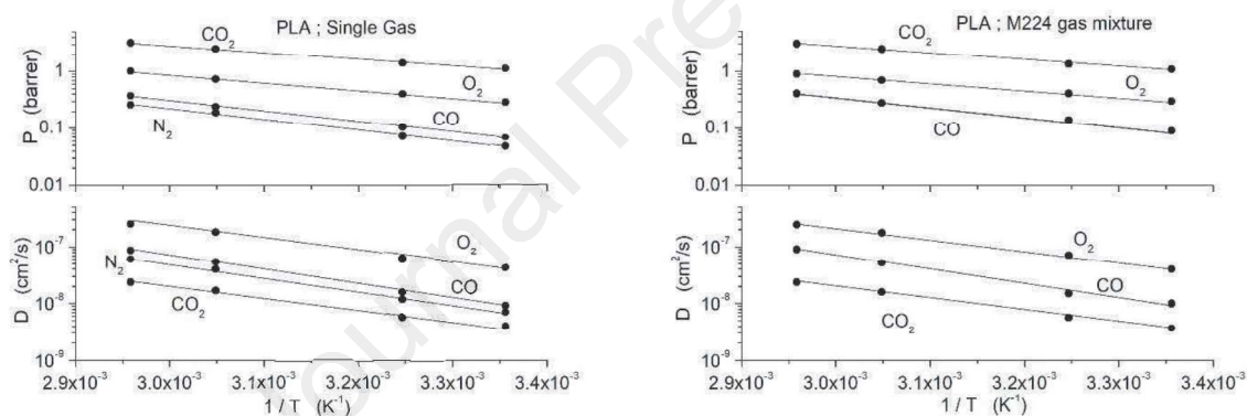
Fig. 7: Arrhenius plot of the gas permeability ( P ) and diffusivity ( D ) of the PLA membrane film as obtained in single gas permeation tests (left panel) and with the ternary M224 gas mixture (right panel). Numerical values are reported in the Supplementary Information section. Permeation tests were carried out with feed pressure between 20 and 90 kPa.
