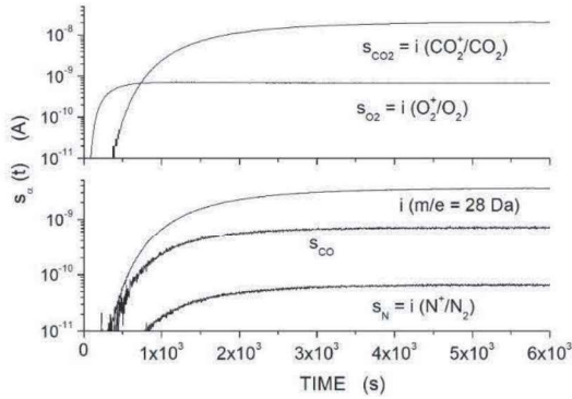
Fig. S13: s_{\alpha}(t) mass signals obtained at T = 300 \pm 2 K with the Matrimid® film sample exposed to the M225 gas mixture ( p_{feed} = 72 \pm 1 kPa).
