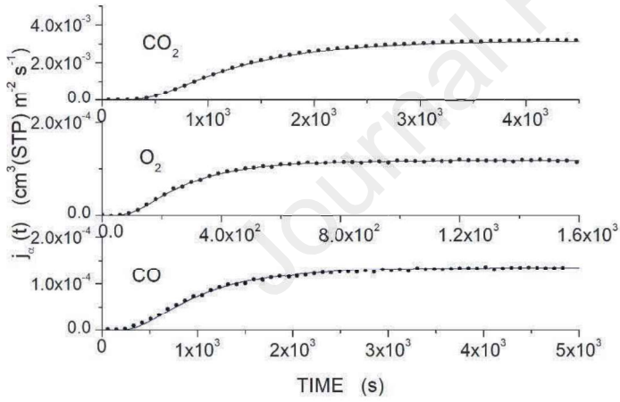
Fig. 2: j_{\alpha}(t) permeation curves obtained with the PEI membrane samples exposed to the M224 gas mixture ( p_{feed} = 45 \pm 1 kPa) at T = 295 \pm 2 K. Curves were calculated converting sampled s_{\alpha}(t) data of fig. S12 by eq. 2.
