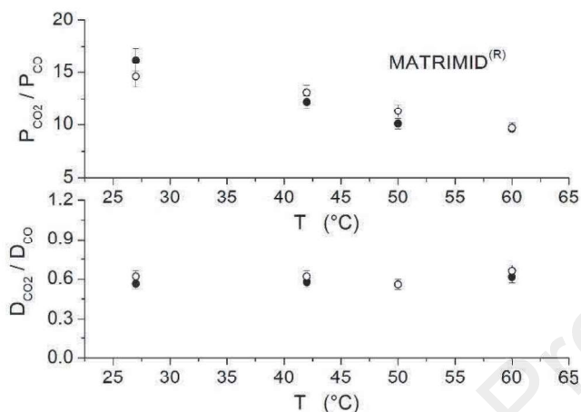
Fig. 9: Matrimid® membrane. Upper panel: CO_2/CO selectivity as a function of temperature. Lower panel: diffusivity ratio D_{CO_2}/D_{CO} as a function of temperature. Solid symbols: single gas tests. Open symbols: M224.
