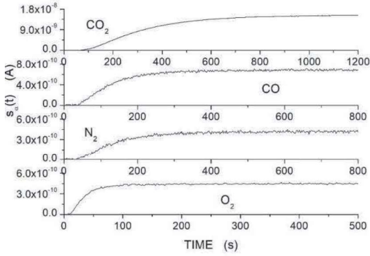
Fig. S11: s_{\alpha}(t) mass signals obtained at T = 298 \pm 2 K with the PLA film sample exposed to pure CO_2 , CO and N_2 gases ( p_{feed} = 45 \pm 1 kPa) and to the dry N_2/O_2 air mixture ( p_{feed} = 72 \pm 1 kPa).
