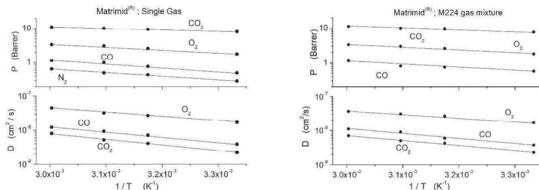
Fig. 5: Arrhenius plot of the gas permeability ( P ) and diffusivity ( D ) of the Matrimid ® membrane sample as obtained in single gas permeation tests (left panel) and with the ternary M224 gas mixture (right panel). Numerical values are reported in the Supplementary Information section. N_2 diffusivity values measured in Single Gas conditions (left panel) are not reported as overlap with CO diffusivity values. Permeation tests were carried out with feed pressure between 20 and 90 kPa.
