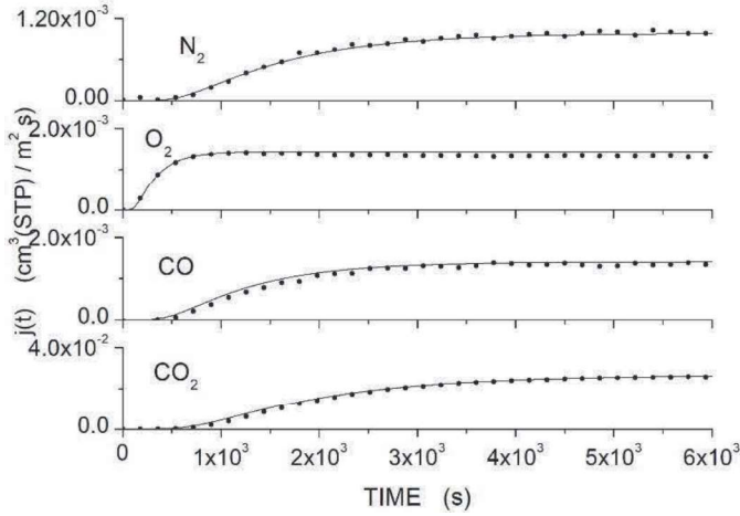
Fig. 3: j_{\alpha}(t) permeation curves obtained with the Matrimid® membrane samples exposed to the M225 gas mixture ( p_{feed} = 72 \pm 1 kPa) at T = 300 \pm 2 K. Curves were calculated converting sampled s_{\alpha}(t) data of fig. S13 by eq. 2.
