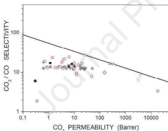
Fig. 12: CO_2/CO selectivity vs. CO_2 permeability. Continuous line refers to the proposed upper-bound correlation similar to the Robeson's plot curve [50,51]. Solid black circle and solid black squares refer to the Matrimid® and PEI films tested in the present study. Open black triangle: Matrimid® film [21]. Open black diamond: Ultem® film [32]. Crossed circles: polyimide films [44,45]. Open red circles: polyurethane-polycarbonate films [47]. Open blue squares: polyethylene films [42]. Open blue diamond: natural rubber [42]. Open blue triangles: polyether-polyamine films [49]. Open red square: poly(1-trimethylsilyl-propyne) film [48]. Open green triangle: polydimethyl siloxane films [48].
