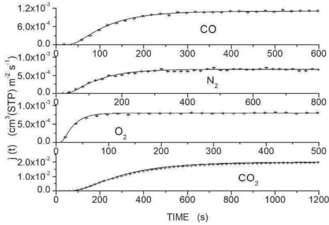
Fig. 1: j_{\alpha}(t) permeation curves obtained with the PLA membrane samples exposed to pure gases CO_2 , CO and N_2 gas ( p_{feed} = 45 \pm 1 kPa) and to the dry N_2/O_2 gas mixture ( p_{feed} = 72 \pm 1 kPa) at T = 298 \pm 2 K. Curves were calculated converting sampled s_{\alpha}(t) data of fig. S11 by eq. 2.
