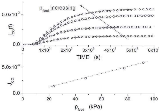
Fig. 4: Upper panel: j_{CO}(t) curves obtained at T = 300 K in single gas tests exposing the Matrimid® membrane sample to carbon monoxide at different feed pressure values [units: \text{cm}^3(\text{STP}) / \text{m}^2 \text{ s} ]. Lower panel: value of the j_{CO}(t) flux in stationary transport conditions ( J_{CO} ) as a function of the CO feed pressure [units of J_{CO} : \text{cm}^3(\text{STP}) / \text{m}^2 \text{ s} ].
