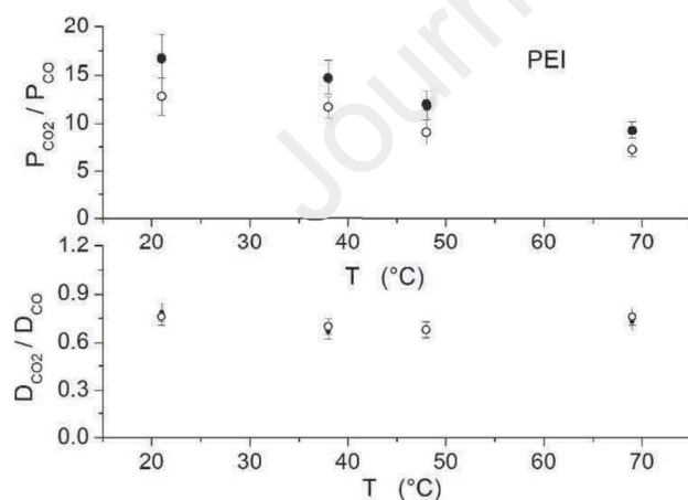
Fig. 10: PEI membrane. Upper panel: CO_2/CO selectivity as a function of temperature. Lower panel: diffusivity ratio D_{CO_2}/D_{CO} as a function of temperature. Solid symbols: single gas test. Open symbols: M224.
