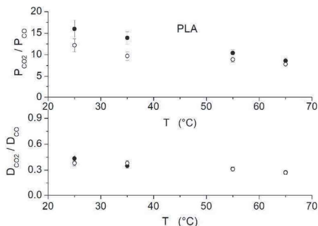
Fig. 11: PLA membrane. Upper panel: CO_2/CO selectivity as a function of temperature. Lower panel: diffusivity ratio D_{CO_2}/D_{CO} as a function of temperature. Solid symbols: single gas tests. Open symbols: M224.
