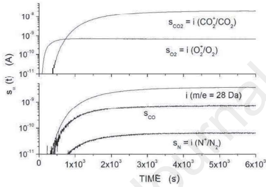
Fig. S12: s_{\alpha}(t) mass signals obtained at T = 295 \pm 2 K with the PEI film sample exposed to the M224 gas mixture ( p_{feed} = 45 \pm 1 kPa).
