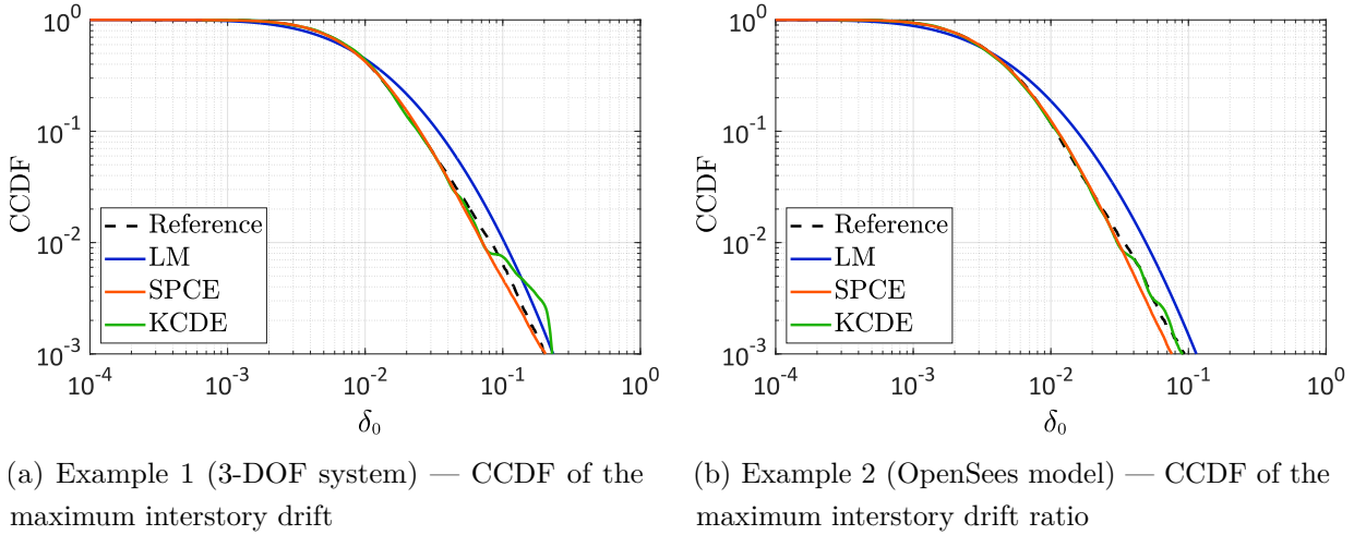
Figure 9: Comparisons of the CCDF estimation (the models are built on N = 1,000 ).
