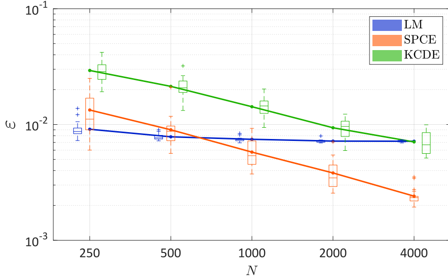
Figure 2: Example 1 — comparison of the convergence among the models in terms of the normalized Wasserstein distance. The lines correspond to the average values over 20 repetitions of the full analysis, whereas the box plot summarizes the 20 results.
