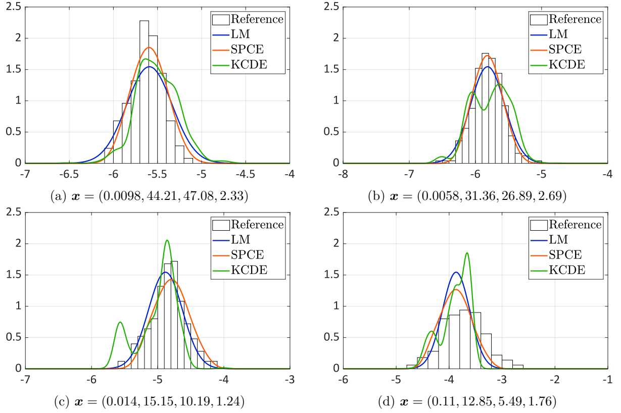
Figure 5: Example 2 — comparison of emulated PDFs of \log(Y_x) for four different values of x ; the models are built on N = 1,000 simulations.
