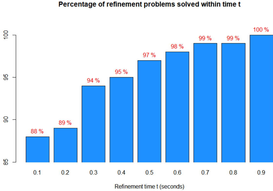
Figure 7.20: Percentage of problems solved within time t.
