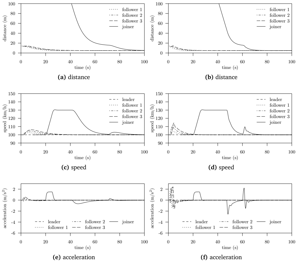
Figure 3.5 – Vehicle dynamics for the join maneuver. The left column shows the results for \xi = 1 , \omega_n = 0.2 Hz, while the right column for \xi = 2 , \omega_n = 1 Hz. Copyright © 2014 IEEE.
