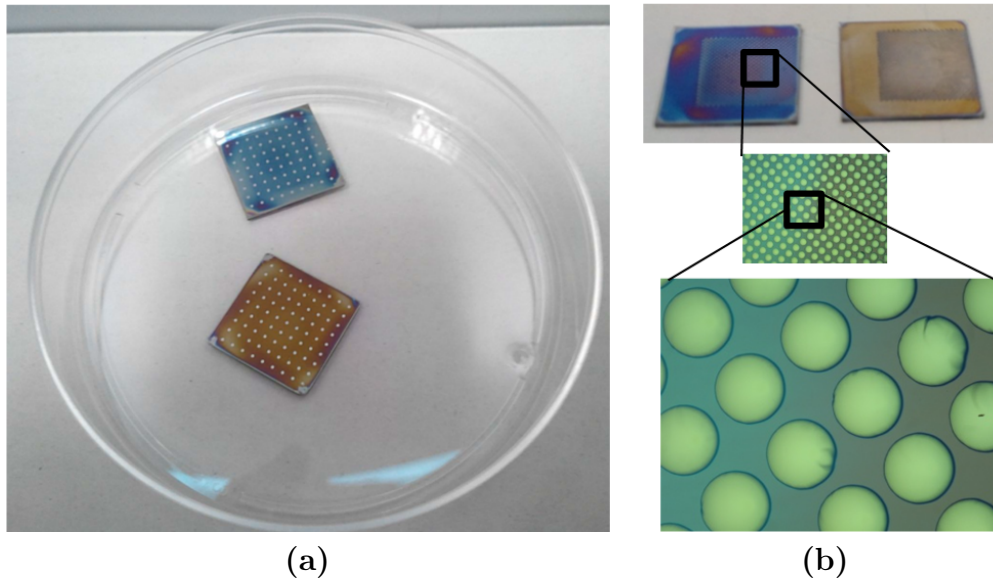
FIGURE 2.6: FBK memristor fabrication deposition techniques. (a) Aluminium dishes ( \sim 1\text{mm} of diameter) deposited on a one-layer and on a two-layer \text{TiO}_2 by Sol-gel. The area of the dices is 2\text{x}2\text{cm} . (b) , Platinum dish-shaped patterns ( \sim 0.35\text{ mm} of diameter) on a two layer \text{TiO}_2 Sol-gel dices.
