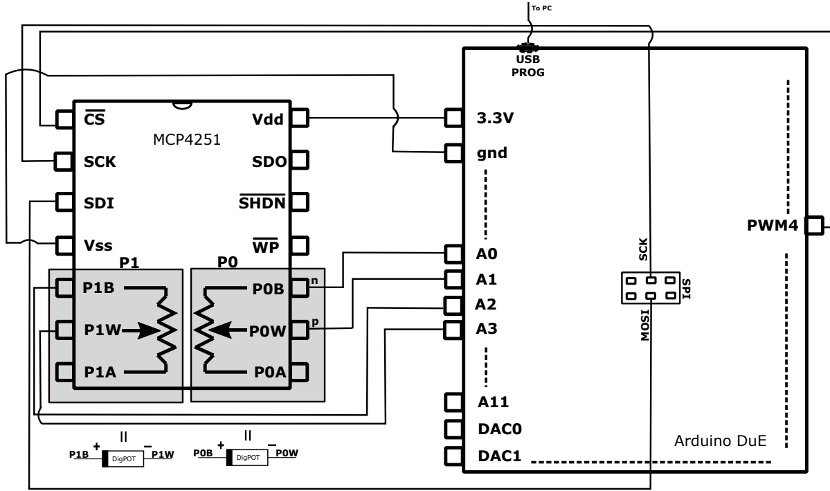
FIGURE 3.1: Pinout Schematic of the Arduino-controlled memristor emulator.
