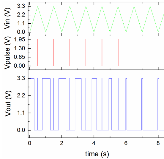
FIGURE A.4: Output of the memristor-based programmable threshold comparator with response to programming pulses applied to M_2 . The input signal V_{in} is a periodic triangular waveform.
