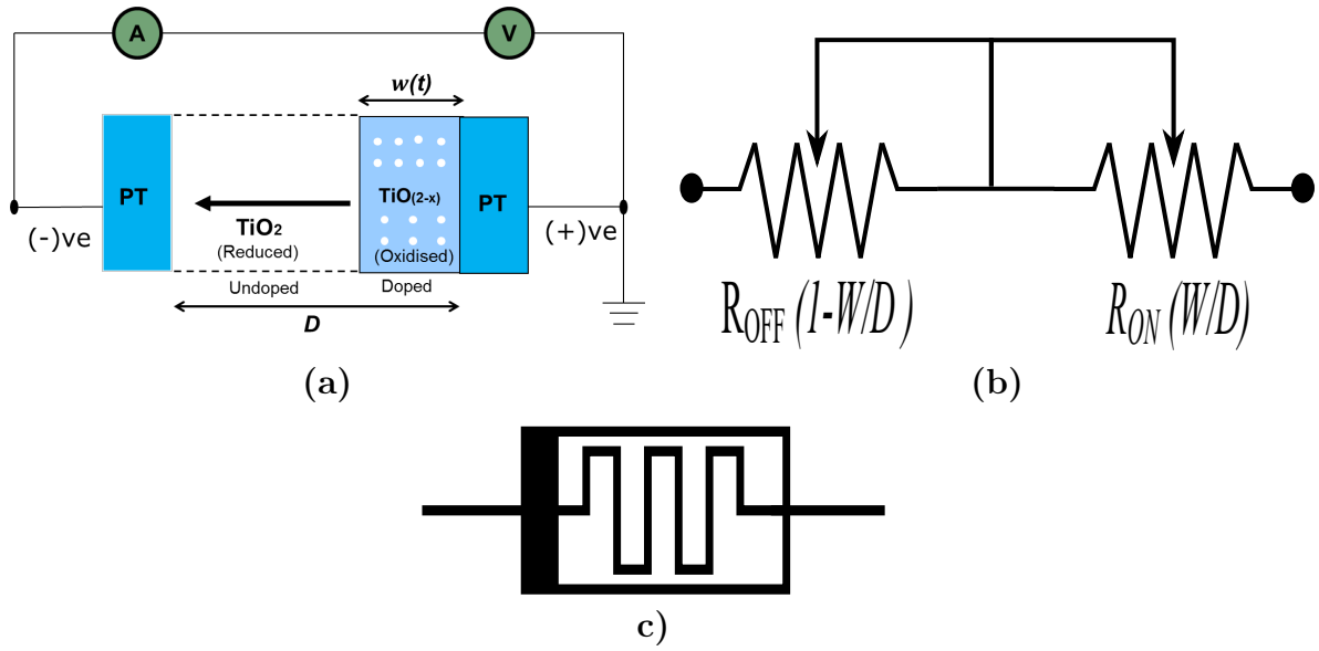
FIGURE 2.2: Diagram of the memristor with simplified equivalent circuit. (a) Cross-section of the memristor showing the Structure of the \text{TiO}_2 memristor consisting of a high conductive (doped) and a low conductive (undoped) layer sandwiched in between two platinum electrodes. The boundary between the two parts is dynamic and is moved back and forth as a function of the passing charge carriers. The parameter w(t) is state variable that describes the position of this boundary, (b) Equivalent resistor circuit, (c) Symbolic representation a memristor in an electric circuit
