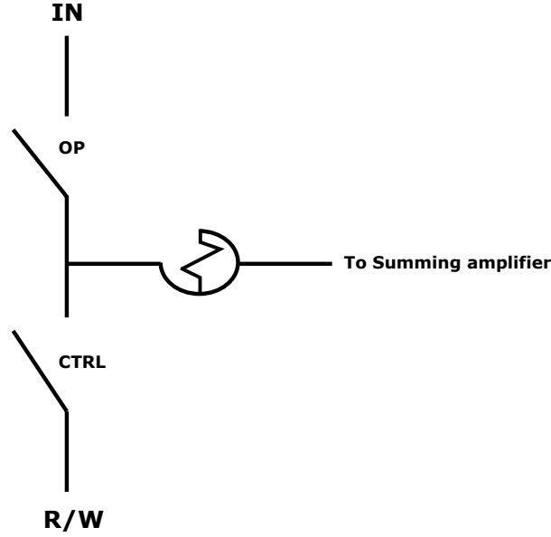
FIGURE D.3: Neuron Input Drivers: An illustration of how the memristor is connected to the CMOS switches
