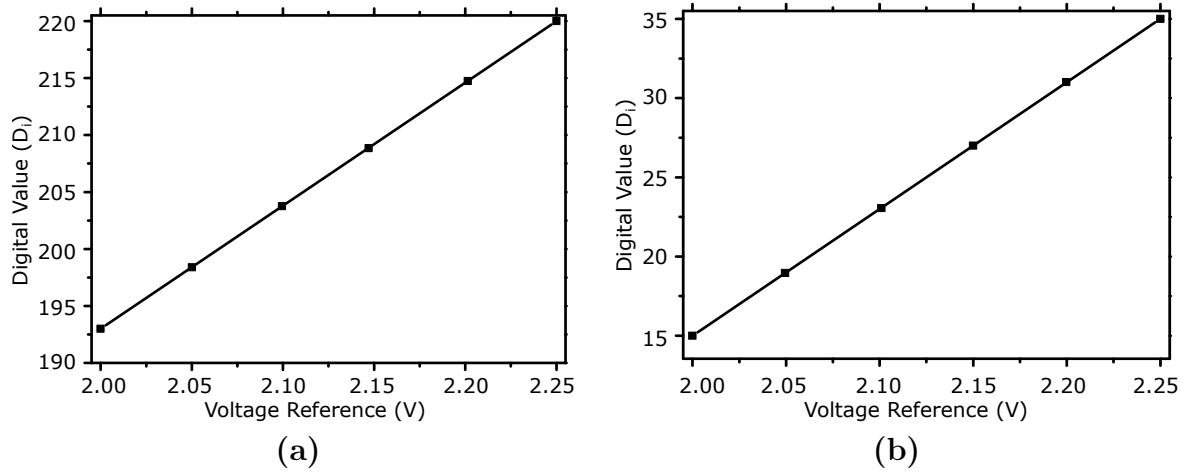
FIGURE 5.5: Digital output versus comparator threshold voltage V_{TH} . (a), Under low illumination for different voltage reference. (b), Under high illumination for different voltage reference.
