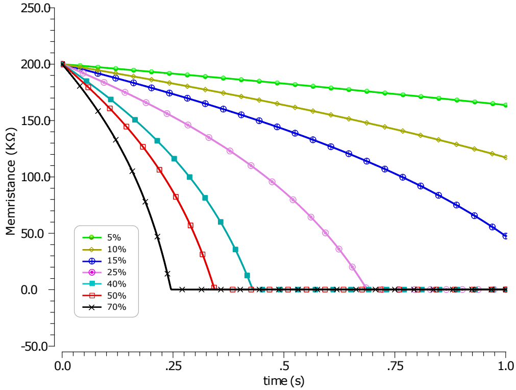
FIGURE 4.4: Memristance rate of change over time for different Duty cycles of a train of voltage pulses with amplitude v_p = 500\text{mV} and programming frequency \omega_p = 50\omega_0 .
