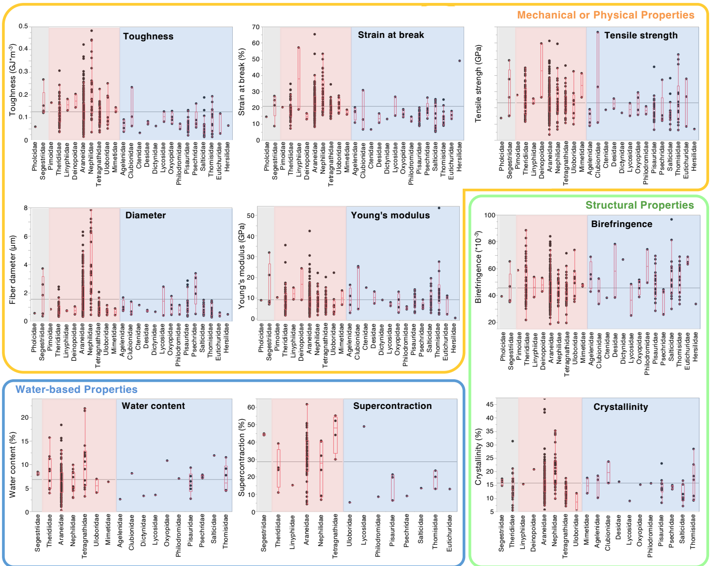
Supplementary Fig. 1 | Distribution of material properties of dragline silk fibers by family.
