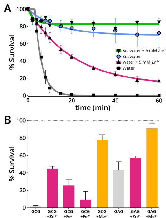
Figure 2. Survival of GCG upon heating in the presence of thiophilic metal ions. (A) GCG in the presence or absence of 5 mM \text{Zn}^{2+} in buffered water (20 mM glycylglycine at pH 8.7) or seawater (pH 8.0) conditions. (B) GCG (5 mM) or GAG (5 mM) in buffered water was heated at 150 °C for 20 min in the presence of 5 mM \text{Zn}^{2+} , \text{Fe}^{2+} , or \text{Fe}^{3+} (magenta) or 40 mM \text{Mg}^{2+} (yellow). Data are the mean \pm SD; n = 3 .
