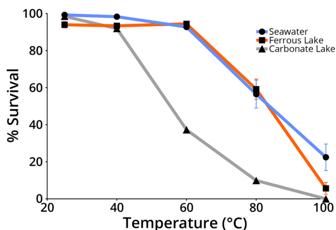
Figure 3. Survival of GCG in solutions mimicking prebiotic geological conditions (seawater, pH 8.0; carbonate lake, pH 9.0; and ferrous lake, pH 6.3). Solutions were heated in a sealed glass vial for 24 h. Data are the mean \pm SD; n = 3 .
