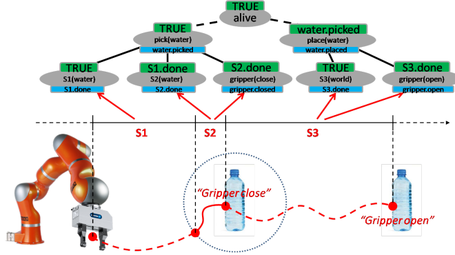
Fig. 2. A representation of the action segmentation during a pick and place task. The RBM (down) performs the action segmentation, while the attentional system (up) connects these segments to the task structure.
