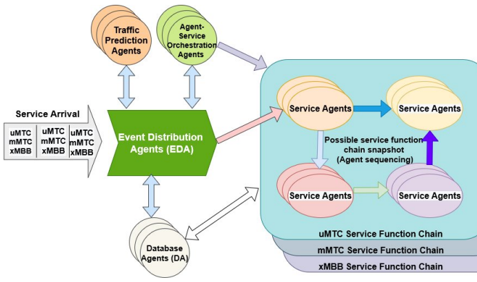
Fig. 10. Agent Sequencing and Scheduling for Arrival Service Processing
