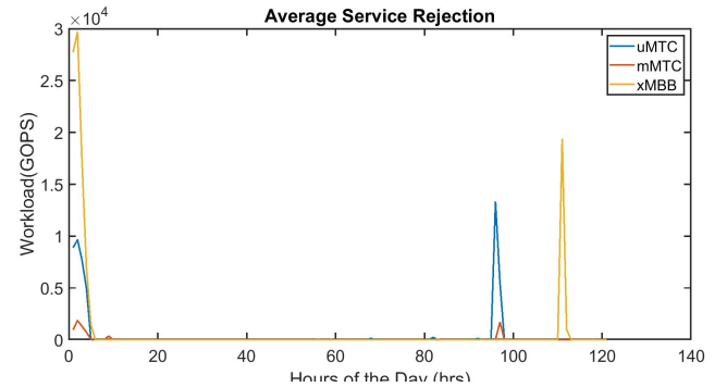
Fig. 29. Service Rejection with Backup Service Processing Agents
