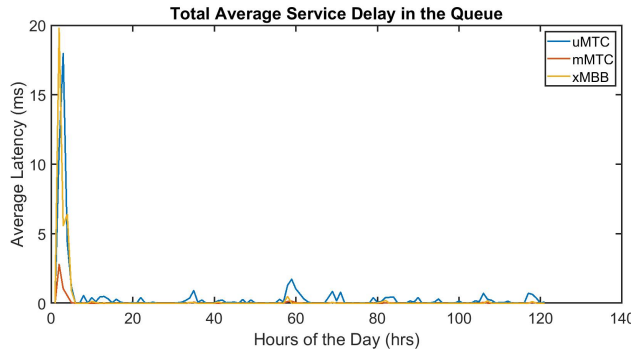
Fig. 23. Arrival Service Queuing Delay
