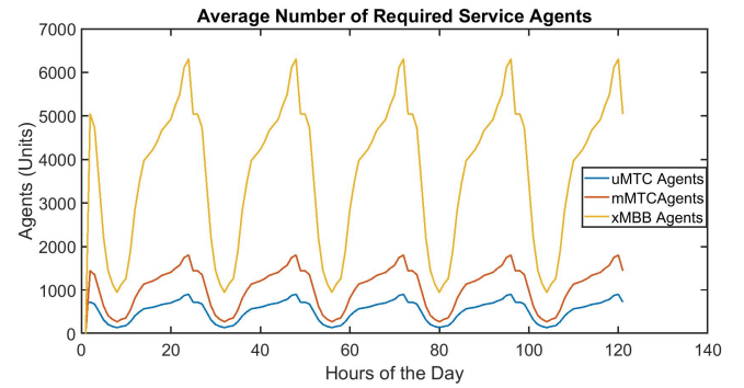
Fig. 16. Average Number of Required Service Agents
