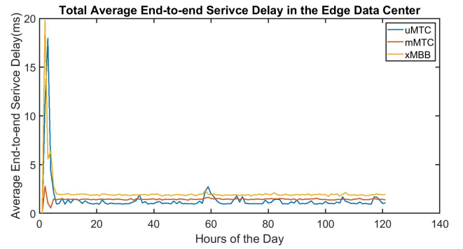
Fig. 25. End-to-End Service Latency in Edge Data Center
