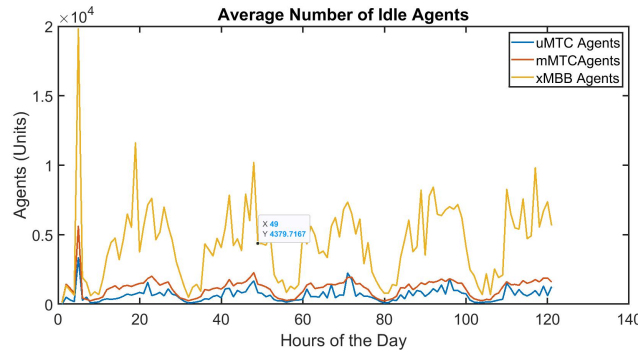
Fig. 17. Average Number of Idle Agents
