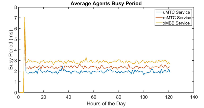
Fig. 21. Agent Busy Period
