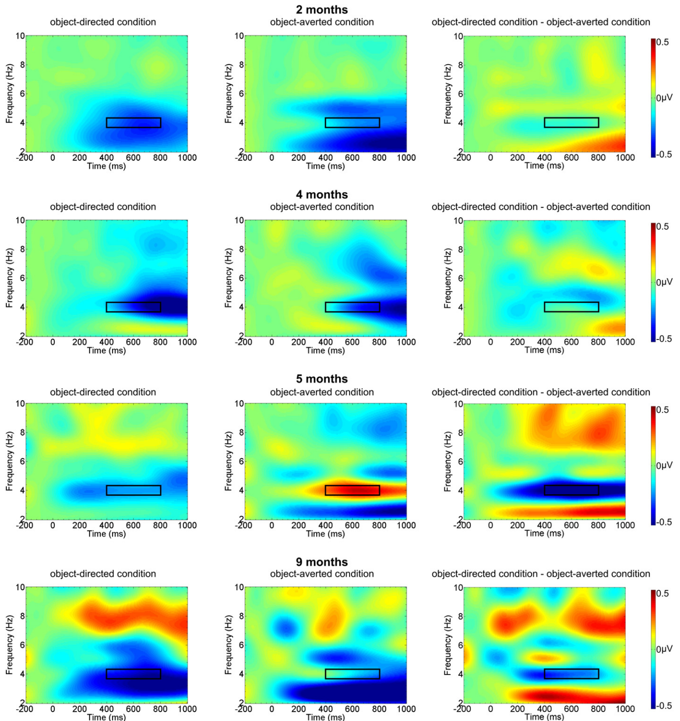
Fig. 2. Mean time–frequency spectrum averaged across 5 fronto-central channels showing theta activity in the object-directed condition, the object-averted condition, and the difference in theta activity between the object-directed–object-averted condition in 2-, 4-, 5-, and 9-month-olds. The rectangle marks the analyzed time window at 4 Hz.
