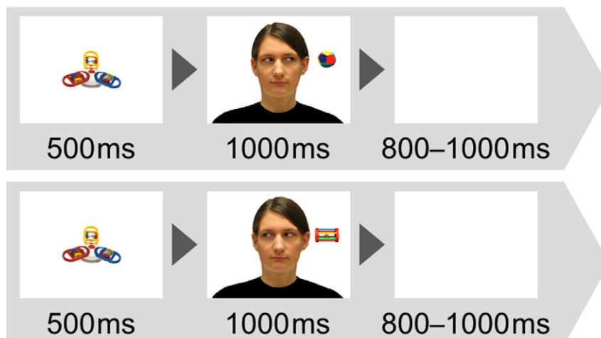
Fig. 1. Examples of a trial in the object-directed condition (top) and the object-averted condition (bottom).
