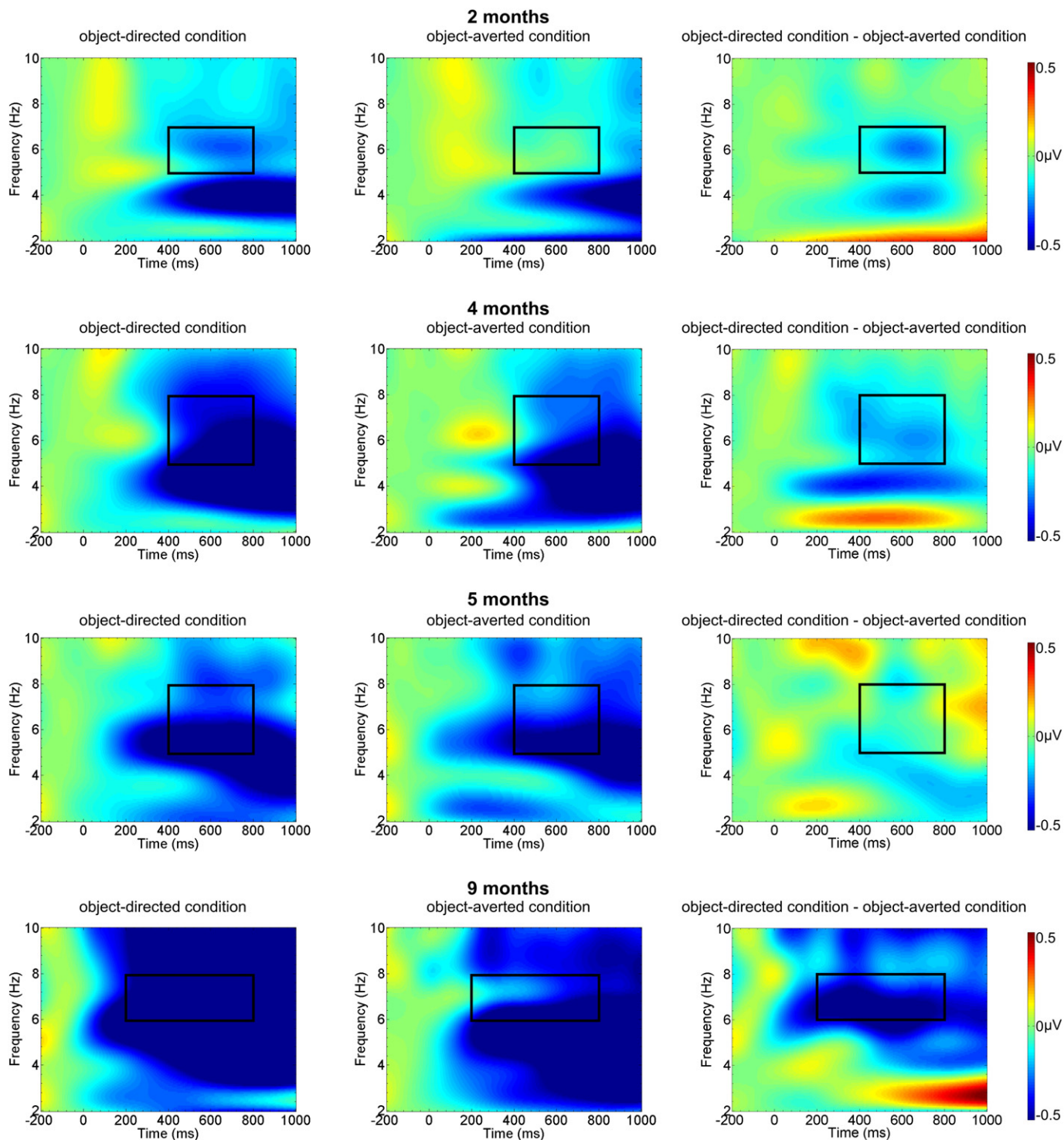
Fig. 3. Mean time–frequency spectrum averaged across 5 posterior-occipital channels showing alpha activity in the object-directed condition, the object-averted condition and the difference in alpha activity between the object-directed–object-averted condition in 2-, 4-, 5-, and 9-month-olds. The rectangle marks the analyzed time–frequency range.
