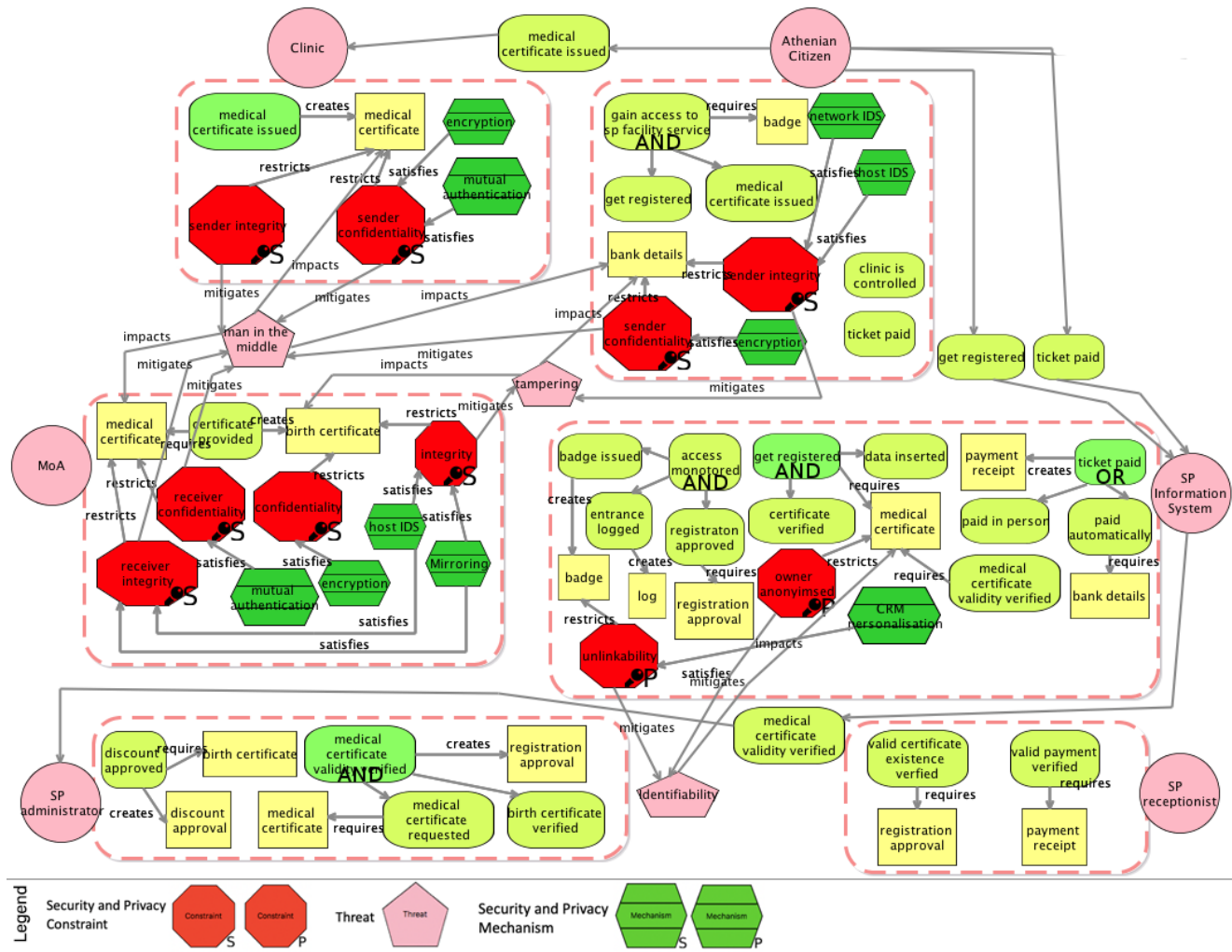
Fig. 6 Example of Security Requirements view
