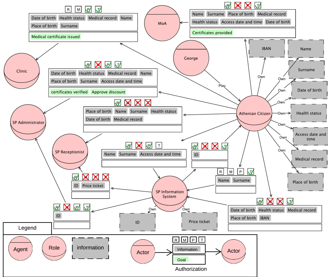
Fig. 4 Example of STS-ml authorisation view
