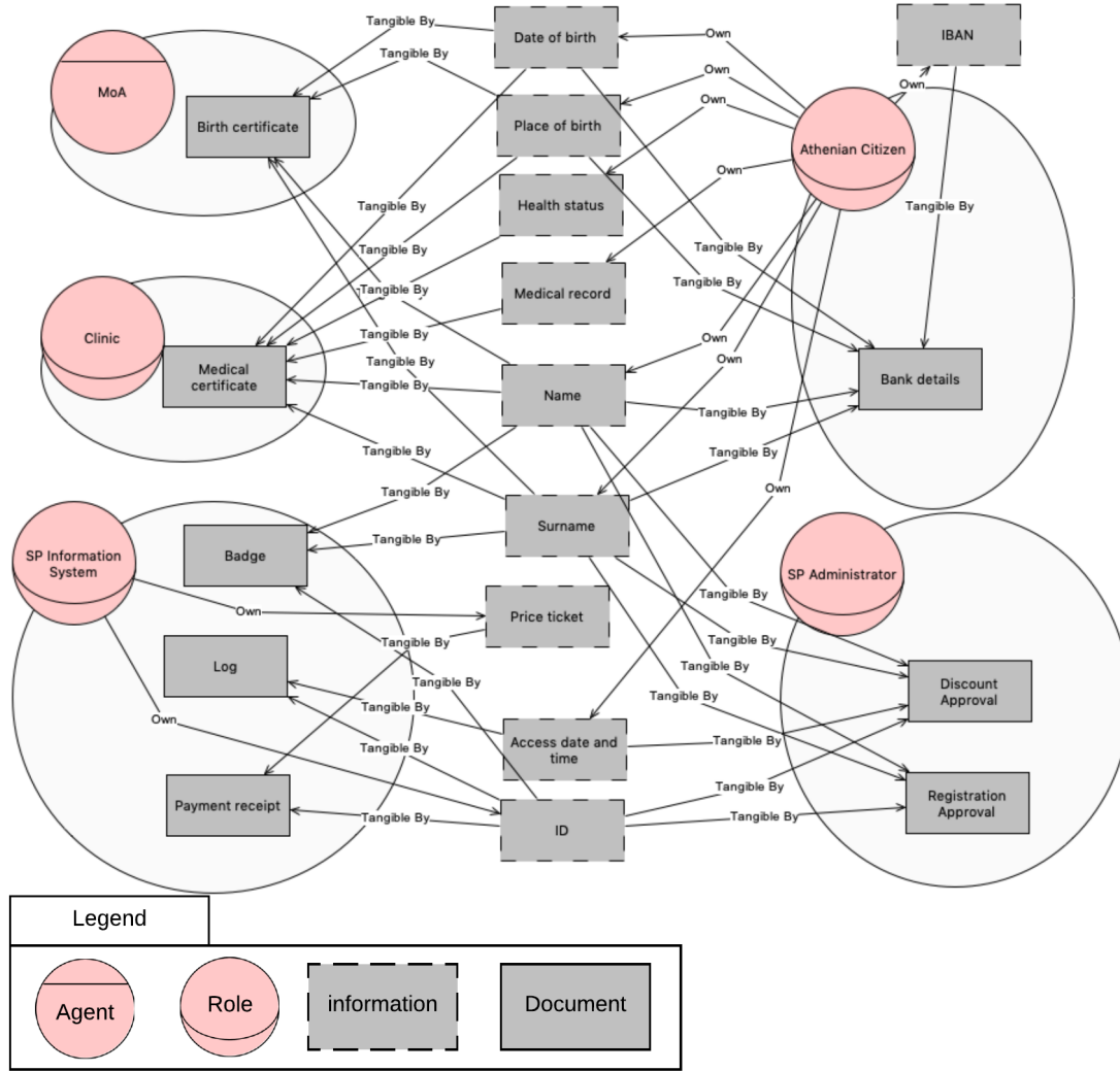
Fig. 3 Example of STS-ml information view
