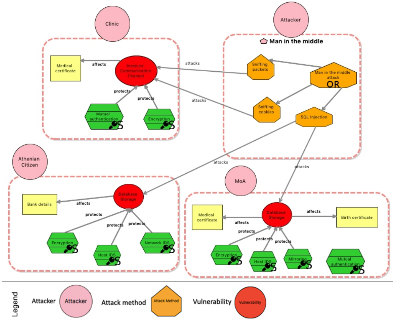
Fig. 7 Example of Attacks view
