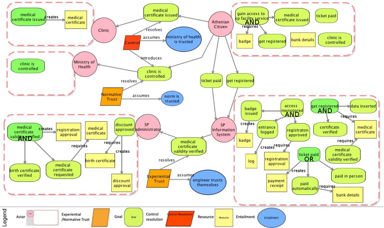
Fig. 5 Example of Trust view
