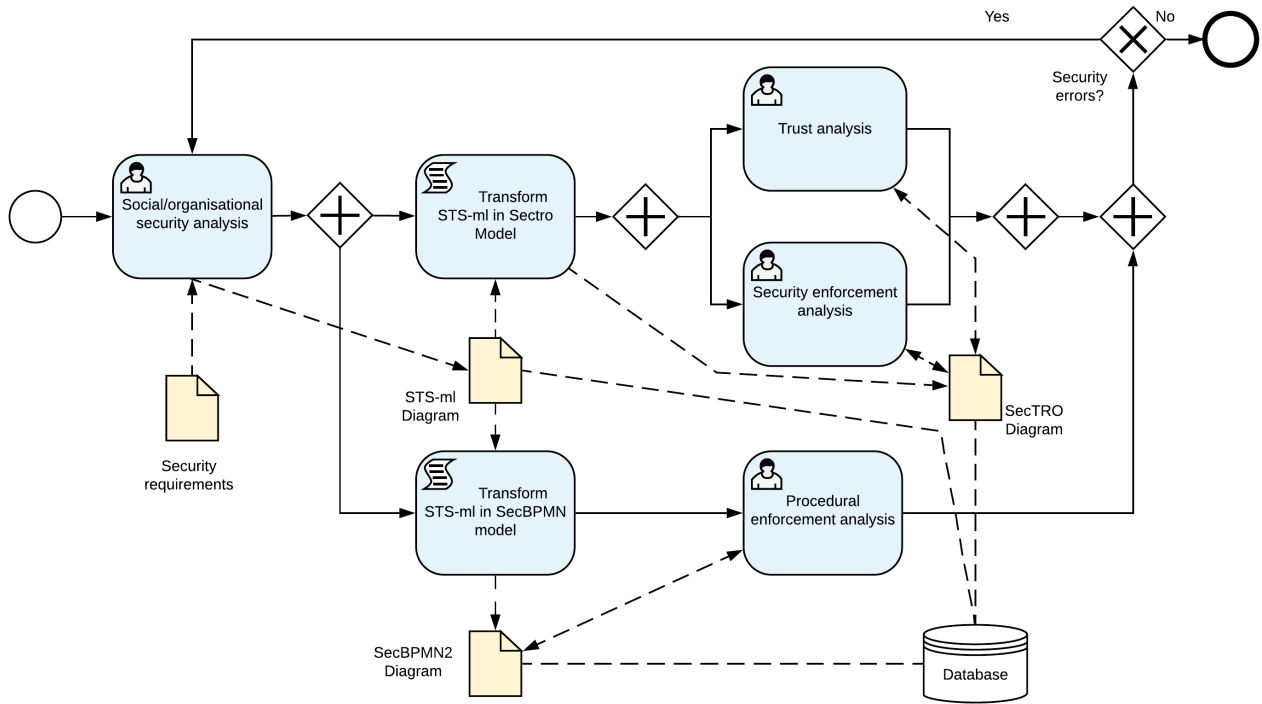
Fig. 1 Systematic approach proposed in this paper
