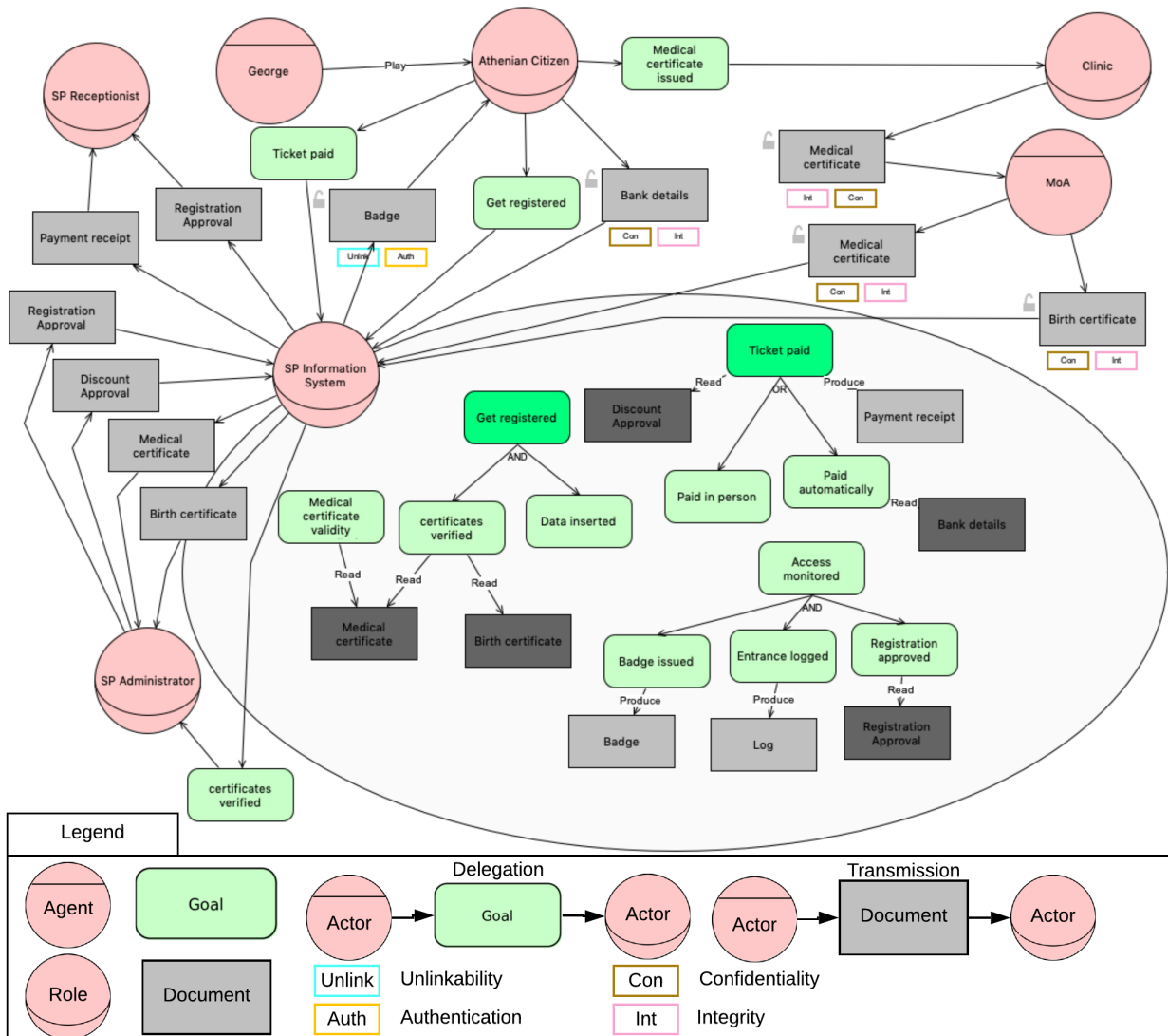
Fig. 2 Example of STS-ml social view
