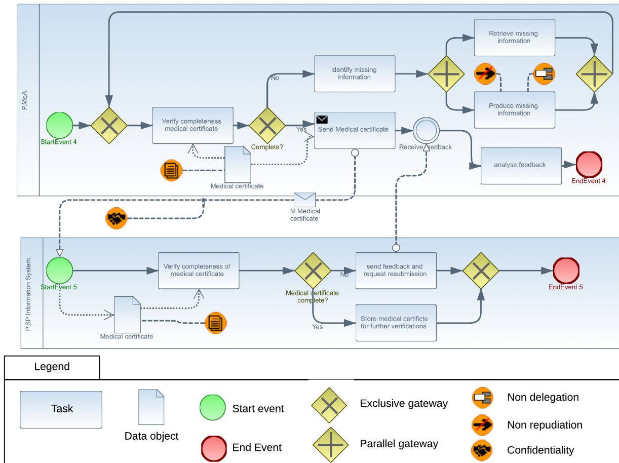
Fig. 8 Example of SecBPMN2
