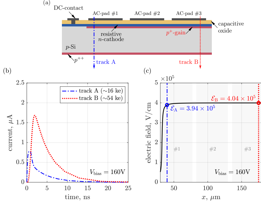
Figure 9: Panel (a): schematic cross section of the simulated RSD (not to scale), where two heavy ion MIP tracks have also been represented. Panel (b): current signals read at the DC-contact for the two tracks A and B (legend reports the corresponding number of collected charges). Panel (c): electric field along the resistive cathode; vertical lines represent the position of the tracks while labels indicate the field at that coordinates.
