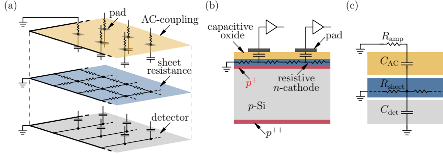
Figure 2: Basic operational principles of the resistive AC-coupled readout: (a) Electronic equivalent circuit. (b) Cross-sectional sketch of a silicon n -in- p RSD where the n -type cathode, freezing the charges, and a cap dielectric, to allow the signal transfer to the pads by capacitive induction, are represented. (c) Circuitual model in correspondence of a single node of the resistive sheet, i.e. for a readout pad.
