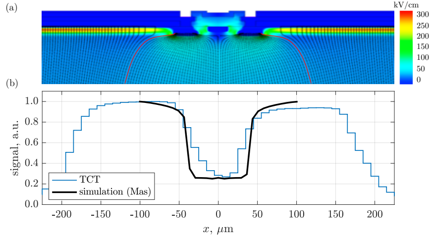
Figure 8: Panel (a): simulated electric field (intensity color map) and drift lines in the inter-pixel region of an LGAD device. Panel (b): comparison between measured (histogram) and simulated (curve) signal amplitude versus position for an IR laser scan carried out along a 200\mu\text{m} -pitch LGAD strip-detector. Note: pictures (a) and (b) are not to the same scale.
