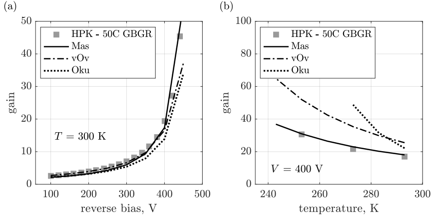
Figure 4: Comparison between measured (symbols) and simulated (lines) gain in unirradiated 50\mu\text{m} -thick LGAD sensors by HPK as a function of (a) applied bias and (b) temperature. Experimental data taken at HPK and presented in Refs. [7, 25].
