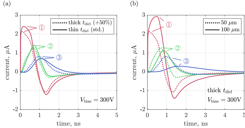
Figure 13: TCAD simulations of AC-coupled signals generated in a 50\mu\text{m} -pitch three-pad RSD sensor (the circled numbers identify the position of the pad, from left to right) by a MIP heavy ion for (a) two dielectric thicknesses and (b) pad pitches. The parametric setup is the standard one in the left plot while in the second one a thick dielectric has been implemented.
