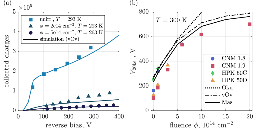
Figure 5: Measurements (symbols) and simulations (lines) of (a) charges versus bias in an irradiated 300- \mu\text{m} LGAD sensor by FBK and (b) bias to collect 20k electrons as a function of fluence in 50- \mu\text{m} -thick LGAD sensors by HPK and CNM. Experimental data presented in Refs. [7, 23, 26].
