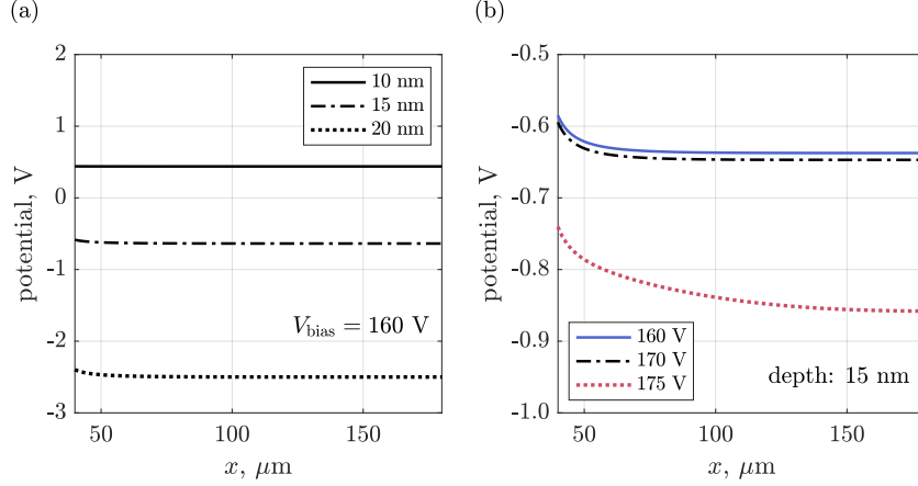
Figure 10: Horizontal trend of the electrostatic potential simulated in the RSD device represented in the cross section of Figure 9 as a function of (a) depth with respect to the Silicon/oxide interface, at fixed bias V_{\text{bias}} = 160 V, and (b) at different applied bias, at a fixed depth of 15 nm.
