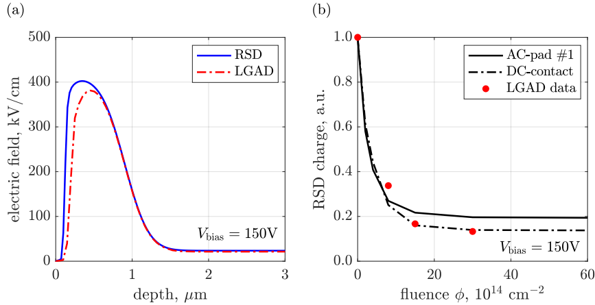
Figure 15: Panel (a): electric field profile along a vertical cut of (unirradiated) RSD and LGAD devices having the same p -gain implant, simulated at 150 V. Panel (b): simulated (normalized) charge degrading with fluence in an RSD device for both AC and DC signals (lines), along with a data set (dots) taken at the same bias voltage on an LGAD device from the UFSD2 run.
