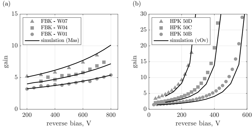
Figure 7: Room temperature comparison between measured (symbols) and simulated (lines) G(V) characteristics in (a) 300μm-thick LGAD detectors from UFSD1 production run by INFN and FBK (with the wafer number W increasing with the gain implant dose) and (b) 50μm-thick LGAD devices by HPK (where, again, the last letter increases with the increasing boron dose).
