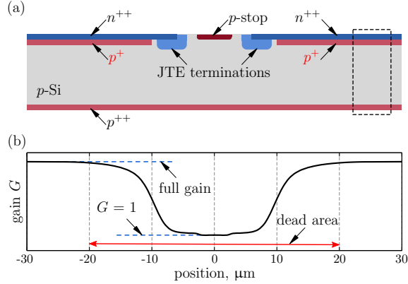
Figure 1: (a) Cross section of the segmentation structures between two adjacent LGAD active areas and (b) gain G as a function of the particle hit position calculated through numerical simulations. In the dashed rectangle: simple-2D slice including only the essential LGAD implants to be used in simplified simulations
