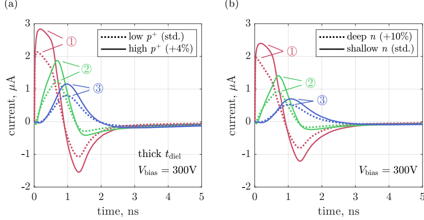
Figure 12: TCAD simulations of AC-coupled signals generated in a 50\mu\text{m} -pitch three-pad RSD sensor (the circled numbers identify the position of the pad, from left to right) by a MIP heavy ion for (a) two p -gain doses and (b) n -cathode depths. The parametric setup is the standard one in the right plot while in the first one a thick dielectric has been implemented.
