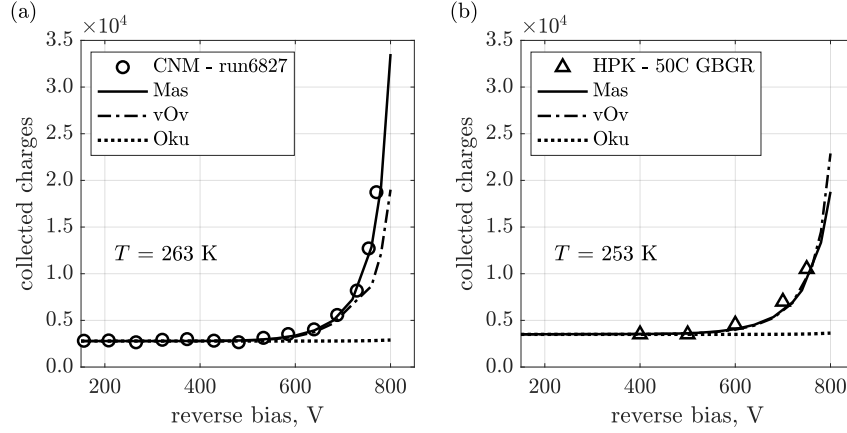
Figure 3: Measured (symbols) and simulated (lines) collected charge (or gain) for 1 MIP in 50\mu\text{m} -thick devices: (a) p - i - n diode irradiated with neutrons at \phi = 3 \cdot 10^{15} \text{ n}_{\text{eq}}/\text{cm}^2 and (b) pions at \phi = 1.5 \cdot 10^{15} \text{ n}_{\text{eq}}/\text{cm}^2 , respectively. Experimental data presented in Refs. [7, 22, 23].
