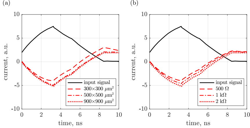
Figure 11: RSD response (red curves) of a TCAD-like input signal (solid black) simulated with Spice as a function of (a) the AC-pad size and (b) sheet resistance. The signal is injected and read on the same node of the resistive grid, as represented in the electrical model of Figure 2(a).
