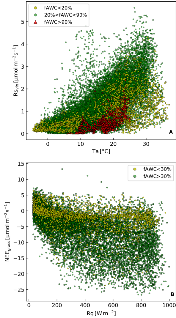
Fig. 4. a) Scatter plot of half hourly air temperature ( T_a ) and vineyard soil respiration ( R_{s_{vin}} ). Colors represent different fractions of soil available water content ( fAWC ): yellow dots fAWC below 20%, green dots fAWC between 20 and 90%, and red triangles fAWC above 90%. b) Scatter plot of half hourly global radiation ( R_g ) and grass net \text{CO}_2 flux ( NEE_{grass} ) at fAWC below (yellow dots) and above 30% (green dots). (For interpretation of the references to color in this figure legend, the reader is referred to the web version of this article.)
