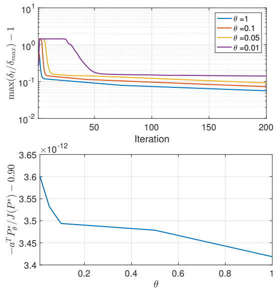
Fig. 3. The EMR overflow (up) and steady-state total transmitted power to the receivers (bottom) using the proposed distributed solution with different \theta and corresponding maximum \rho values according to Proposition V.1.
