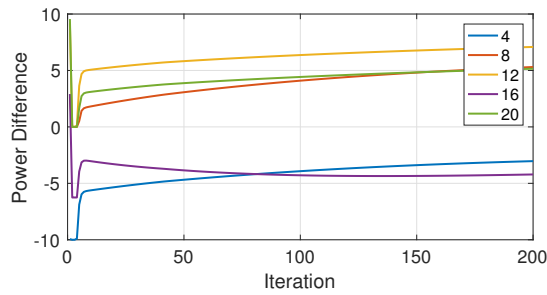
Fig. 4. The difference of the transmitter power levels in our algorithm and their optimal values, with \theta = 0.1 and the corresponding maximum \rho .
