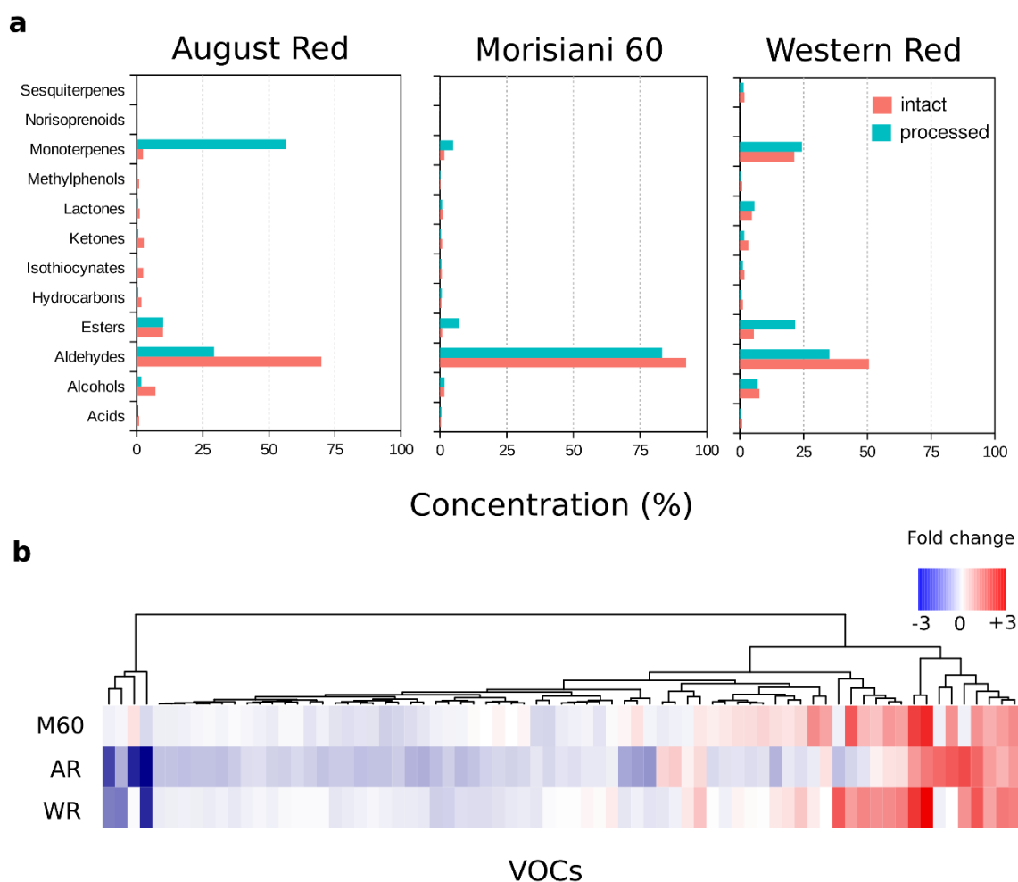
Figure 1. Analysis of unprocessed and processed nectarine VOC profile assessed by SPME/GC-MS.
