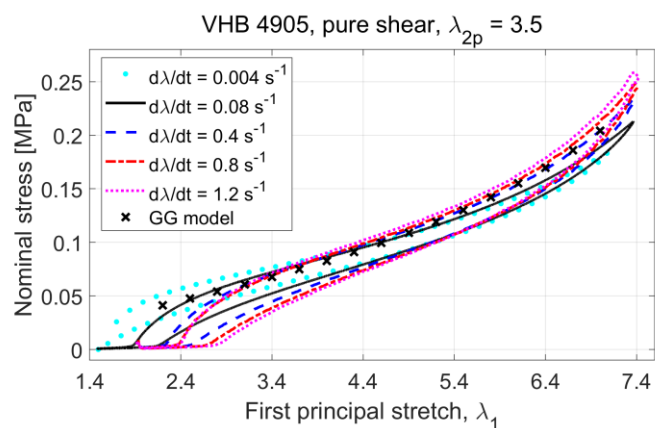
Figure 18. Cyclic stress-strain response of a pure-shear specimen with transversal pre-stretch \lambda_{2p} = 3.5 made of VHB 4905 for large stroke: experimental data at different strain rates vs. Gent-Gent (GG) model fitting
