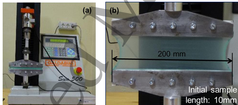
46 47 48 49 50 Figure 4: Set-up for membrane stress-strain response measurement
