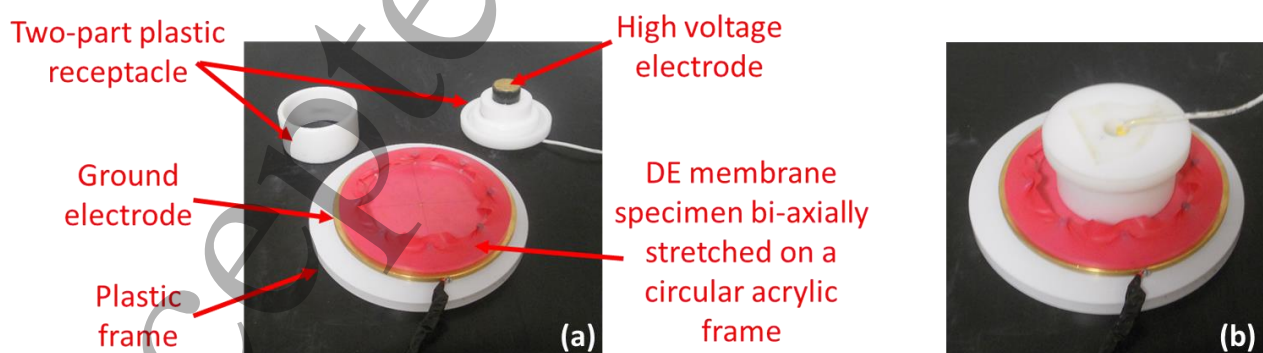
Figure 2: Electrode set-up for membrane dielectric strength measurement [30]: a) exploded view; b) assembled view
