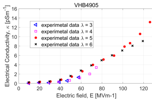
Figure 12: Electrical conductivity vs. electric field for VHB 4905: results comparison for specimens tested at different levels of equi-biaxial stretch ( \lambda )
