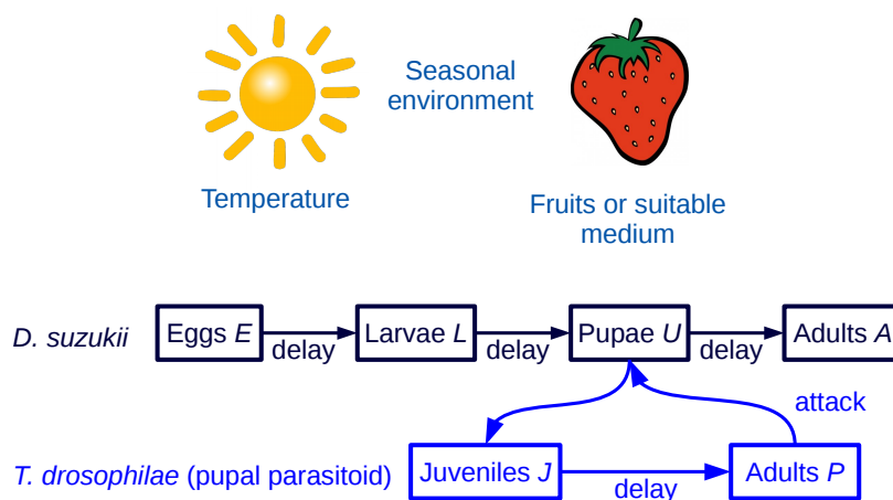
Fig. 1: Flow chart for the stage structured model
