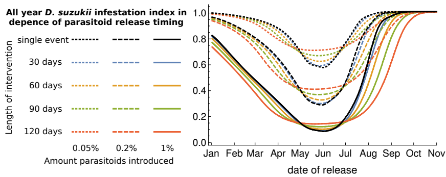
Fig. 10: Effect of time of parasitoid introduction and amount of parasitoids introduced on all year D. suzukii infestation index (which is proportional to the total amount of D. suzukii eggs laid over the year). The dotted, dashed and straight lines correspond to an overall introduction of 0.05%, 0.2% and 1% of parasitoids compared to the yearly maximum of D. suzukii adults reached without parasitoid intervention. The black lines correspond to a scenario where all parasitoids are released at a single event at the date given on the x-axis. The other lines correspond to an equally distributed parasitoid release around the date on the x-axis for 30, 60, 90 and 120 days. The underlying temperature curve is the generic sinusoidal fit used before
