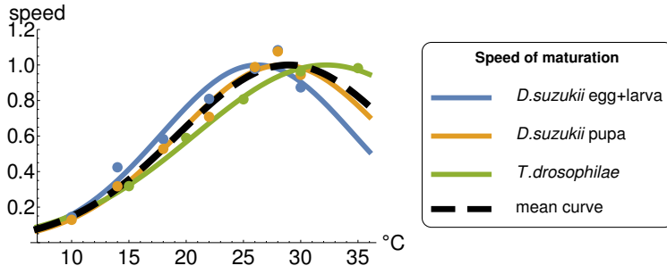
Fig. 3: Maturation speed of different life stages of D. sukukii and its pupal parasitoid T. drosophilae
