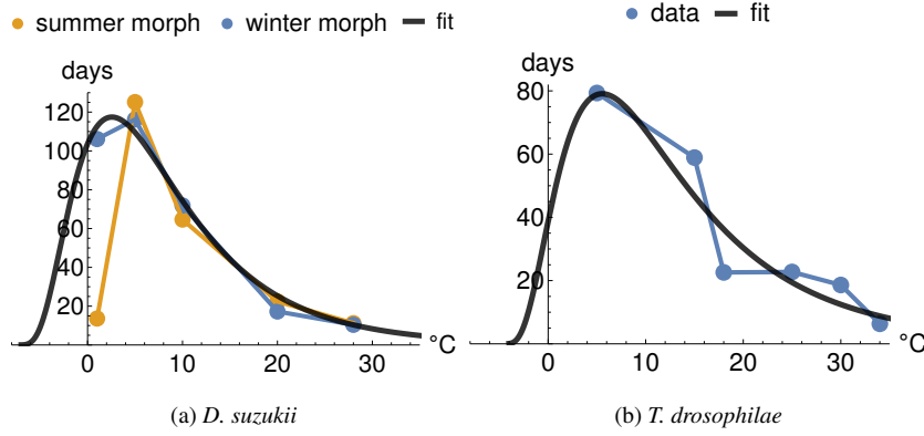
Fig. 5: Average adult life length of D. suzukii and T. drosophilae
