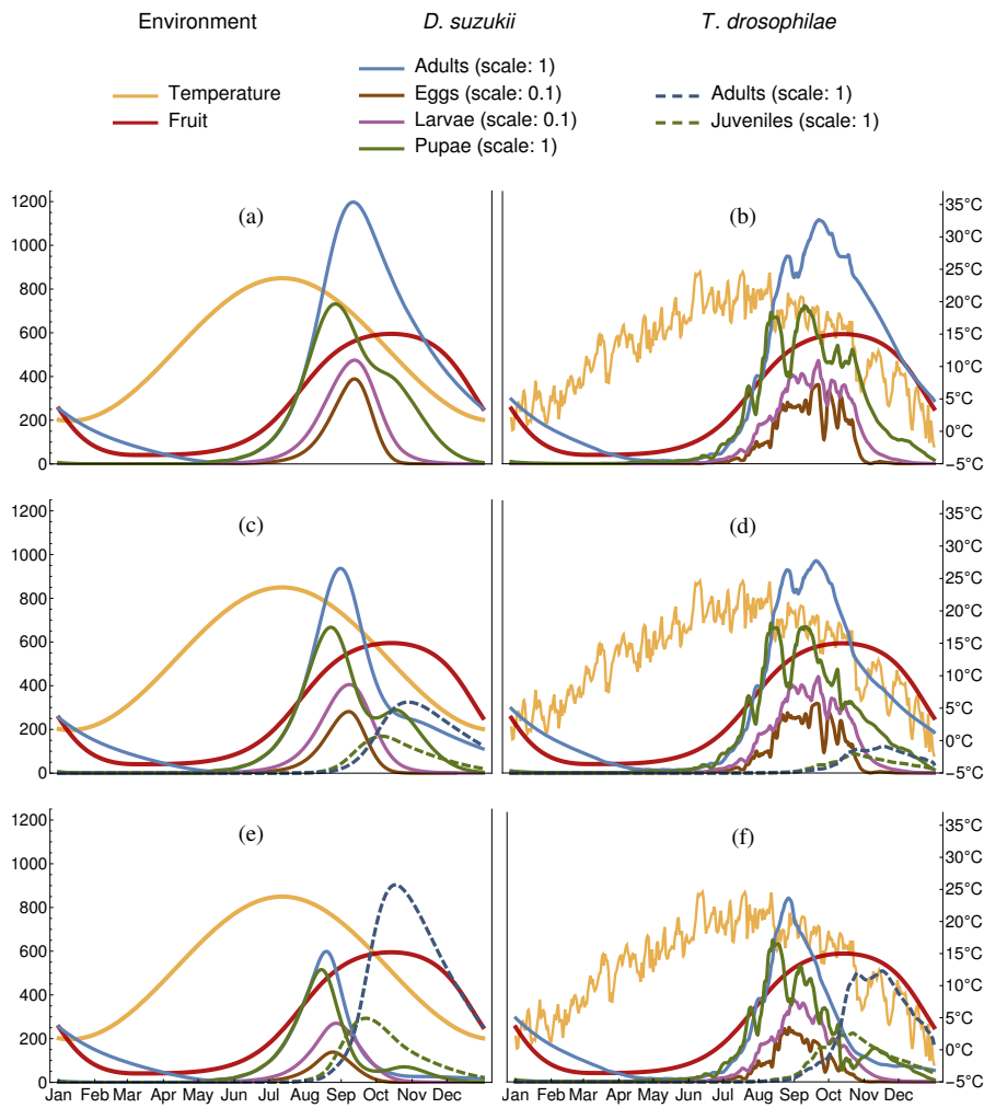
Fig. 8: Simulated D. suzukii population size without (a, b) and with parasitoids introduced on 1 April (c, d) and 1 June (e, f). Figures a, c, and e (left) were created using the sinusoidal temperature curve and b, d, and f (right) interpolating the daily mean temperatures. Curves were created using weather data originally collected during 2014 in S. Michele all'Adige at 228m a.s.l., Province of Trento, Italy. The number of parasitoids released corresponds to 0.1% of the maximal D. suzukii adult population size reached in the simulations without intervention
