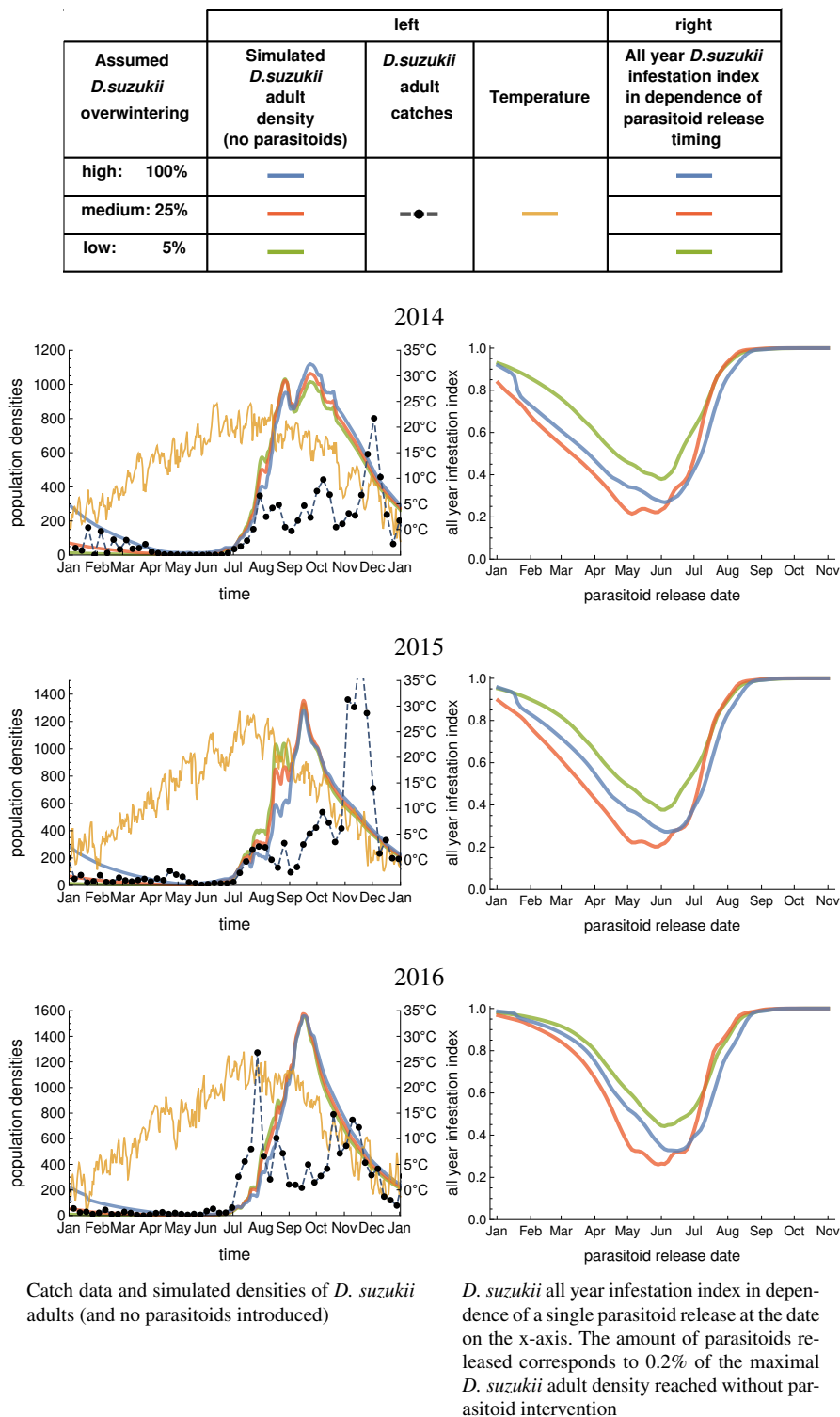
Fig. 11: Simulations with daily mean temperature data of the years 2014-2016. Left: simulated D. suzukii adult densities and catch data. Right: success of a parasitoid intervention in dependence of its timing. Three scenarios for the winter survival are simulated: high, medium and low survival corresponds to starting the year with 100%, 25% and 5% of the D. suzukii adults at the end of the previous year (without parasitoid intervention). For each survival scenario, the D. suzukii attack rate \alpha_A is adjusted so that the simulations fit roughly the onset of the catch data
