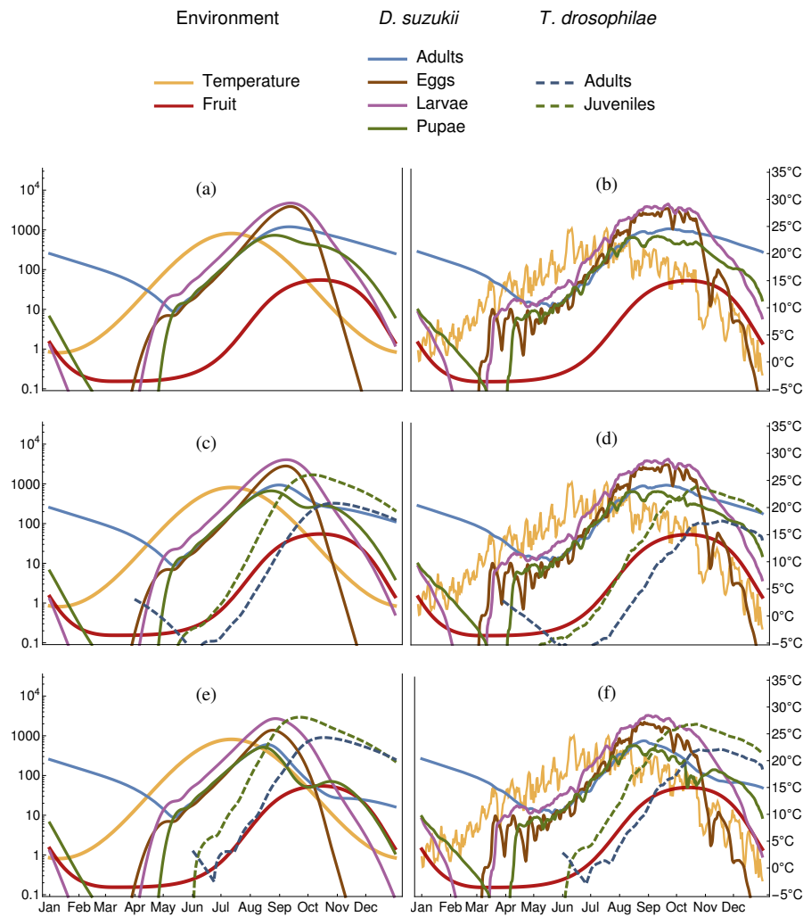
Fig. 9: Simulations of different parasitoid release scenarios. The plots are the same as in Fig. 8, but the population densities are shown in logarithmic scale
