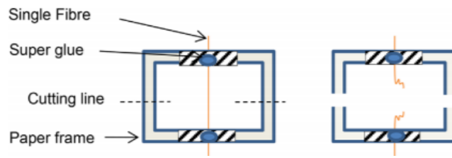
Figure 1. Schematic illustration of single fiber sample preparation for mechanical tests.
