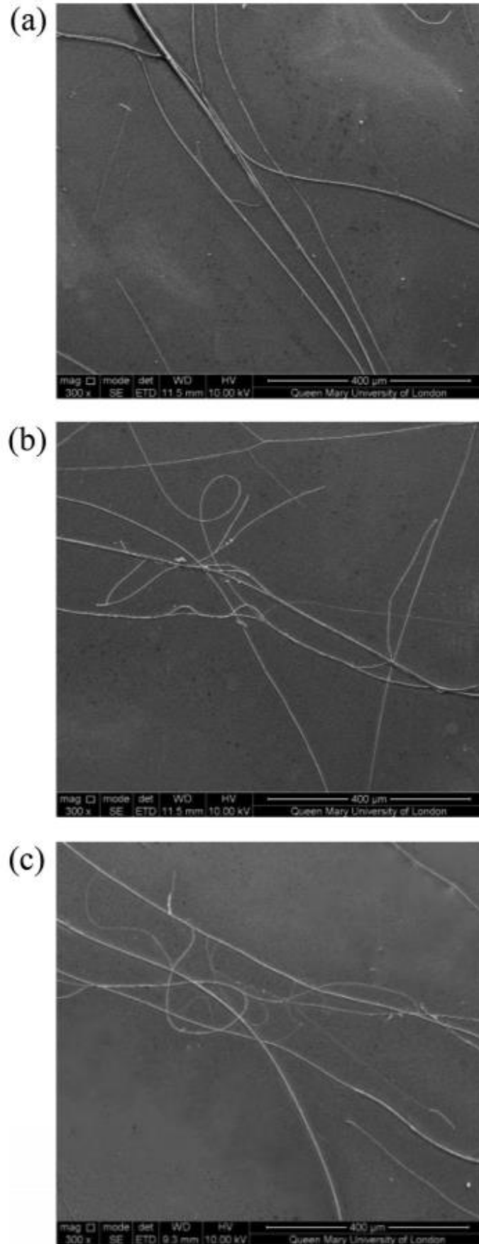
Figure 4. SEM micrographs of fibers electrospun from PPTA solutions with concentrations of (a) 15 wt% (b) 17 wt%, and (c) 19.46 wt% PPTA in H 2 SO 4 .
