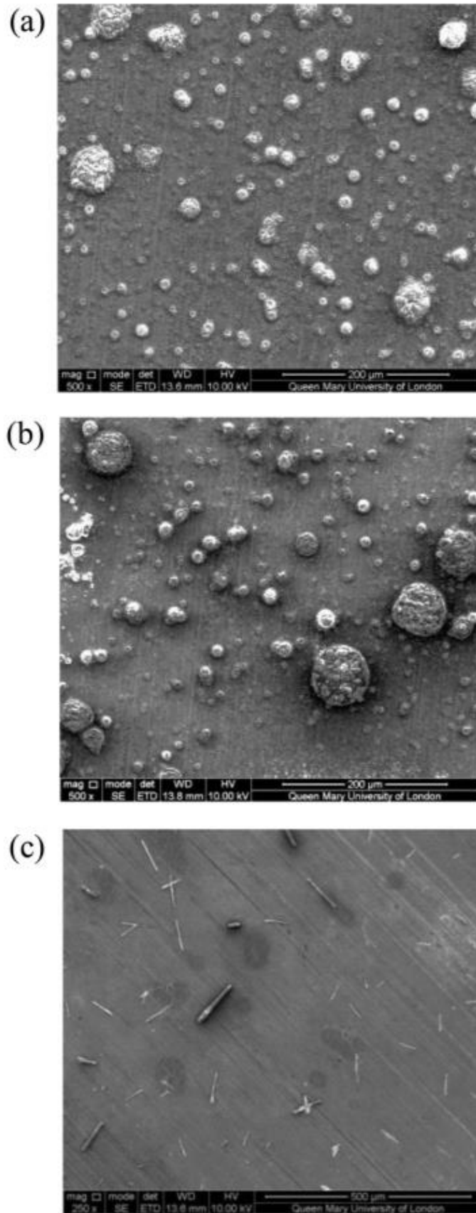
Figure 3. SEM micrographs of electrospun (or rather electrospayed) PPTA solutions with concentrations of (a) 3 wt% (b) 5 wt%, and (c) 7 wt% PPTA in H 2 SO 4 .
